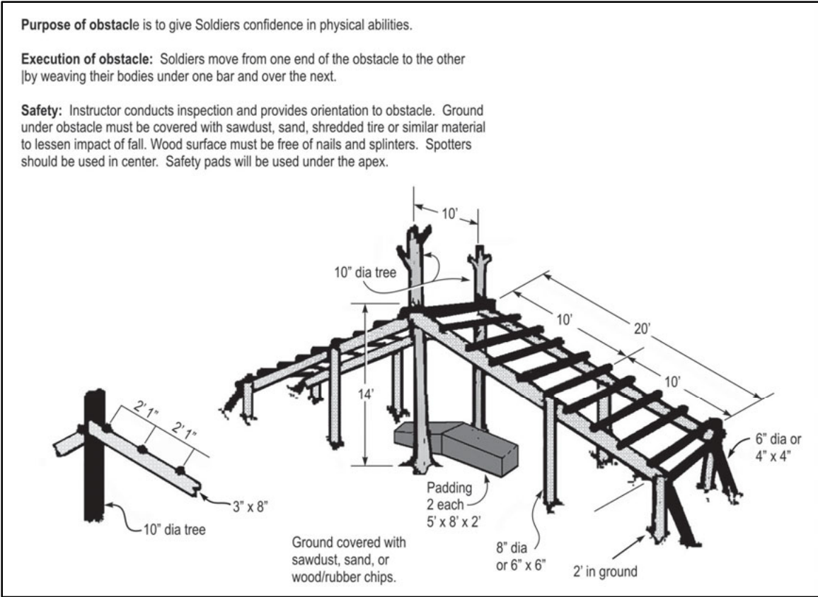
Figure E-32. Weaver (course sketch)
