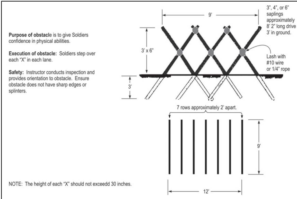
Figure E-21. Tough nut (course sketch)
