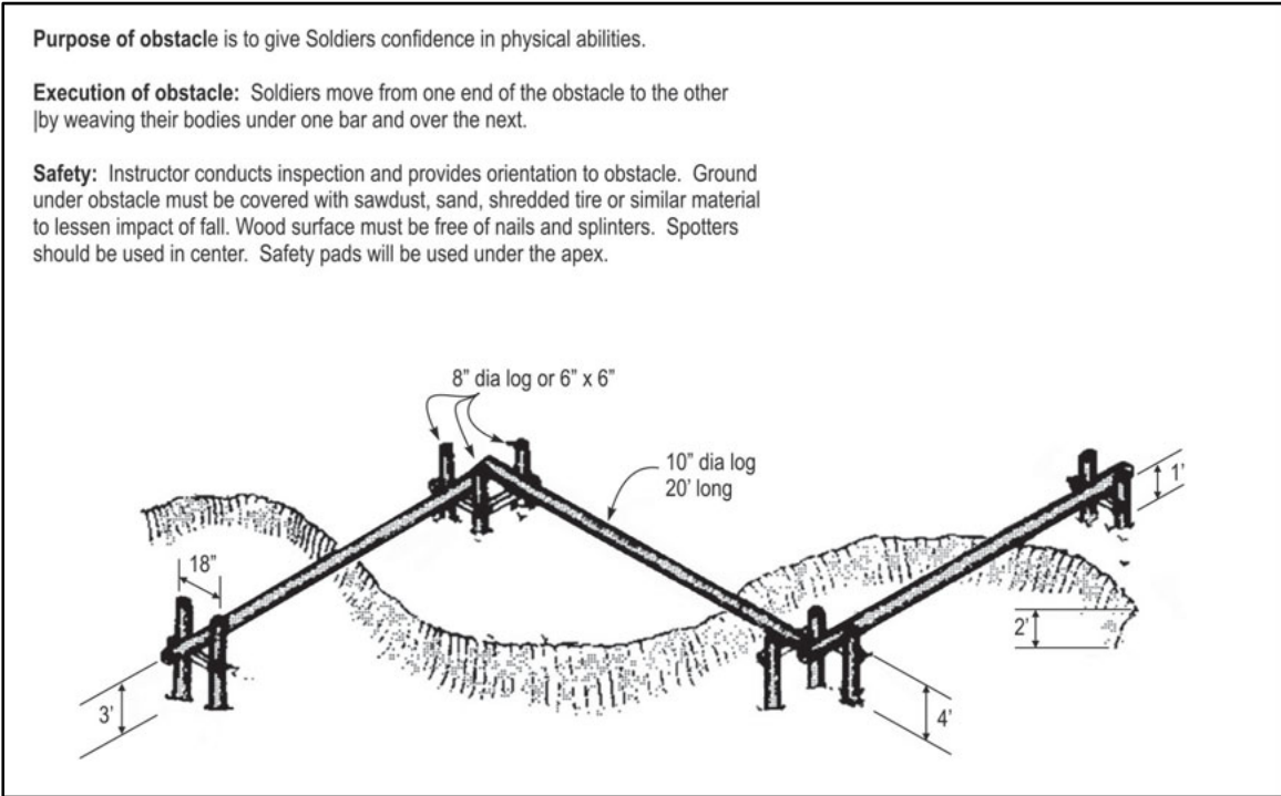
Figure E-33. Balancing logs (course sketch)
