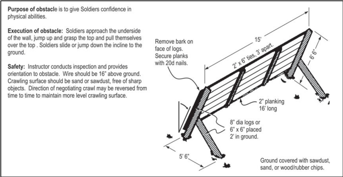
Figure E-23. Inclining wall (course sketch)
