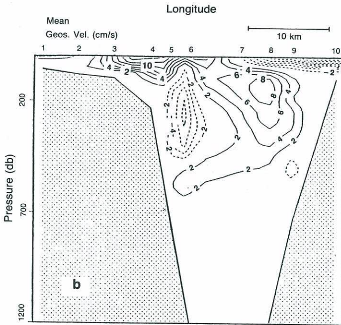
Figure 11 Sequence of ten hydrographic stations acquired across MB between 8 and 11 May 1988, at the locations indicated (a). To obtain the geostrophic velocities shown in the lower panel (b), the temperature and salinity data acquired at each location were averaged to reduce the effects of aliasing by the internal tide. The level of no motion (assumed) was chosen to correspond to the deepest common depth between stations. Solid contours depict flow into the Bay and dashed contours, flow out of the Bay. (Adapted from Koehler 1990).
