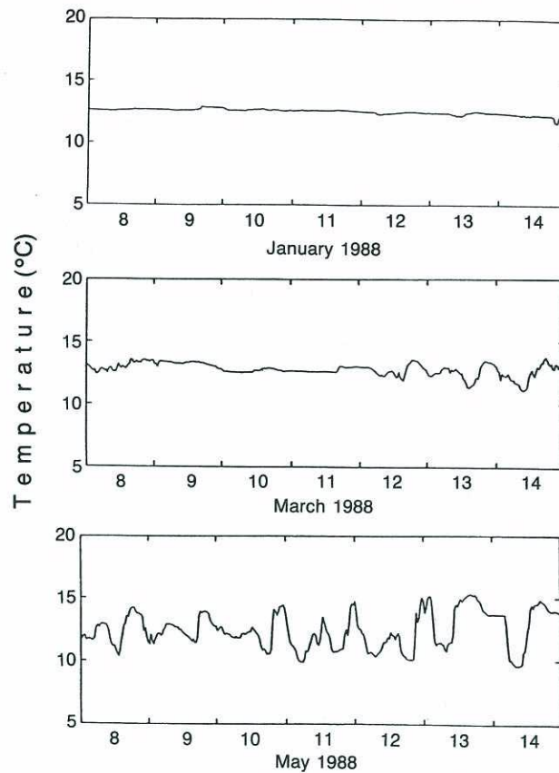
Figure 20 Temperature at 12m in southern Monterey Bay near Monterey Bay Aquarium (MBA-Fig. 1) during one week periods in January, March and May 1988. Effects of the internal tide at this depth increase with development of seasonal stratification.
