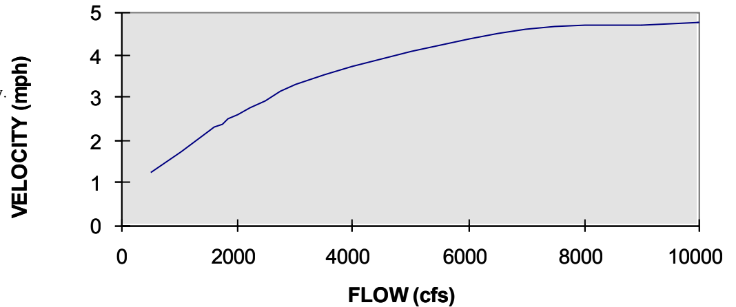
Velocity vs Flow
