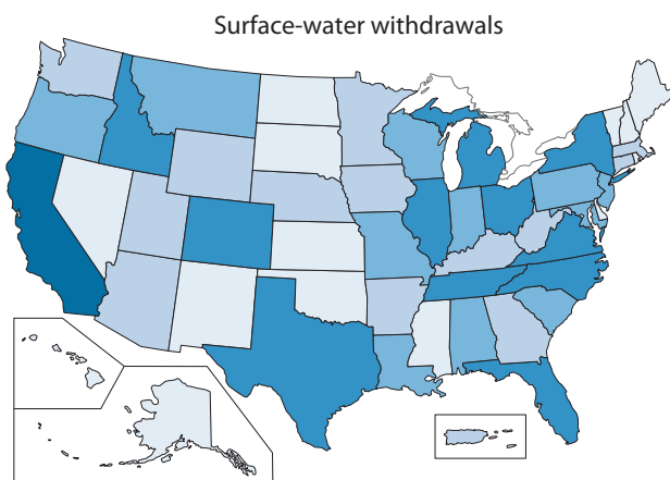
Total, surface-water, and groundwater withdrawals, 2005.
