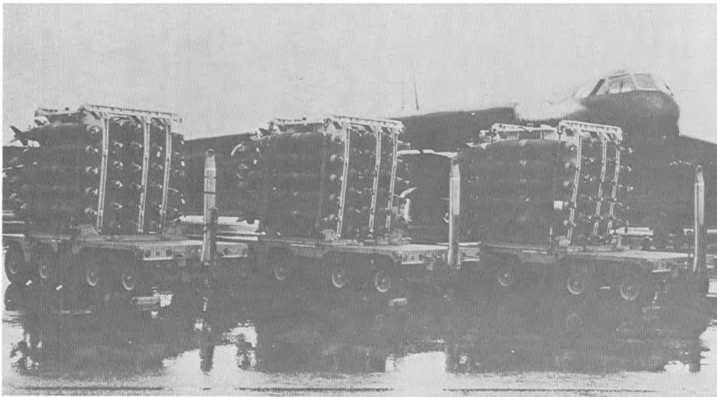
Preloaded bombs on "clip-in" racks. Bombs can be loaded one at a time, or preloaded and inserted as a clip-in package, if special preload equipment is available. There was no preload equipment at Andersen; all bombs had to be loaded in the bomb bay racks one at a time. Shown is a full internal load of 84 500-pounders.
