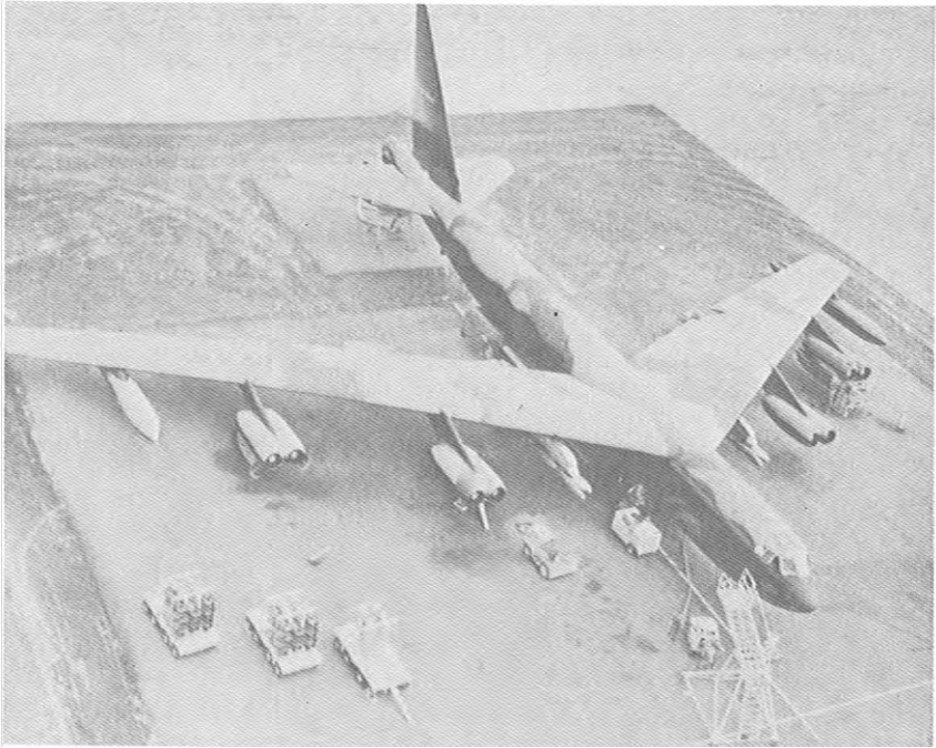
During preparatory maintenance, each parking hardstand, such as this one at U-Tapao, was crowded with special equipment and weapons. The clip-in assemblies shown are loaded with 750-pounders.
