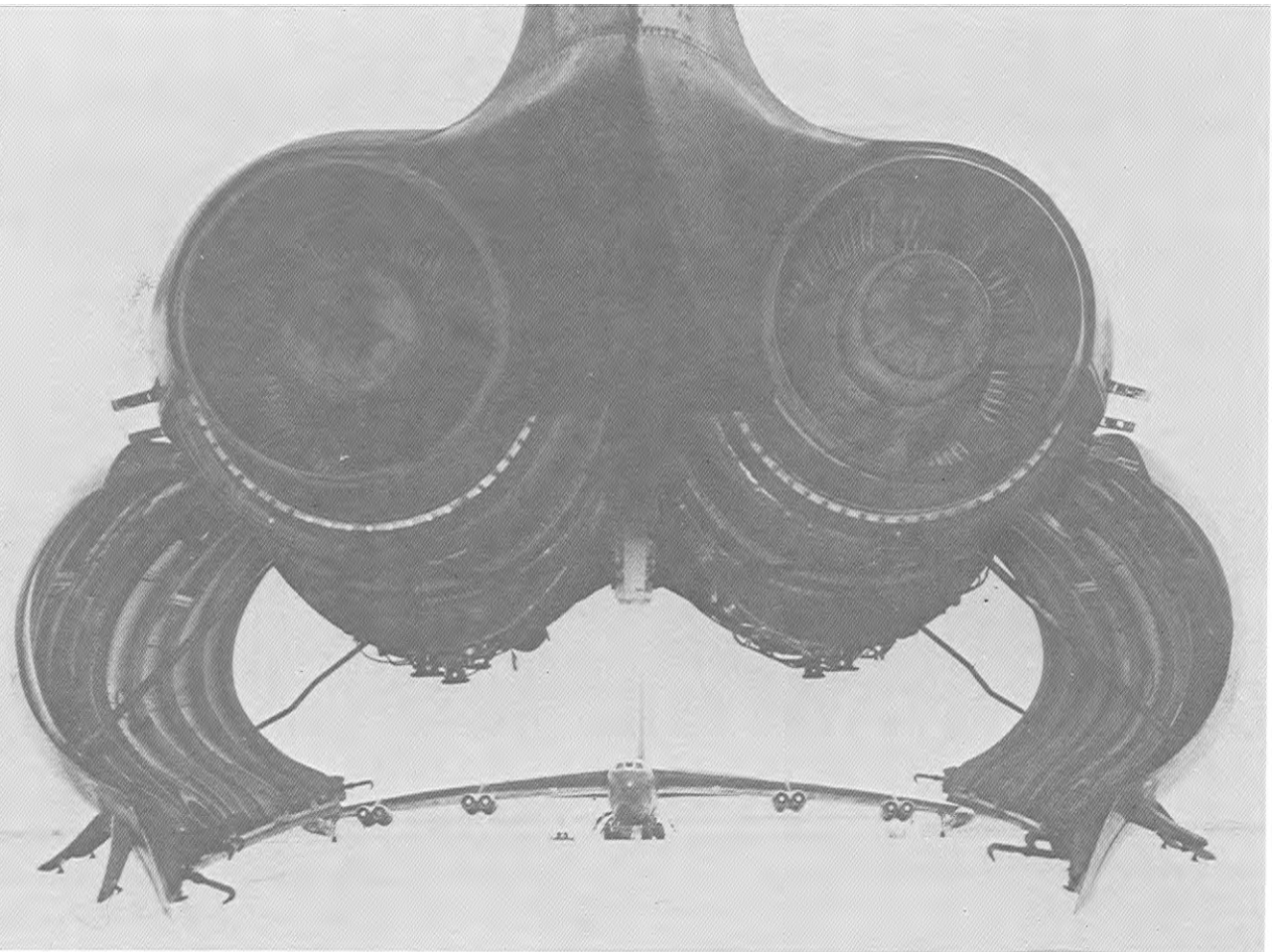
Two of the eight jet engines on a B-52 have their cowlings spread to permit maintenance specialists access to engine components.
