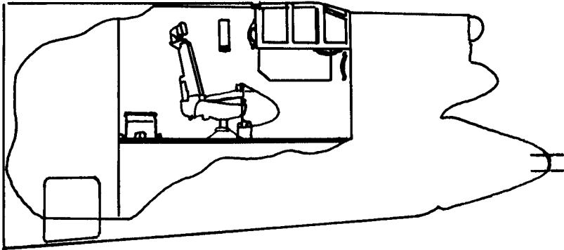
The B-52D tail gunner's compartment. Unlike the G model, five men occupy the forward crew compartment, with the sixth in the extreme tail end. This position has a gun turret which may be jettisoned, followed by manual bailout.
