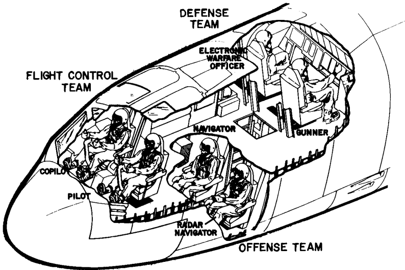
B-52G crew positions. The six-man crew is positioned in the forward 15 percent of the aircraft. All are equipped with ejection-seats. The total area available for crew movement may be visualized by this sketch.
