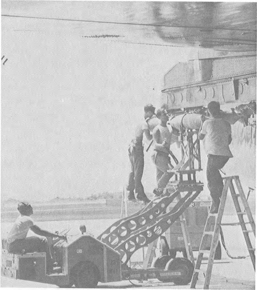
Loading one of 12 bombs which mounted on the external racks under each wing of the "D" model." It took teamwork, muscle power, and special equipment to position and attach each bomb.
