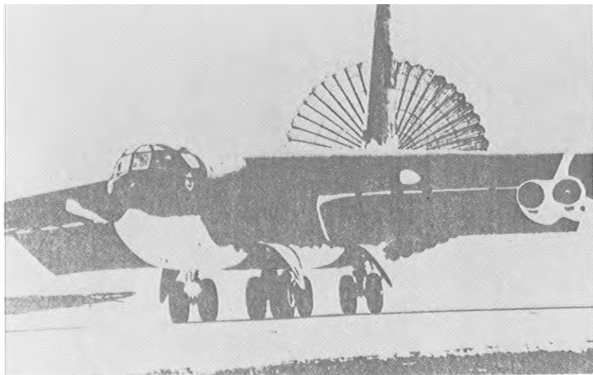
Looking deceptively short through the telephoto lens, a B-52G deploys its drag chute during the landing roll.
