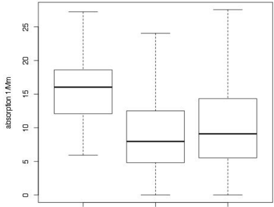
Red, Green and Blue Channels, 1um, PSAP
