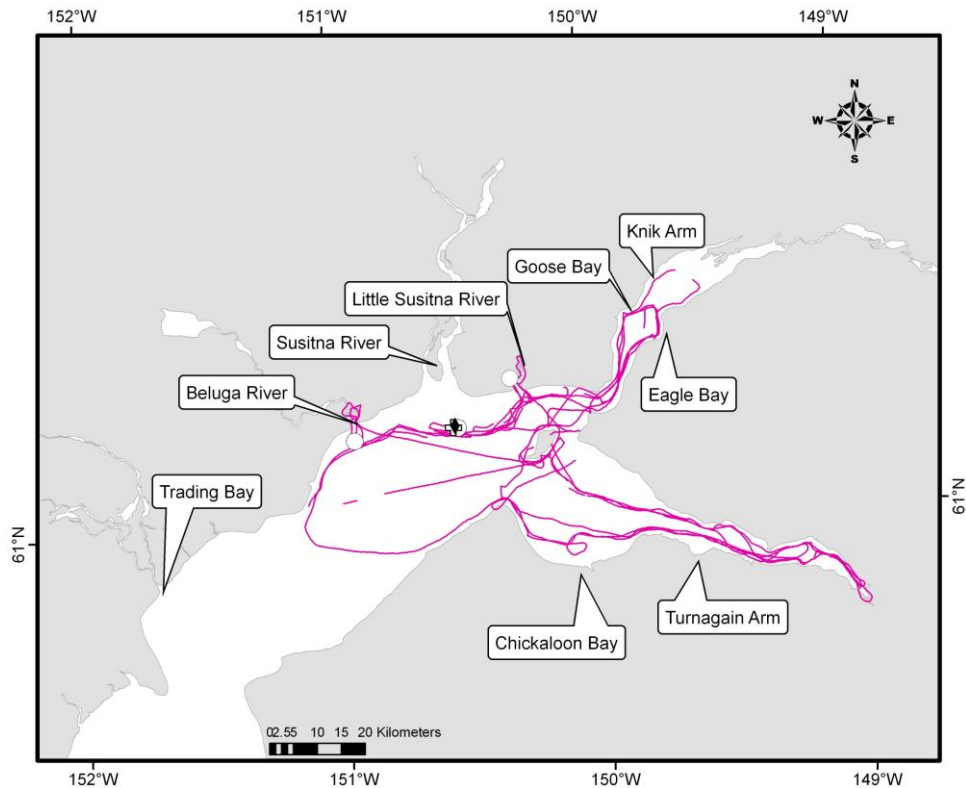
Figure 4. All on-effort tracklines flown during the August 2011 survey (red lines) with daily harbor seal sightings (white crosses = 9 Aug., white circles = 10 Aug., and black diamonds = 11 Aug).
