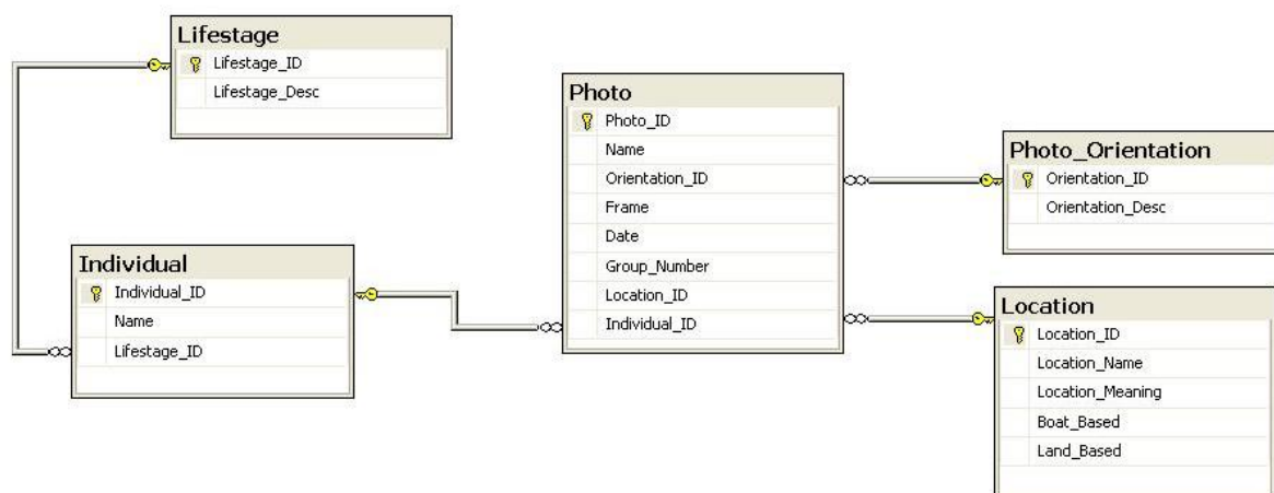
Figure C1. Database Diagram for Photo ID Catalog
