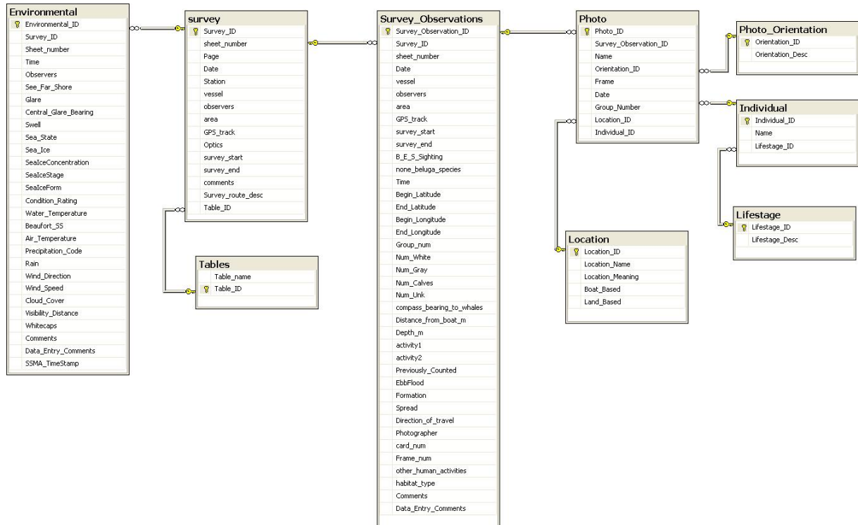
Figure C2. Complete Database Diagram for Photo_ID Catalog study
