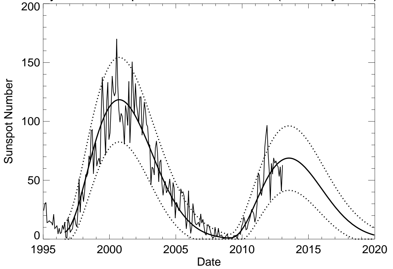
Cycle 24 Sunspot Number Prediction (February 2013)
