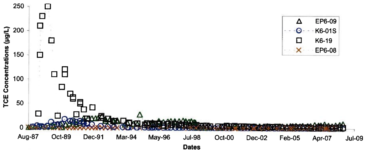
Figure 5. Historical TCE concentrations at Pit 6 monitoring wells EP6-08, EP6-09, K6-01S, and K6-19
