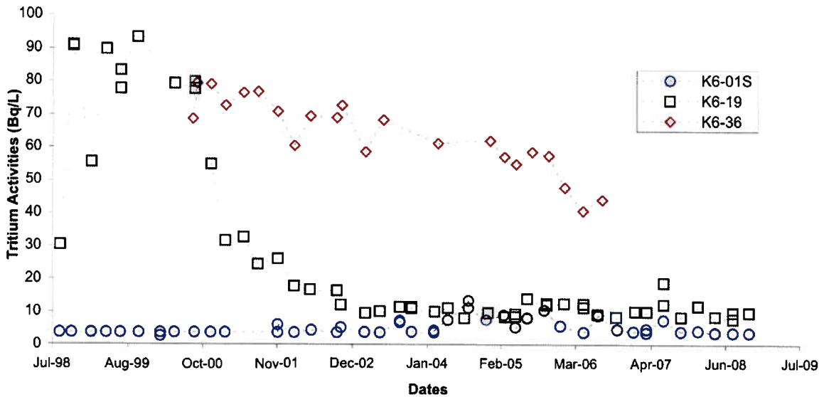
Figure 4. Historical tritium activities at Pit 6 for wells K6-01S, K6-19, and K6-36
