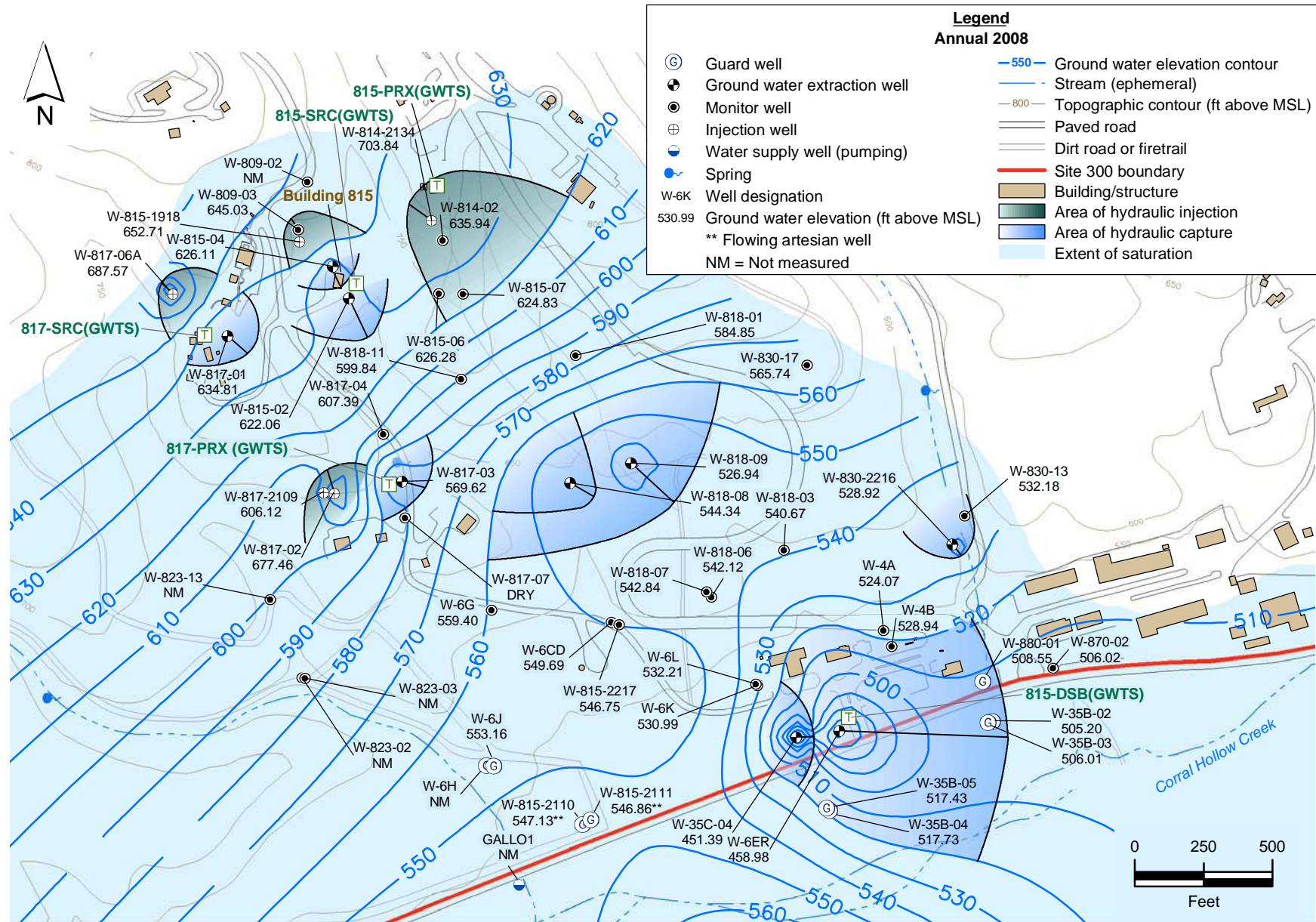
Figure 2.4-7. High Explosives Process Area OU ground water potentiometric surface map for the Tnbs 2 HSU.
