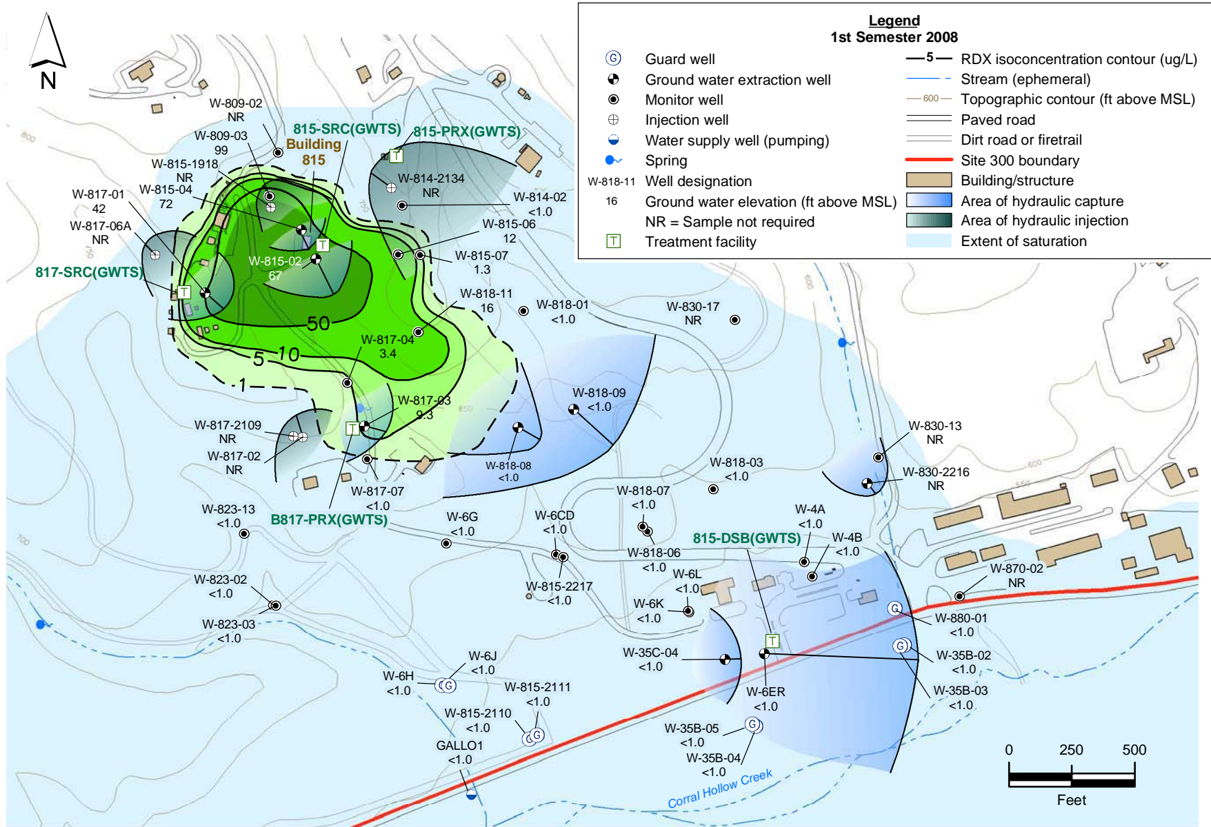
Figure 2.4-9. High Explosives Process Area RDX isoconcentration contour map for the Tnbs 2 HSU.
