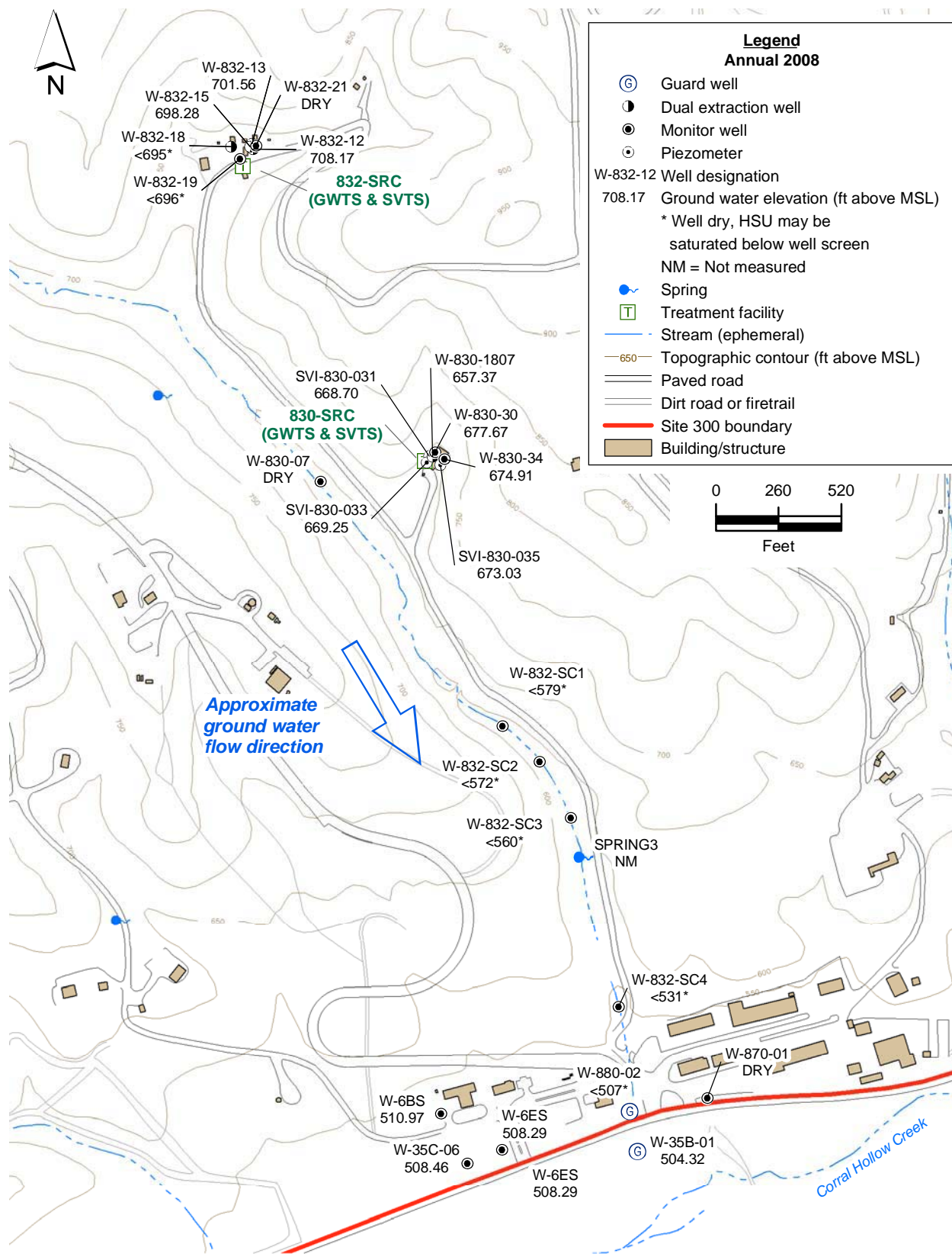
Figure 2.7-2. Building 832 Canyon OU map showing ground water elevations and ground water flow direction for the Qal/WBR HSU.
