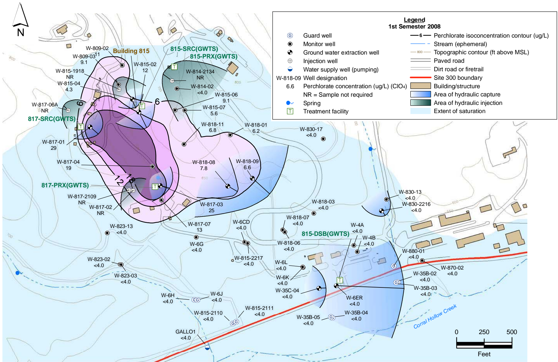
Figure 2.4-10. High Explosives Process Area perchlorate isoconcentration contour map for the Tnbs 2 HSU.
