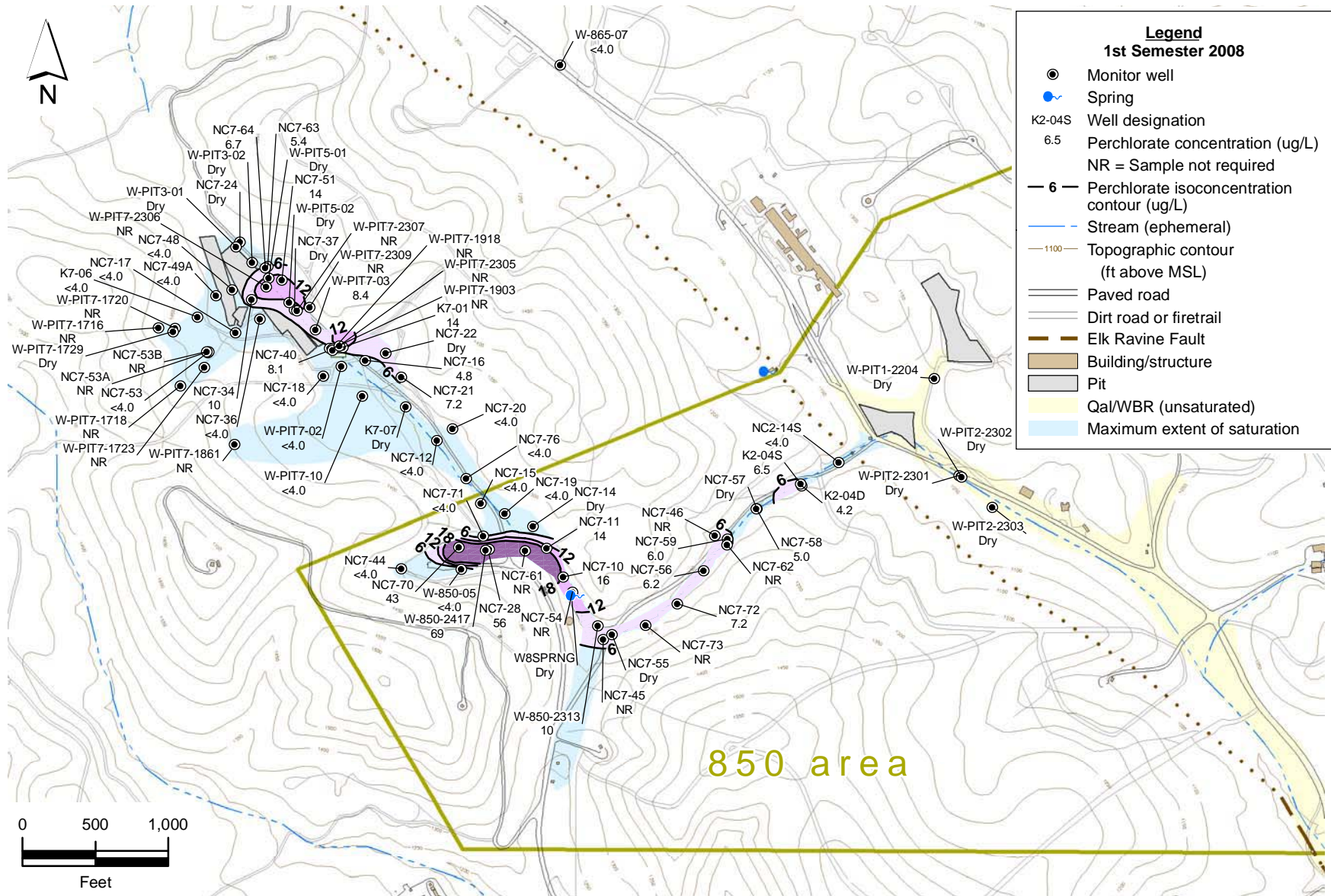
Figure 2.5-10. Building 850 area perchlorate isoconcentration contour map for the Qa1/WBR HSU.
