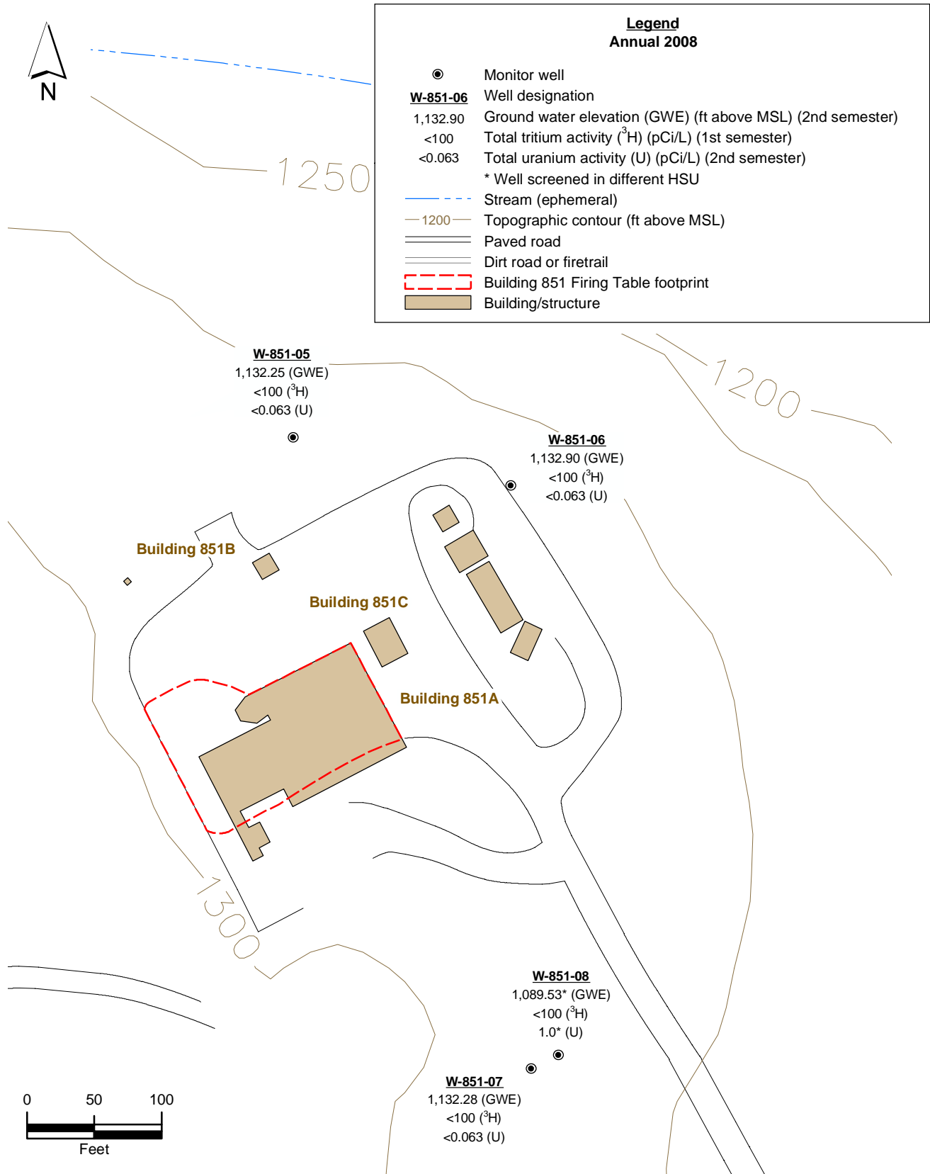
Figure 2.8-4. Building 851 Firing Table site map showing monitor well locations, ground water elevations, and tritium and uranium activities in the Tmss HSU.
