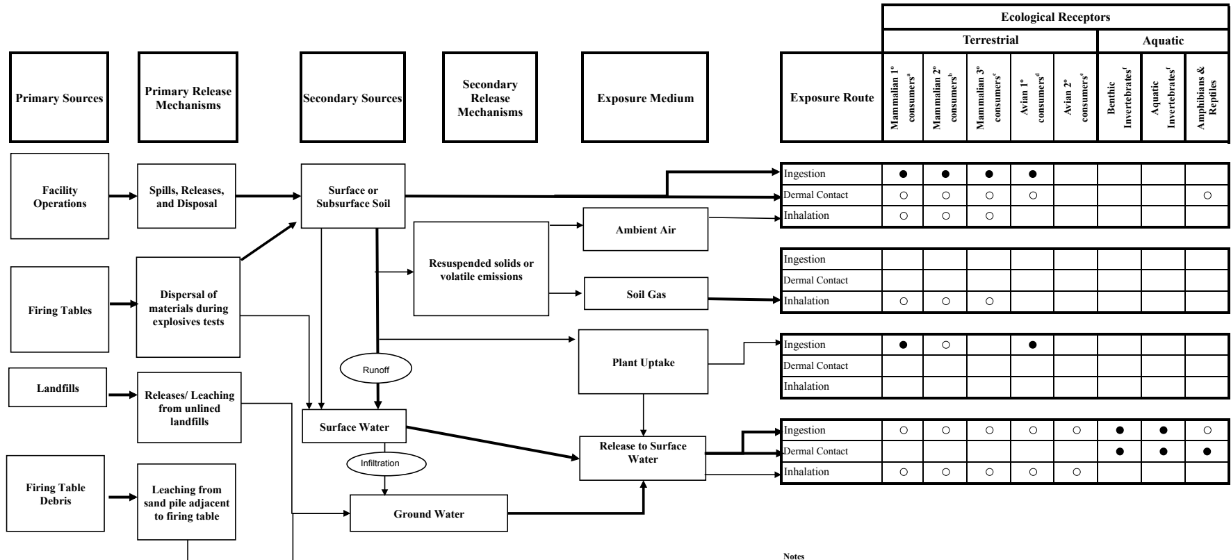
Figure 4.2-3. Generalized Conceptual Site Model for LLNL Site 300 Lawrence Livermore National Laboratory, Site 300, Livermore, California
