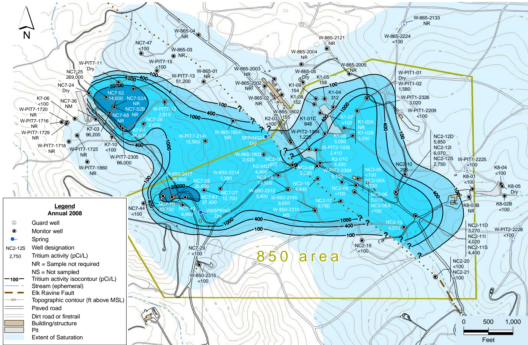
Figure 2.5-5. Building 850 area tritium activity isocontour map for the Tnbs_1/Tnbs_0 HSU.
