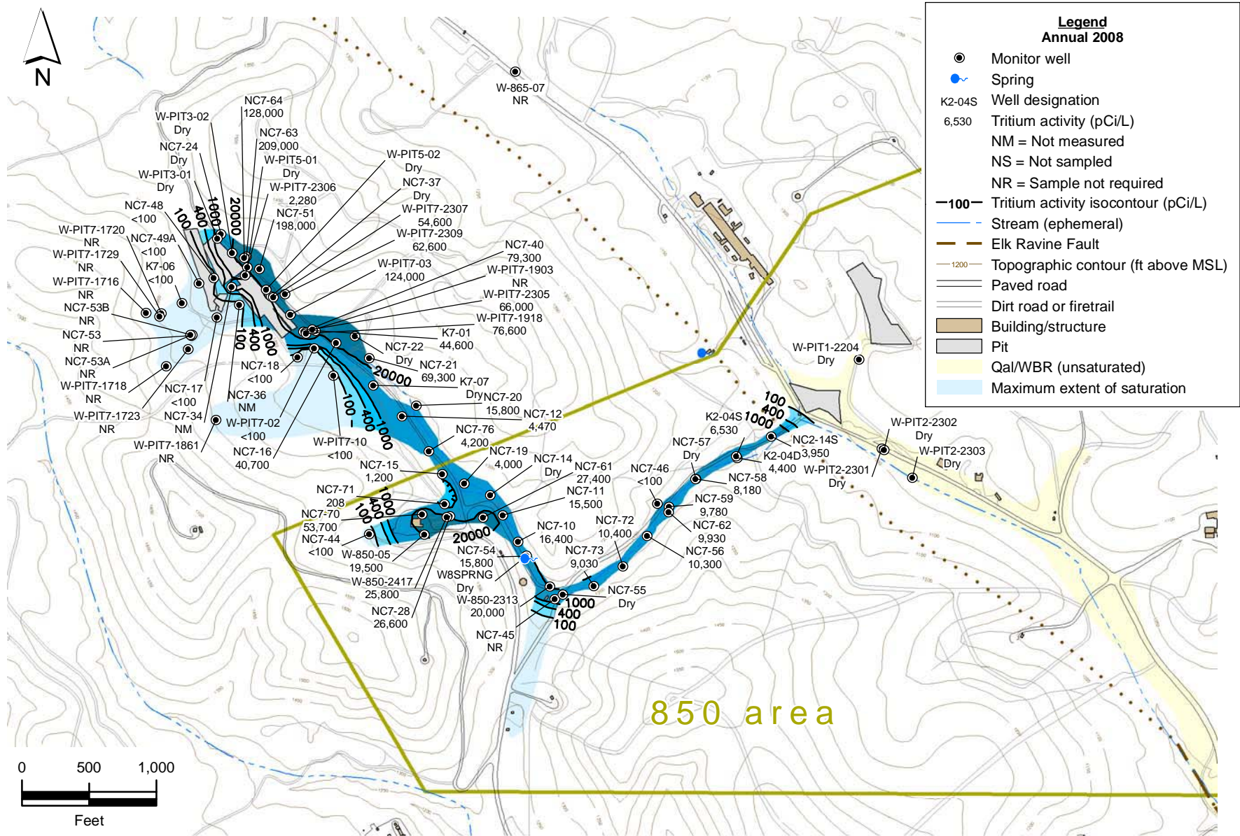
Figure 2.5-4. Building 850 area tritium activity isocontour map for the QaI/WBR HSU.
