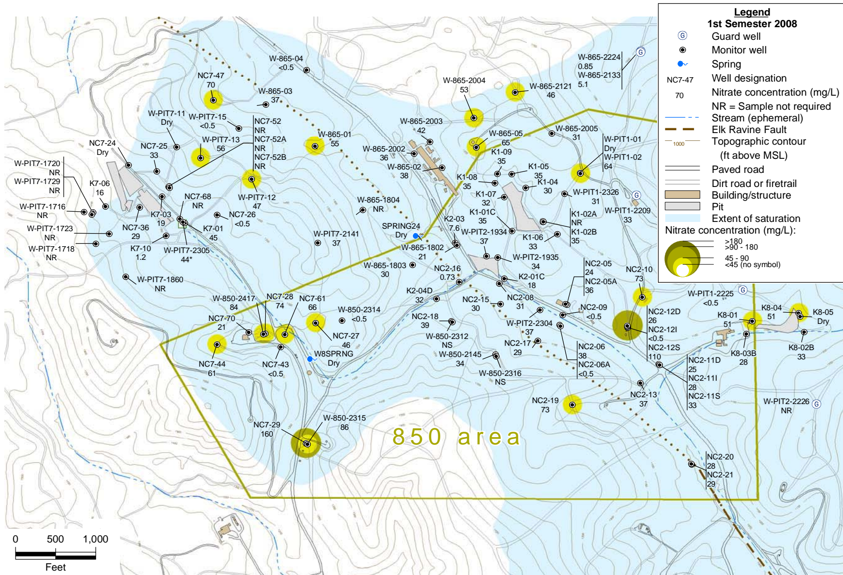
Figure 2.5-9. Building 850 area map showing nitrate concentrations for the Tnbs 1 /Tnbs 0 HSU.
