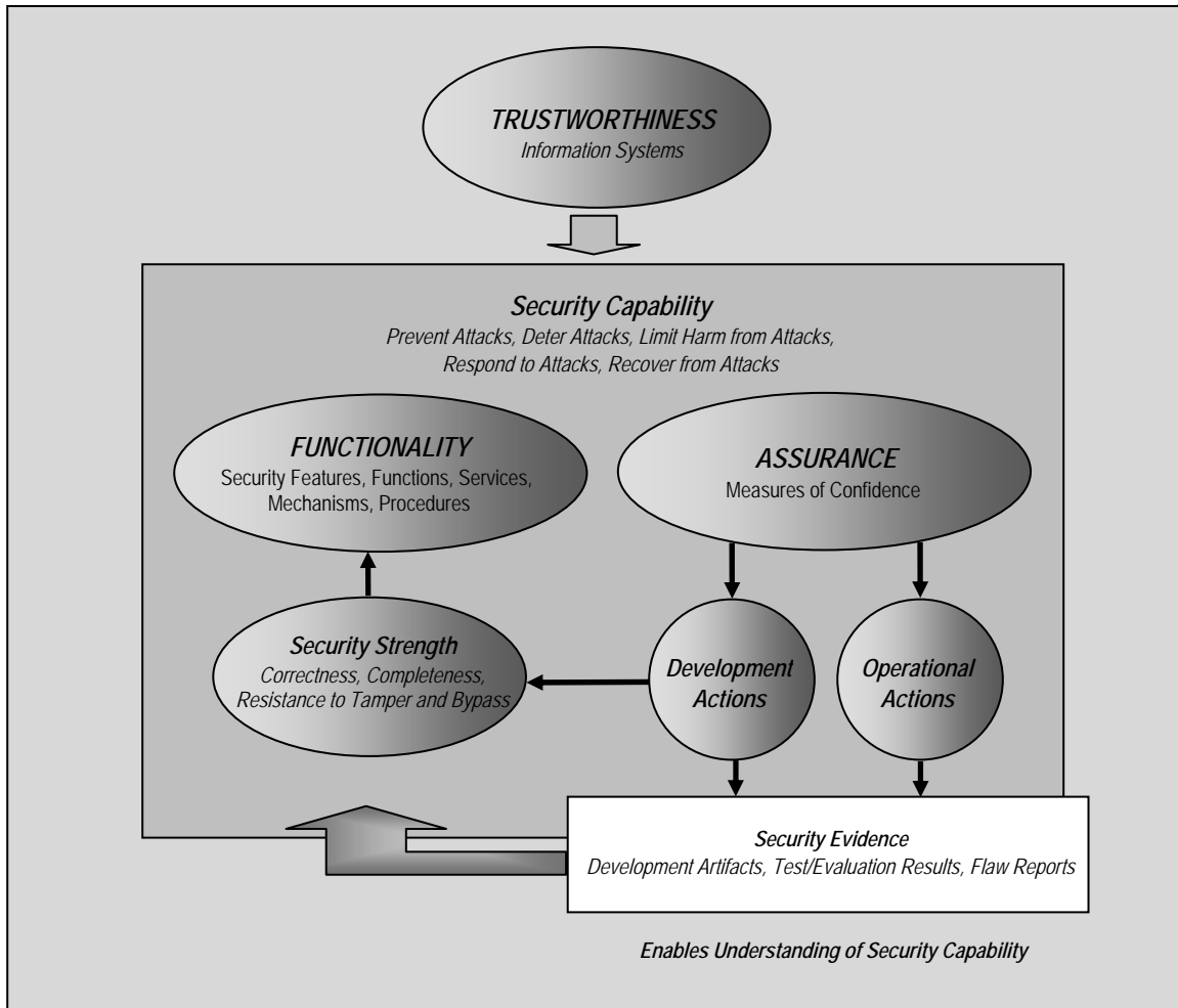
FIGURE 3: TRUSTWORTHINESS MODEL
