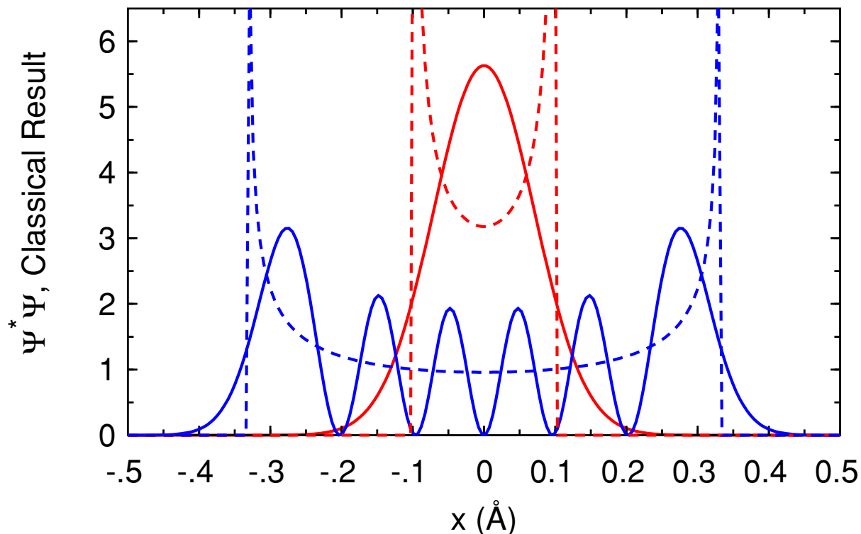
Figure 2: Quantum and classical probability of finding oscillator as a function of position.
