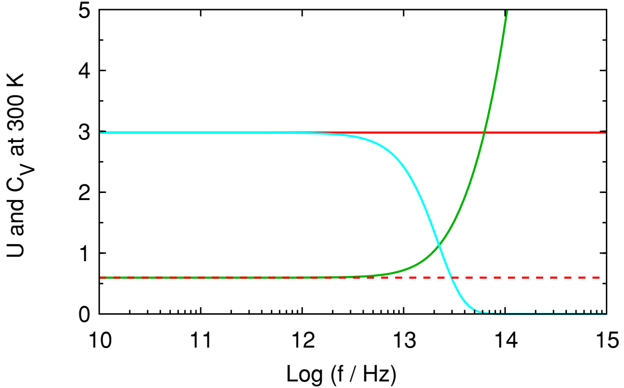
Figure 4: Harmonic oscillation at 300 K: average energy and heat capacity versus frequency
