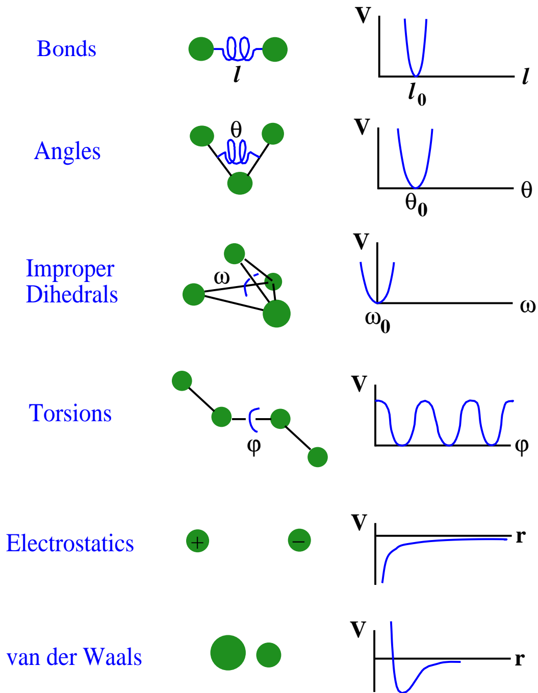
Figure 7: Interactions included in representative potential energy function for MD simulation.
