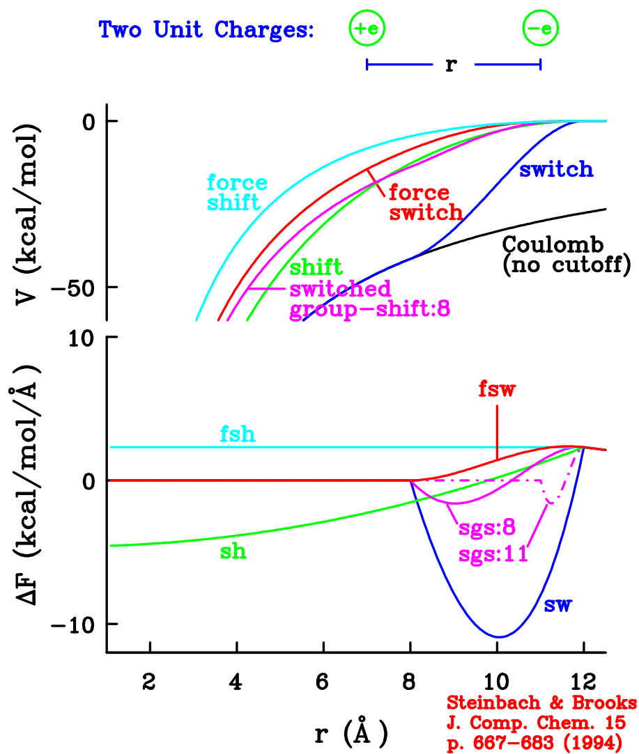
Figure 8: Potential energy and error in force calculated by some 'spherical cutoffs.'
