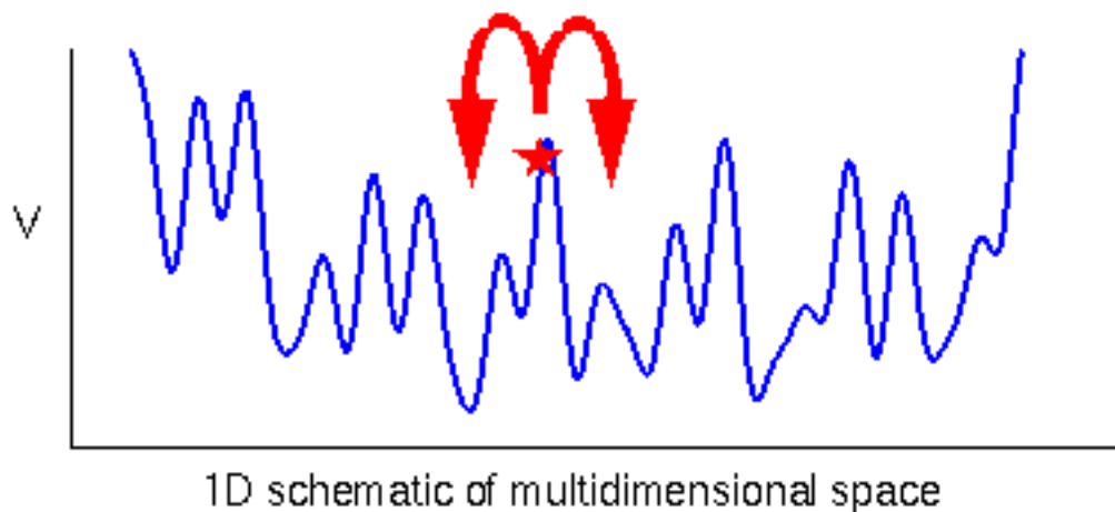
Figure 13: Simulated annealing can overcome barriers by heating and cooling the system.
