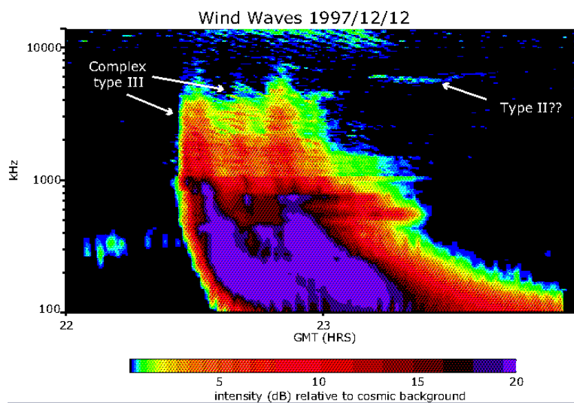
Figure 1.3. The 1997 December 12 complex type III burst that started below about 7 MHz, but was very intense at kilometric wavelengths (from Gopalswamy et al., 2000).
