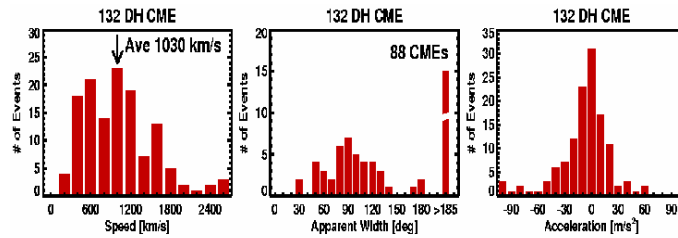
Figure 1.8. Speed, width and acceleration of 132 CMEs associated with DH type II bursts. Note that 88 CMEs were halo events.
