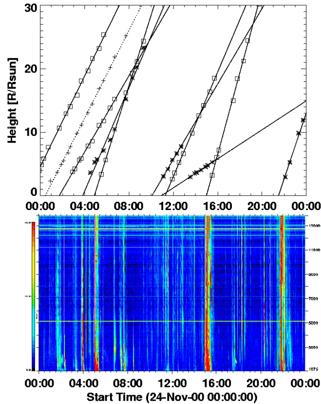
Figure 1.4. Height-time plots of all the CMEs that occurred on 2000 November 24 (top), along with the WAVES/RAD2 dynamic spectrum. Note that all the complex type III bursts are associated with major CMEs.
