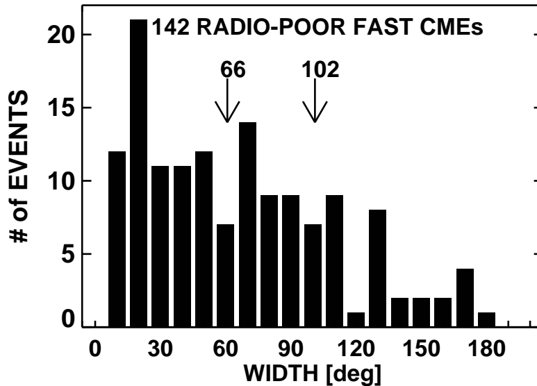
Figure 1.9. Histogram of fast CMEs (> 900 km/s) that did not have associated DH type II bursts. These have an average width of 66°, compared to the 102° for DH type II CMEs.
