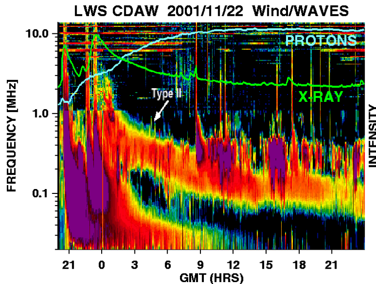
Figure 1.14. Wind/WAVES dynamic spectrum of the 2001 November 22 events. The type II burst (marked by arrow) of the second CME was intense and broadband. Both CMEs were associated with major flares as indicated by the GOES light curve (X-RAY) and the time profile of the solar energetic particle time profile.
