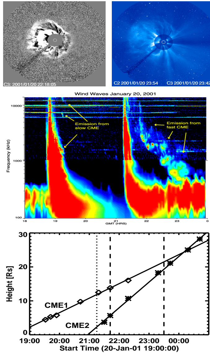
Figure 1.13. top: SOHO/LASCO difference image at 22:18 UT on 2001 January 20 showing two CMEs that became indistinguishable in the 23:42 UT image. middle: DH type II bursts associated with the two fast CMEs. The type II burst of CME1 was weak and of narrow band compared to the intense broadband type II associated with CME2. bottom: Height-time plots of the two CMEs with the vertical dashed lines showing the duration of the type II burst of CME2. The vertical dotted line shows the onset of the complex type III burst that mark the onset of CME2.
