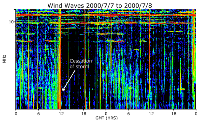
Figure 1.6. Type III storm activity (vertical streaks) observed by Wind/WAVES during 2000 July 7-8. The noise storm was interrupted by a CME on July 7 around 12 UT, but recovers by 20 UT to the original intensity.
