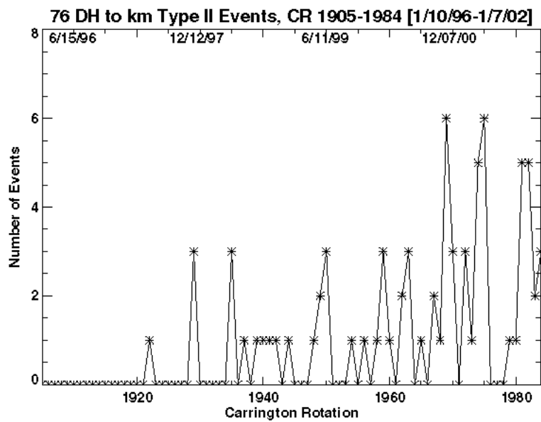
Figure 1.16. Number of type II bursts that begin in the DH domain and continue to the kilometric domain plotted as a function of time (Carrington Rotation number and UT). Note that there are several rotations with no such long-lasting type II bursts.
