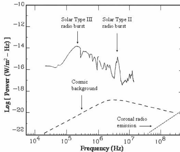
Figure 1.1. Plot showing the level of IP radio burst (types II and III) flux as compared to the cosmic background noise and the quiet coronal emission. The low-frequency end of the solid curve represents in situ plasma frequency. The high-frequency end corresponds to the ionospheric cut-off.
