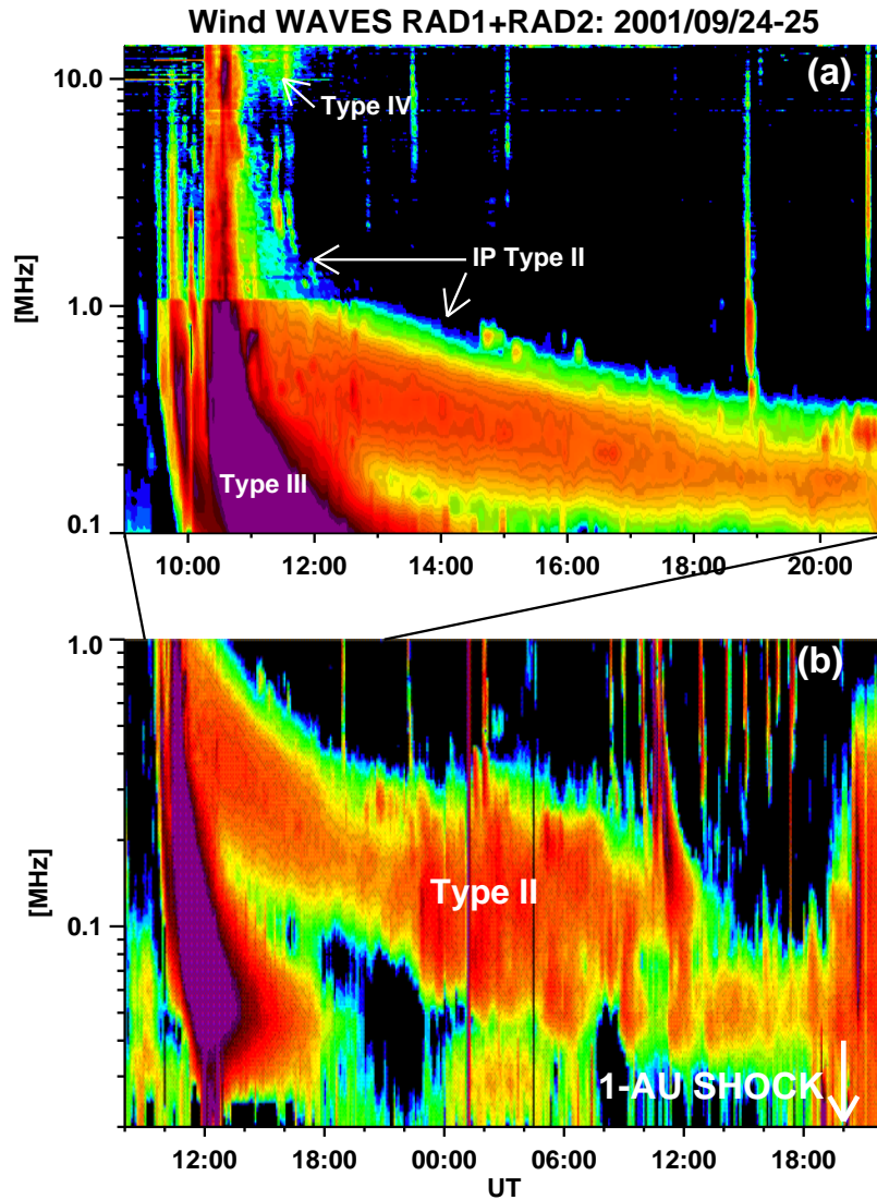
Figure 1.7. IP Type II burst of 2001 September 24-25. The top panel shows the dynamic spectrum over the entire WAVES spectral range. The bottom panel shows the complete evolution of the type II burst until the shock arrived at 1 AU (marked by arrow). The complex Type III, which appeared at the beginning of the event and the associated type IV burst are marked. The collecting area of the antenna in the high-frequency domain is smaller, so the type II burst is faint.
