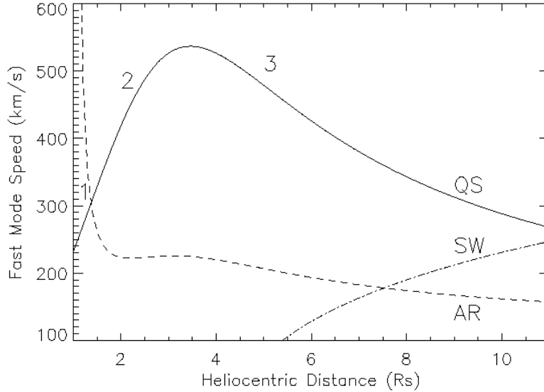
Figure 1.11. Radial profile of the fast mode speed ( V_F ) in the active region (AR) and quiet (QS) corona. The solar wind speed profile (SW) is also shown. The sharp increase of V_F in region 1 prevents shock formation in the core of active regions. Shock formation is easier in regions 2 and 3 because of lower V_F .
