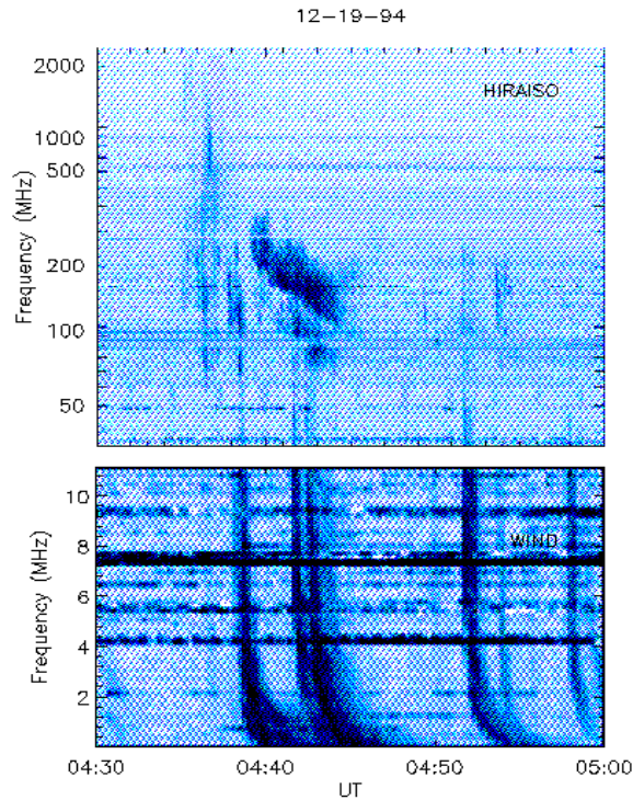
Figure 1.2. A combination of ground-based (Hiraiso - top) and Wind/WAVES (bottom) dynamic spectra showing a number of isolated type III bursts (vertical features). The slanted feature is the type II burst. It is clear that some metric type III bursts continue to lower frequencies, and some don't.
