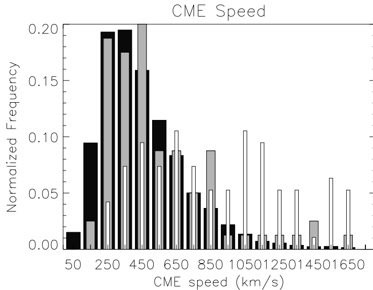
Figure 1.10. Speed distribution of CMEs associated with metric type II bursts as compared to that of general population of CMEs (dark), and DH CMEs (white).
