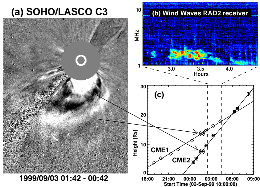
Figure 1.12. (a) Two CMEs on 1999 September 3 as observed by SOHO/LASCO, and (b) the associated continuum radio emission detected by Wind/WAVES around 2 MHz. (c) The height-time plots of the two CMEs with the duration of the radio emission marked by vertical lines.
