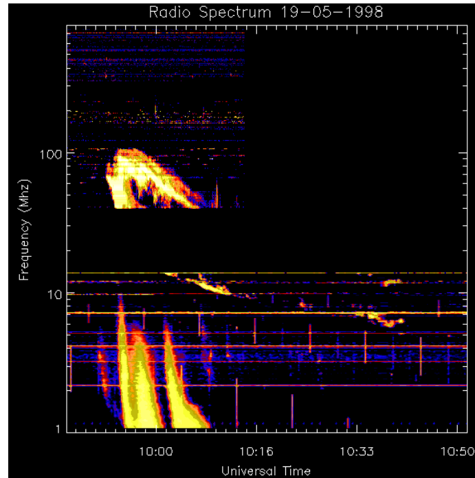
Figure 1.5. A hybrid dynamic spectrum consisting of Potsdam data (top, above 40 MHz) and Wind/WAVES (bottom, below 14 MHz). The Complex type III bursts start only below 10 MHz and delayed with respect to the onset of the type II burst.
