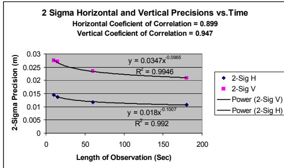
Figure 15 – Plot 2σ Horizontal and Vertical Precisions relative to Length of Observation.
