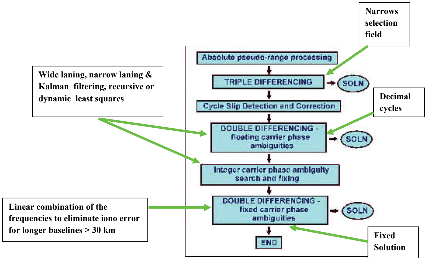
Diagram III-2 – General Flow of Ambiguity Resolution [graphic: Rizos (1999)]
