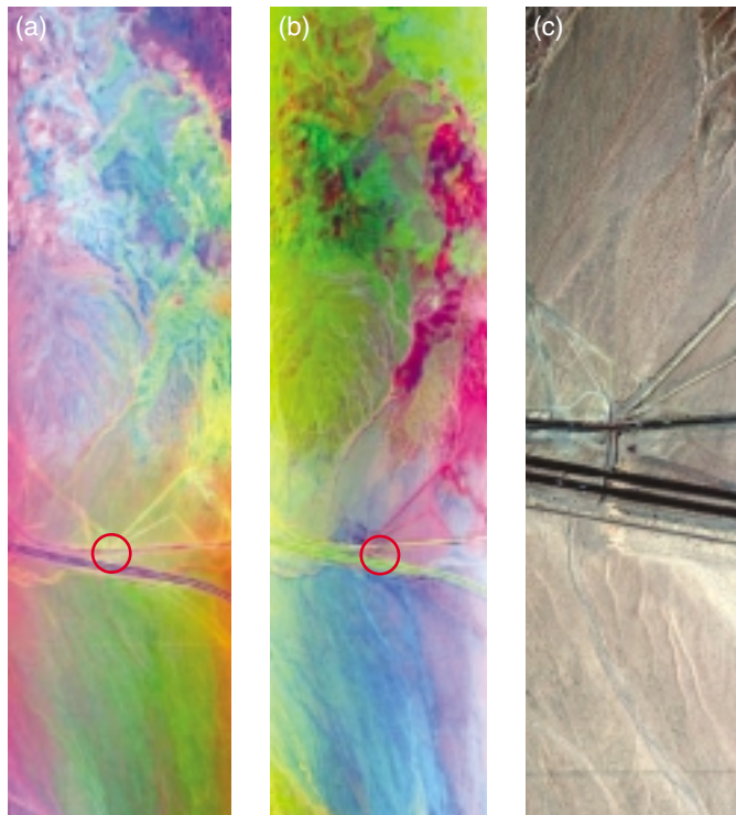
Three views of a pipeline leak. (a) Minimum noise fraction (MNF) transformation in pseudo-color, showing leak area west of Ludlow, California. (b) Using different MNF transformed bands emphasizes features differently and is a common technique for sorting out what is seen in the imagery. (c) A true color, three-band image at 3-meter resolution.
