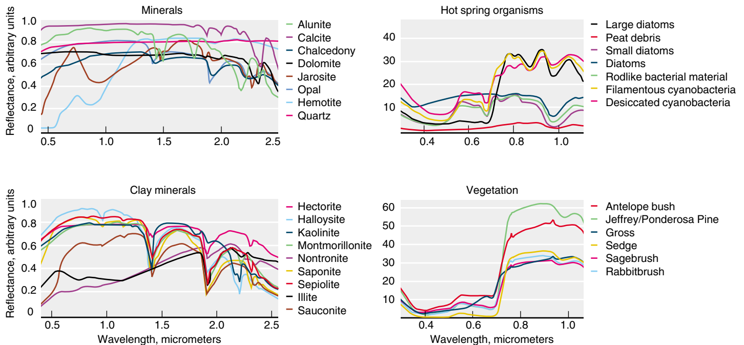
Hyperspectral images provide distinctive spectral shapes that allow identification of mineral types, clay soil types, plant species, plant health within species types, and hot and cold spring microorganisms. These spectra are from Mammoth Mountain–Long Valley hyperspectral imagery but are representative of most areas.
