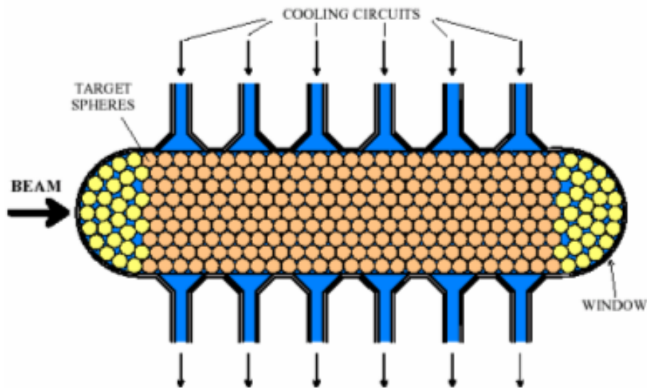
Fig. 1: Schematic section through the granular target
