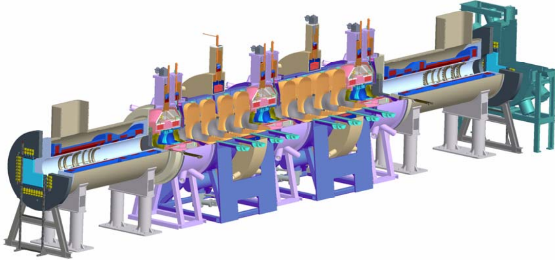
Fig. 2: Drawing of the MICE experiment [9]. The beam enters the experiment from the bottom left-hand corner. The beam first passes through one of the scintillator hodoscopes that form the time-of-flight system. After passing through the upstream spectrometer, the beam passes through three absorber/focus-coil modules and two cavity/coupling-coil modules before it passes through the downstream spectrometer and, a second time-of-flight hodoscope, the downstream Cherenkov counter and is stopped in the electromagnetic calorimeter. The beamline and upstream instrumentation is not shown.
