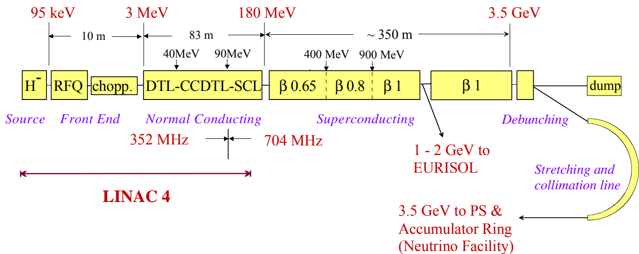
Fig. 4: The SPL
