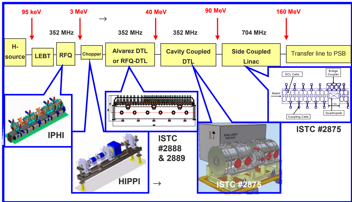
Fig. 5: LINAC4
