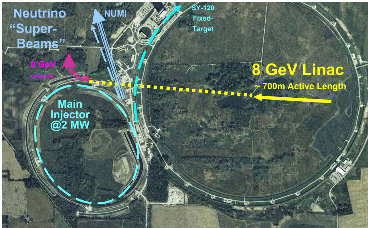
Fig. 9: The Fermilab proton complex with a 8 GeV SPL
