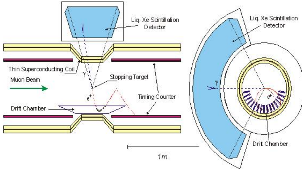
Fig. 2: A sketch of the MEG detector
