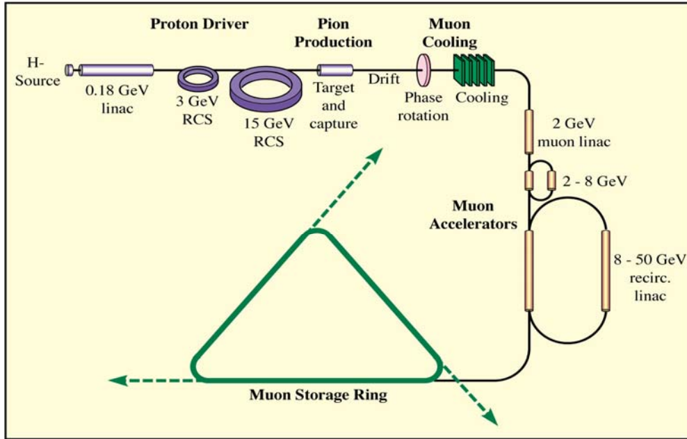
Neutrino Factory at RAL
