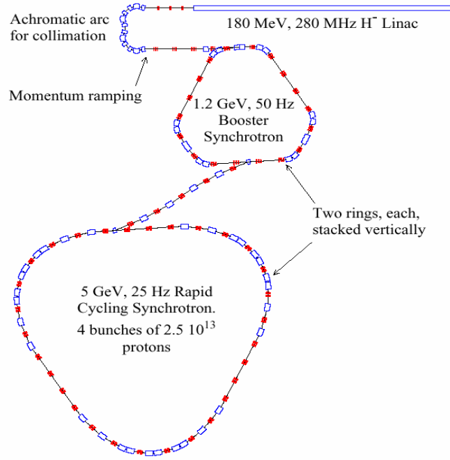
Fig. 2: Schematic of the 5 GeV, 50 Hz RCS design
