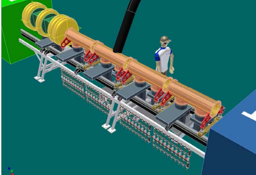
Fig. 3: Drawing of the radio-frequency quadrupole and chopper for the RAL proton front-end test stand
