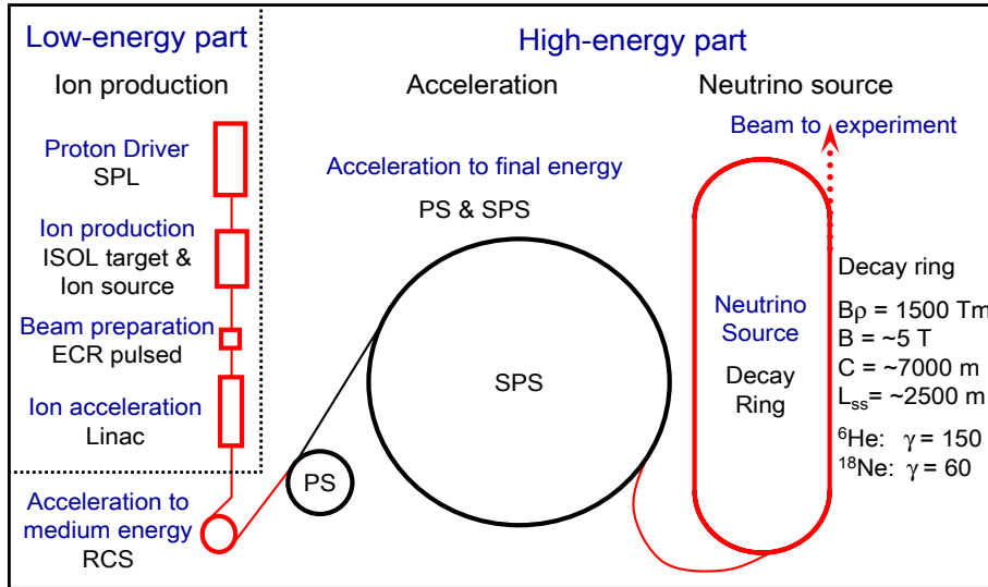
Fig. 1: CERN betabeam conceptual design
