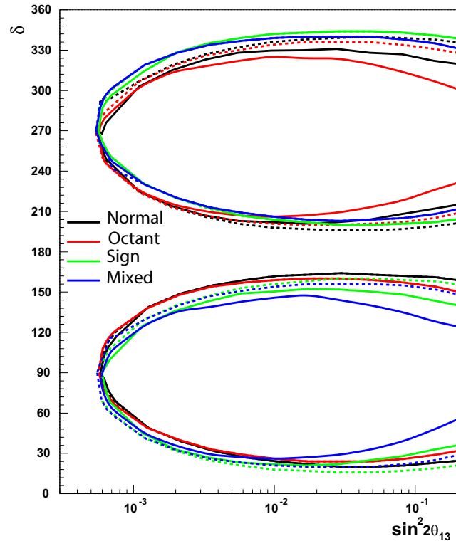
Fig. 11: Leptonic CP violation discovery potential at 3\sigma ( \Delta\chi^2 > 9.0 ) of the betabeam with \gamma = 100 computed for the four different options about the true values of \text{sign}(\Delta m_{23}^2) and \theta_{23} and including all the possible degeneracies (see text). Dotted curves are computed neglecting the effects of the clone solutions. Taken from Ref. [106].
