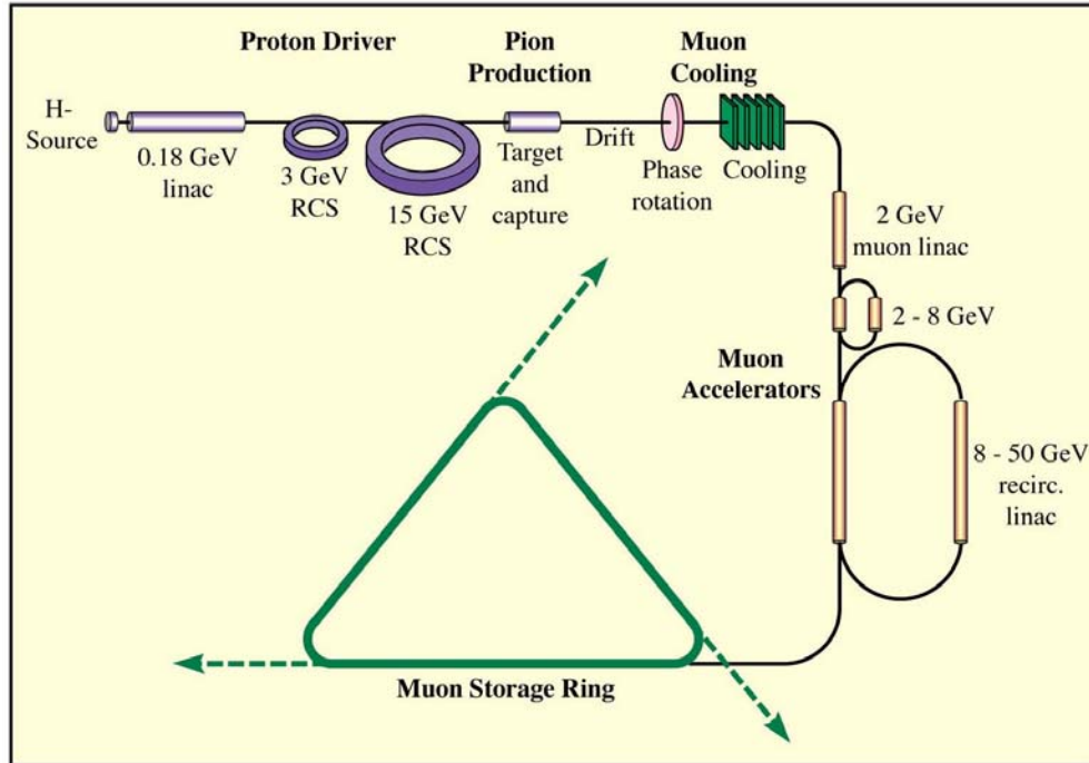
Fig. 1: Neutrino Factory at RAL
