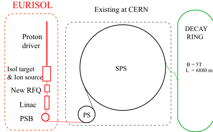
Fig. 9: A schematic layout of the betabeam complex. At left, the low-energy part is largely similar to the EURISOL project [99]. The central part (PS and SPS) uses existing facilities. At right, the decay ring has to be built.
