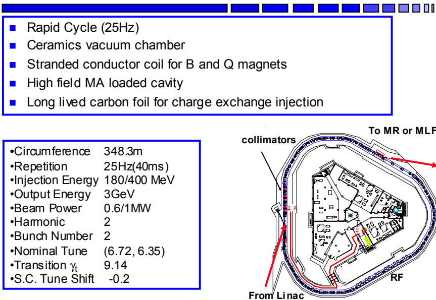
Fig. 12: Layout of the JPARC 3 GeV machine
