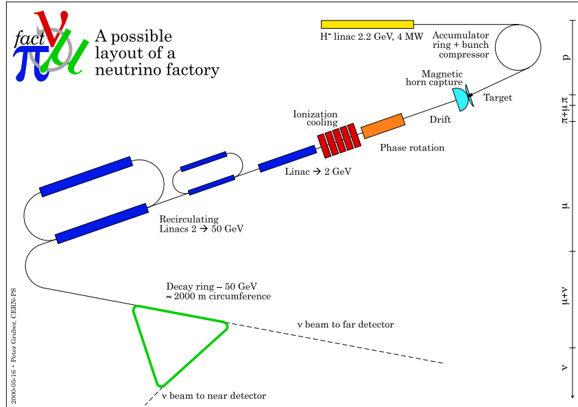
Fig. 13: Schematic layout of a Neutrino Factory
