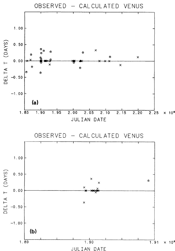
FIG. 1. (a) Observed minus calculated time for a given separation for Venus. The circles represent the observations recorded as occultations for which the closest approaches occurred during the daytime. The triangles represent the recorded occultations where the closest approaches occurred during the night. The \times 's represent the records of "fans" or appulses. (b) This is the same as (a) but shows the detail from JD 1890000 to 1910000.
