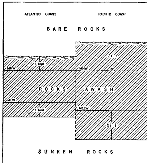
FIGURE 57—Planes of reference for rocks
