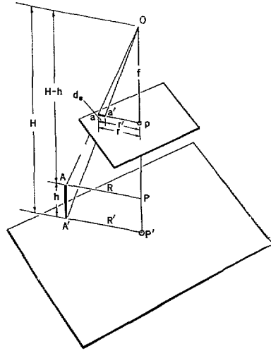
FIGURE 3.6—The magnitude and direction of relief displacement
