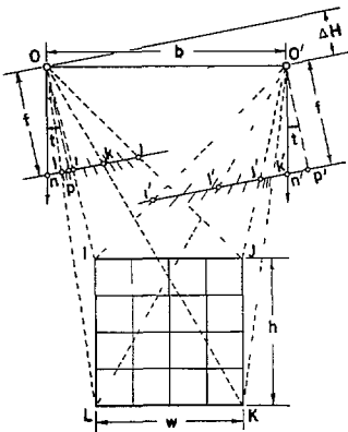
FIGURE 3 21—Condition in taking equally tilted photographs
