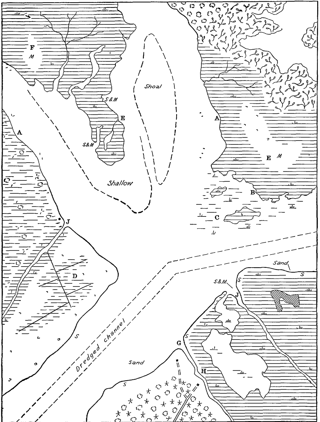
FIGURE 5 6a —Alongshore physical features on a shoreline manuscript
