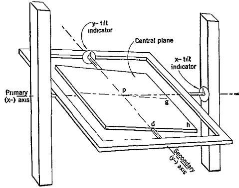
FIGURE 3 48 —Gimbal mechanism of the rectifier of the Coast and Geodetic Survey
