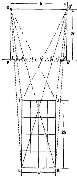
FIGURE 3.17 —Deformation caused by an increase in viewing distance
