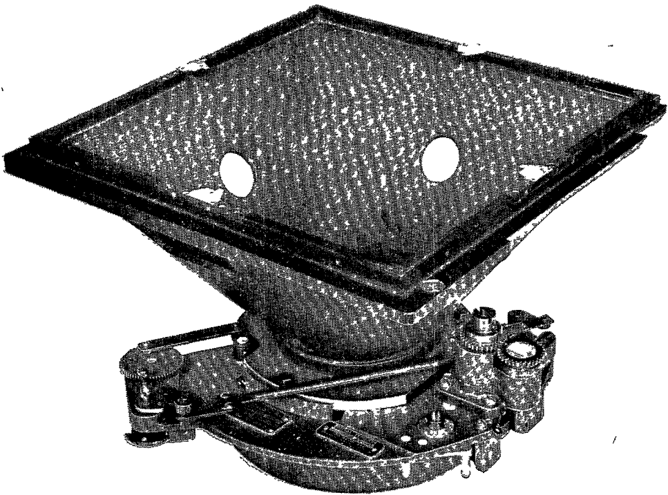
FIGURE 24—Inner cone of cartographic camera
