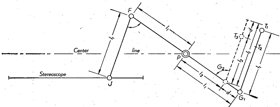
FIGURE 6.5.—The stereoscope-pantograph mechanism.
