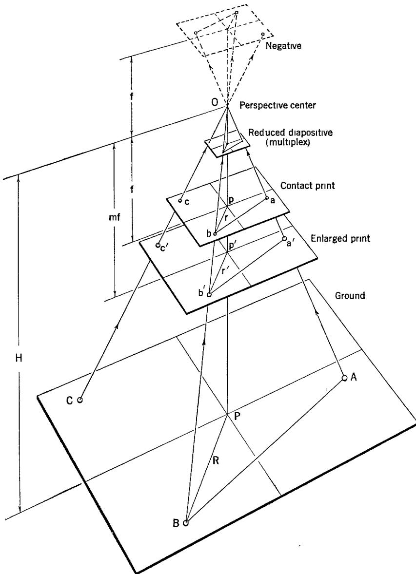
FIGURE 33—The perspective relation of the various forms of a photograph
