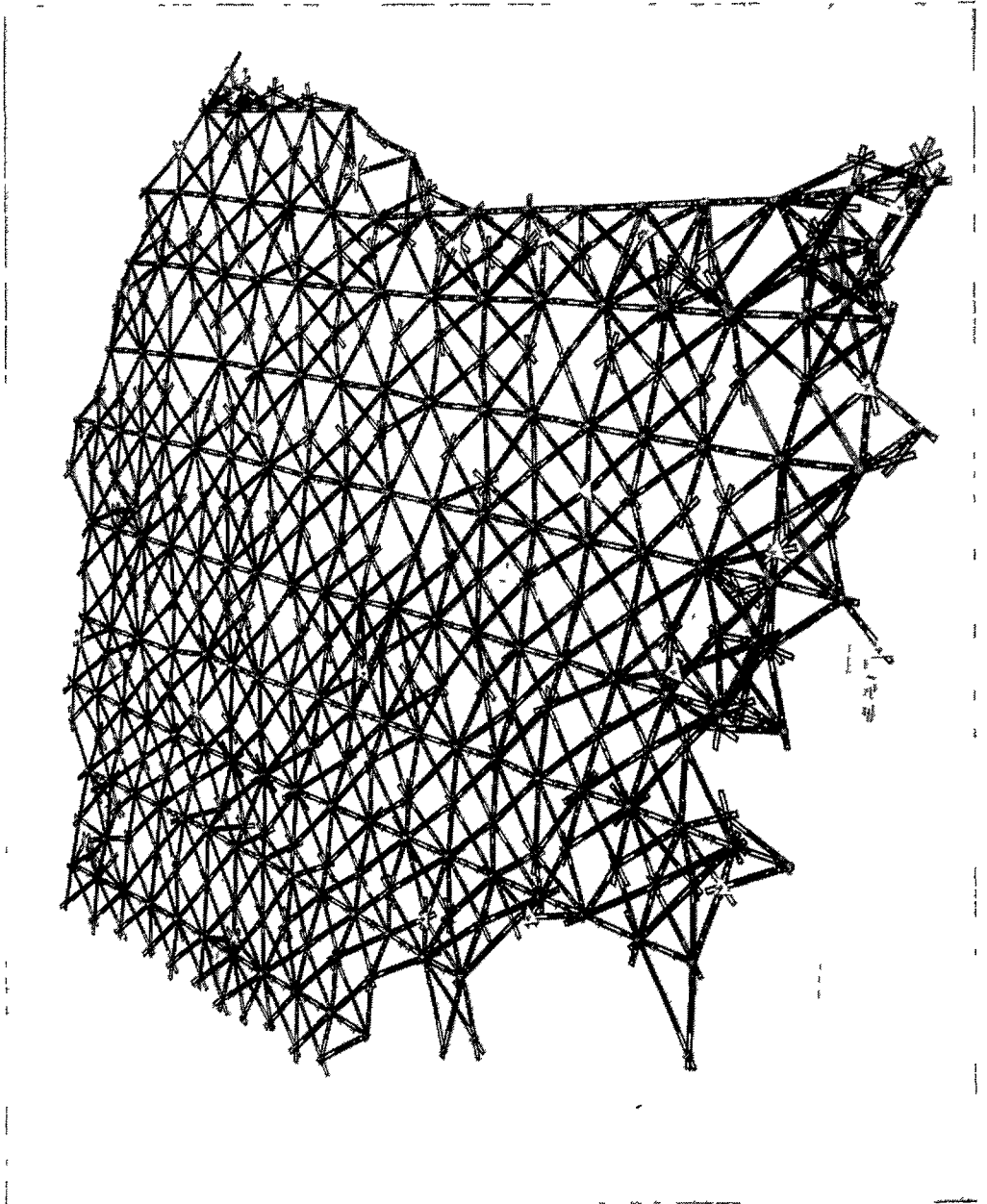
FIGURE 4 19.—Radial plot assembly with spider templets
