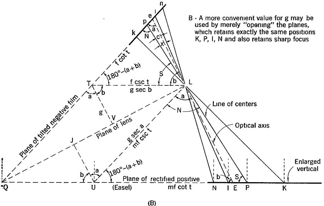
FIGURE 3 46 —Theoretical and practical rectification
