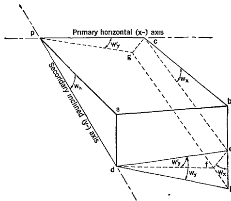
FIGURE 3 49 —Relations of component tilt angles
