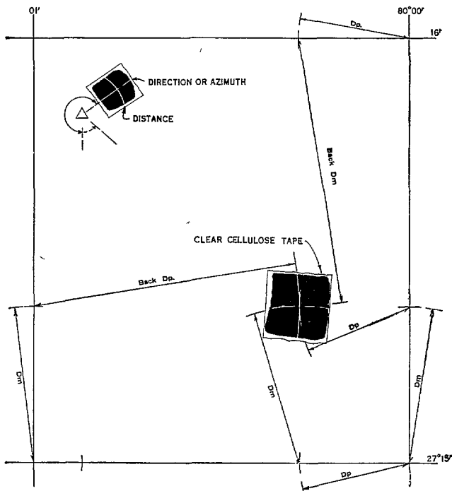
FIGURE 46—Plotting by dms and dps
