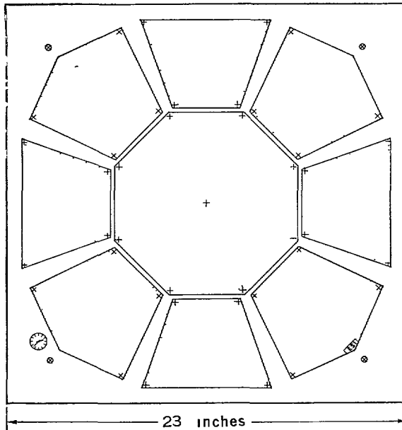
FIGURE 2 8 —Nine lens negative
