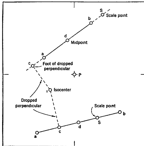
FIGURE 3 35 —Scale point construction
