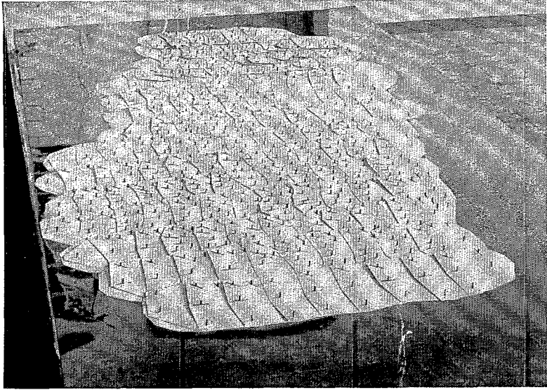
FIGURE 4.21.—Radial-plot assembly with slotted templets (Courtesy Soil Conservation Service).
