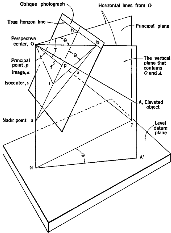
FIGURE 3 62—Horizontal angle from an oblique photograph
