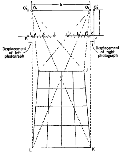
FIGURE 3 19 —Deformation caused by separation of photographs
