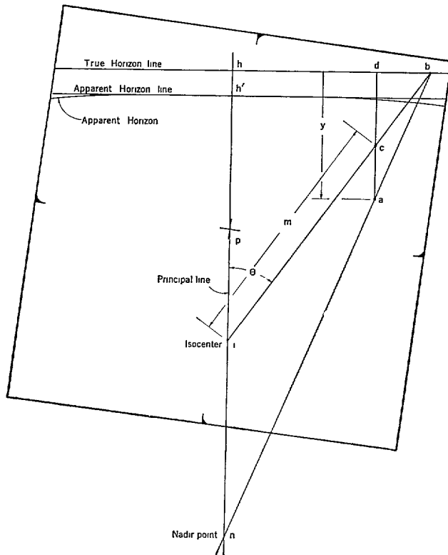
FIGURE 3 61—Horizontal and vertical angles from an oblique photograph
