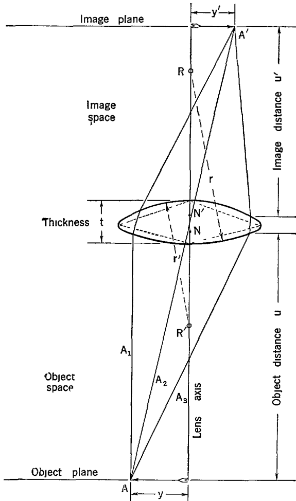
FIGURE 3 2—Image formation with a simple lens
