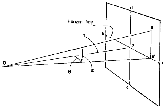
FIGURE 3 57—Geometry of the horizontal photograph
