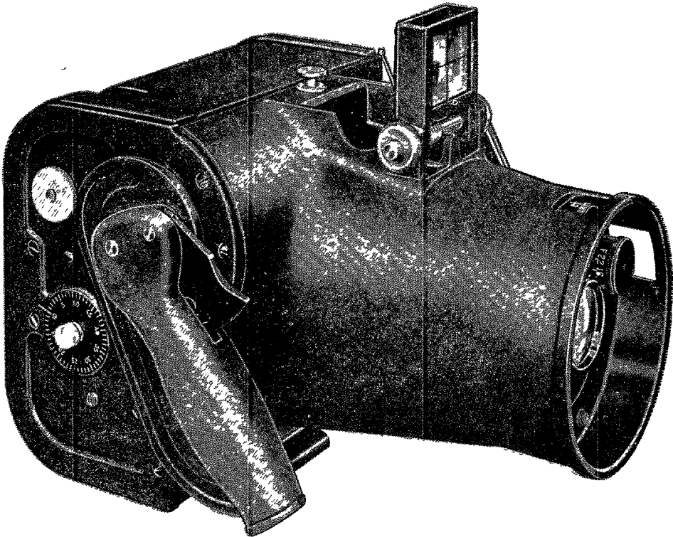
FIGURE 25 —K-20 camera
