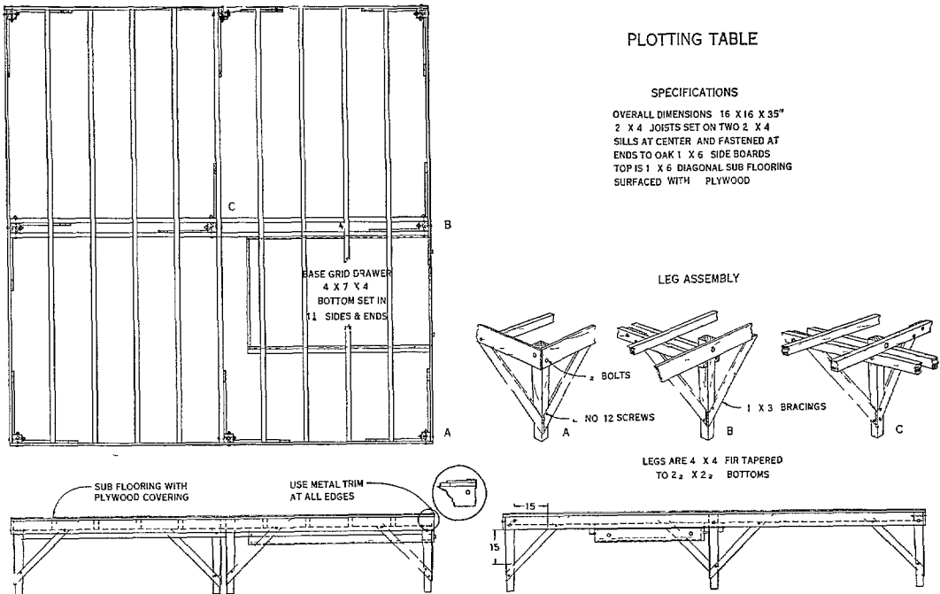
FIGURE 1 10 —Plotting table
