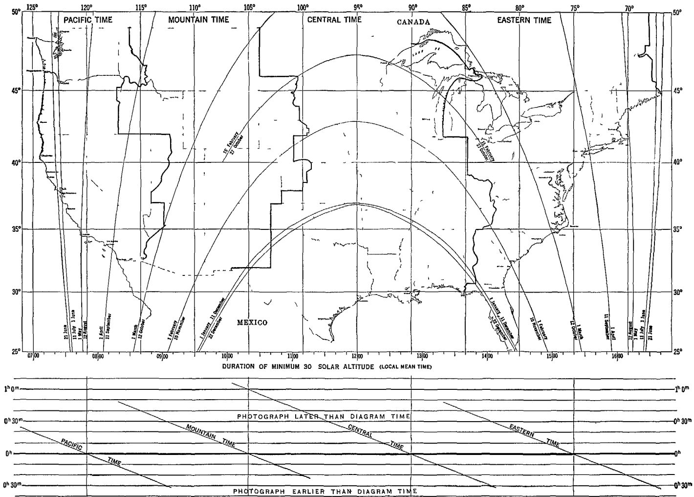
FIGURE 2 11 —Duration of Minimum Solar Altitude
