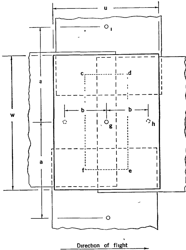
FIGURE 37—The usual overlapping arrangement of aerial photographs
