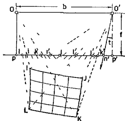
FIGURE 3 23 —Deformation caused by unequal tilt
