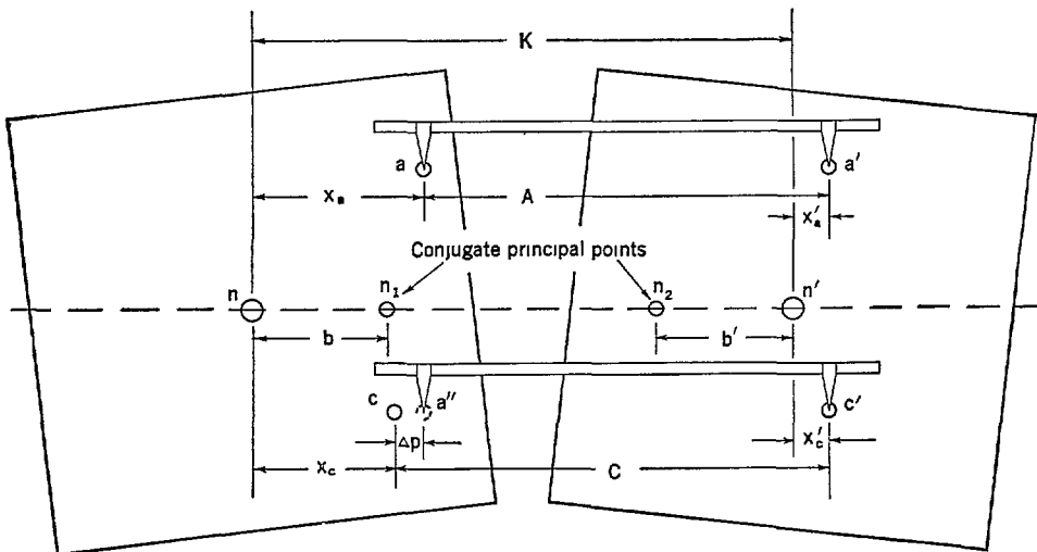
FIGURE 3.11—How difference in parallax can be measured with dividers
