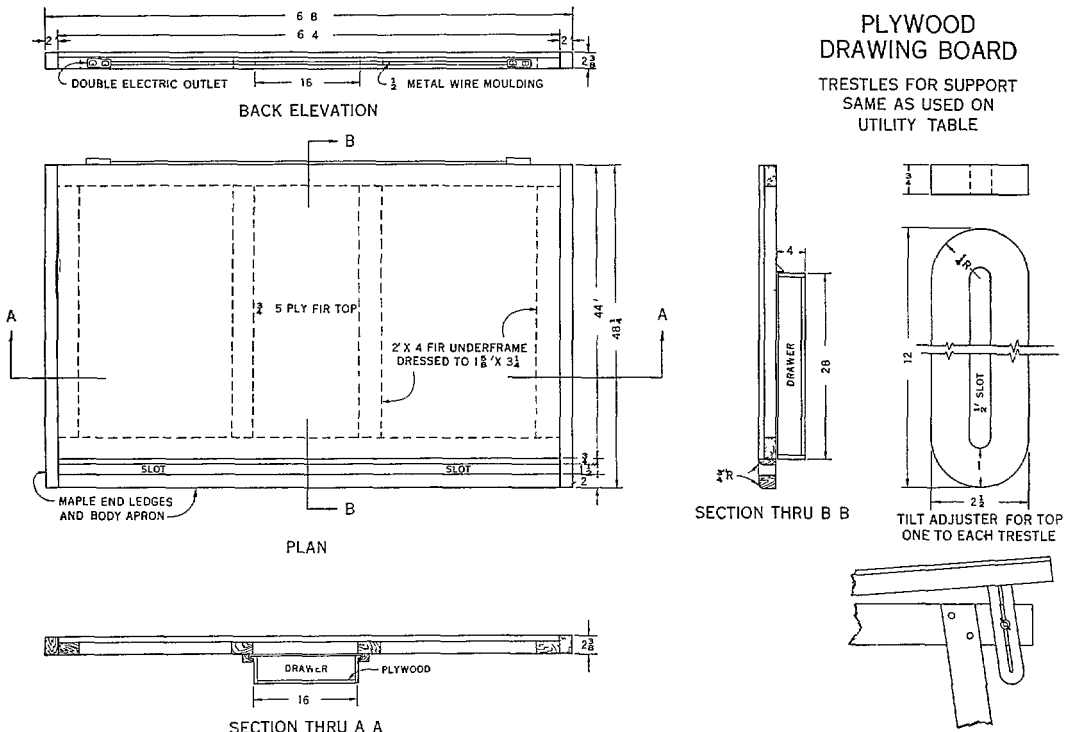
FIGURE 17—Plywood drawing board
