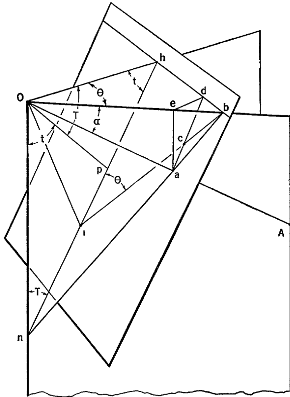
FIGURE 3 63 —Vertical angle from an oblique photograph
