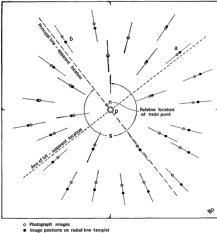
FIGURE 340—Sketch showing typical displacement pattern due to tilt, scale, and moderate relief
