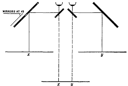
FIGURE 1 14—Principle of mirror stereoscope
