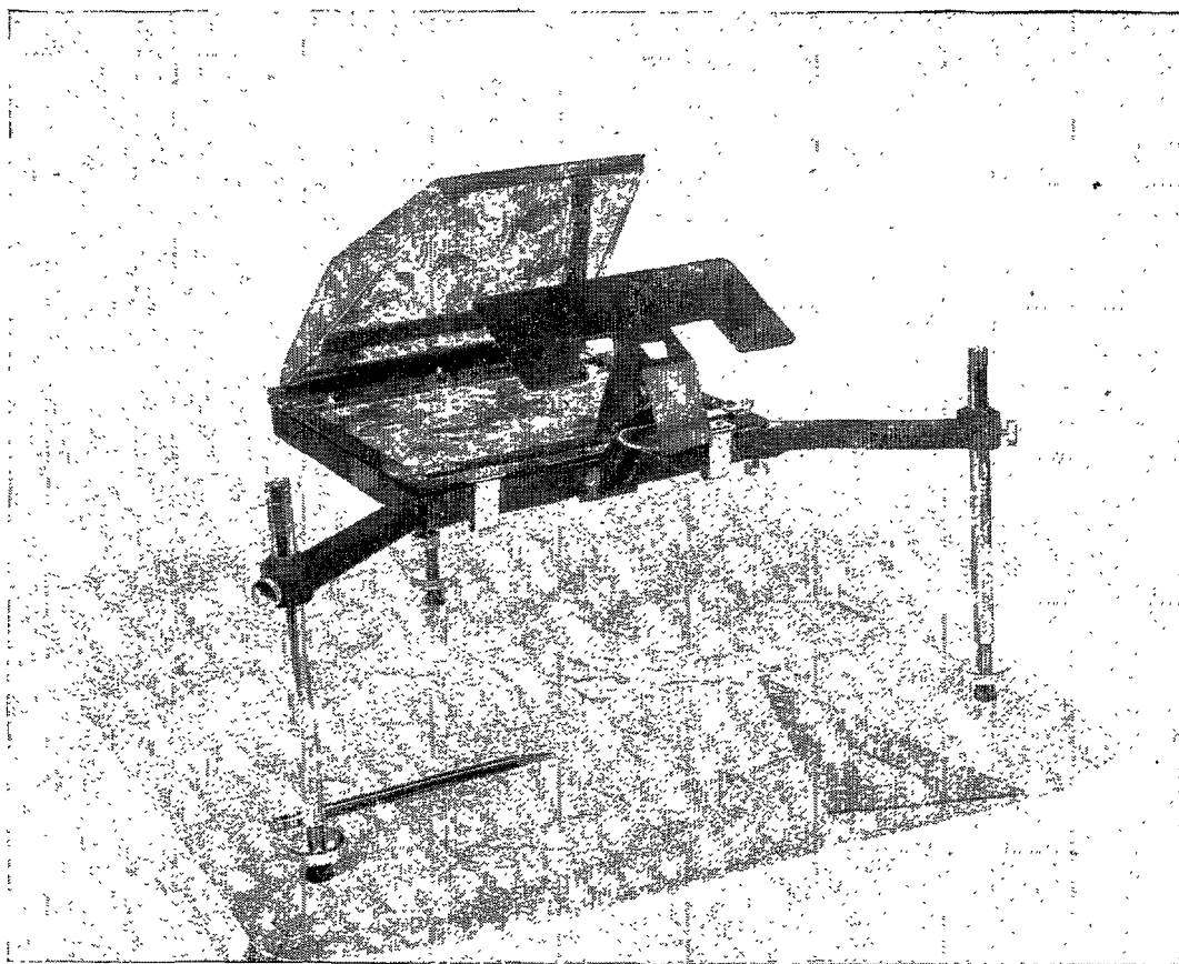
FIGURE 9.5.—Vertical sketchmaster.
