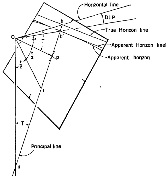
FIGURE 3 60—Geometry of the high oblique photograph
