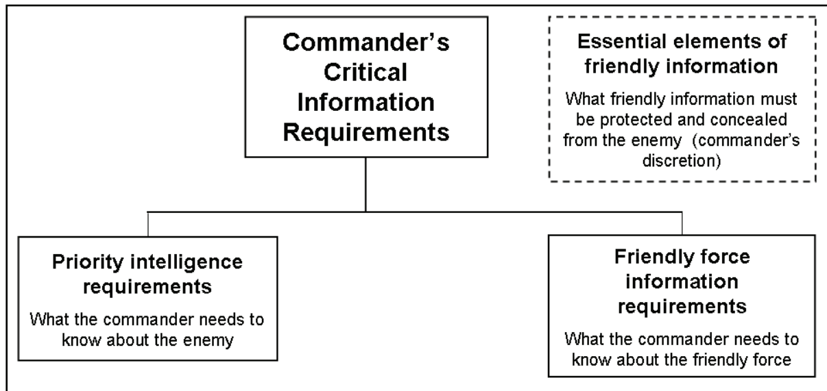
Figure 5-2. CCIR
