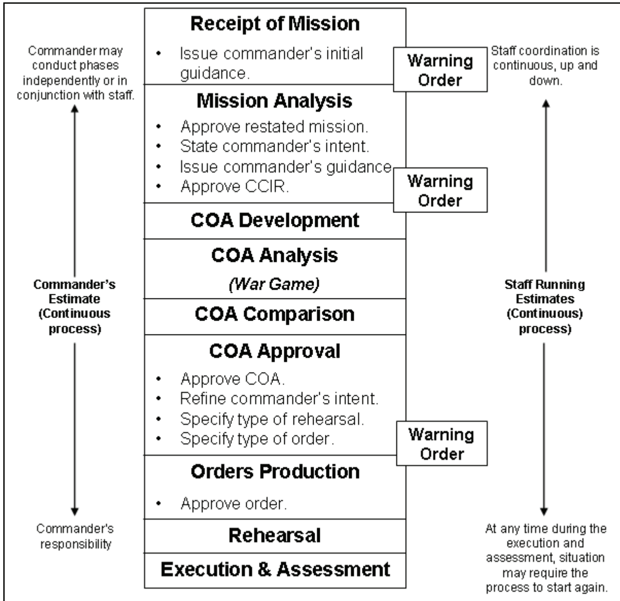
Figure 5-5. The MDMP
