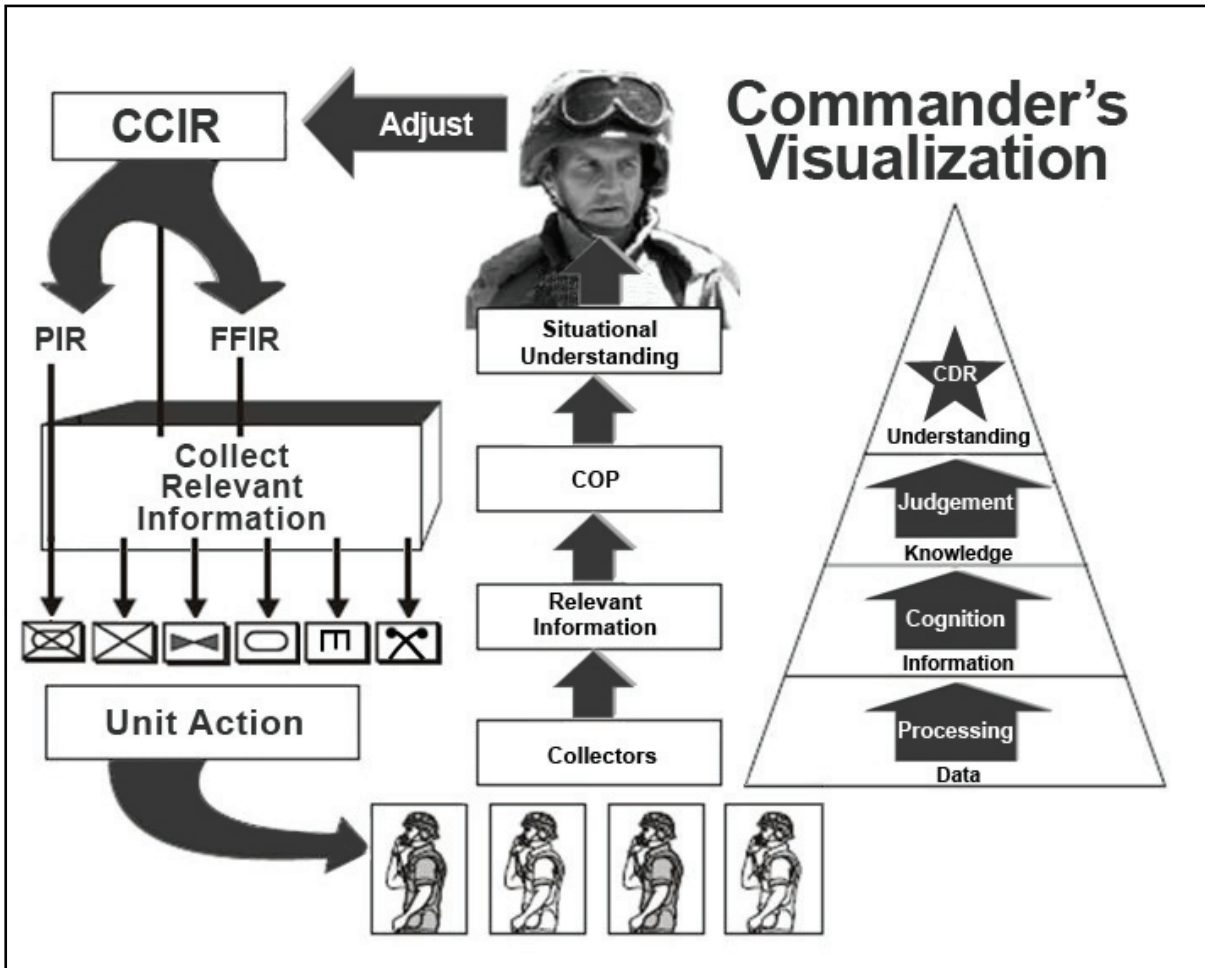
Figure 5-3. Developing SU
