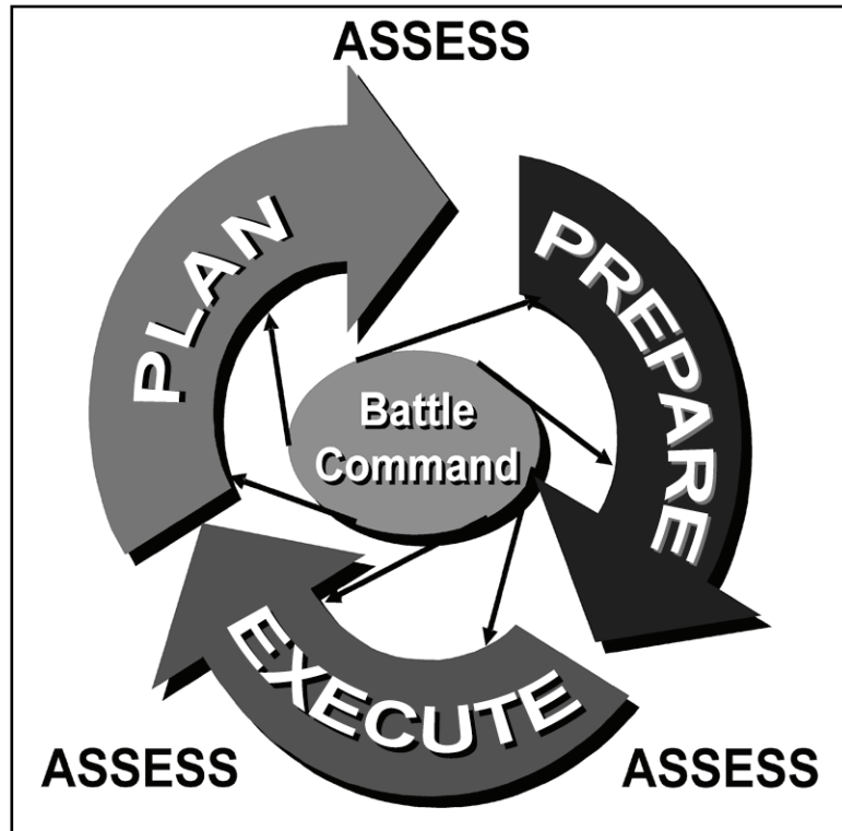
Figure 5-4. Operations process
