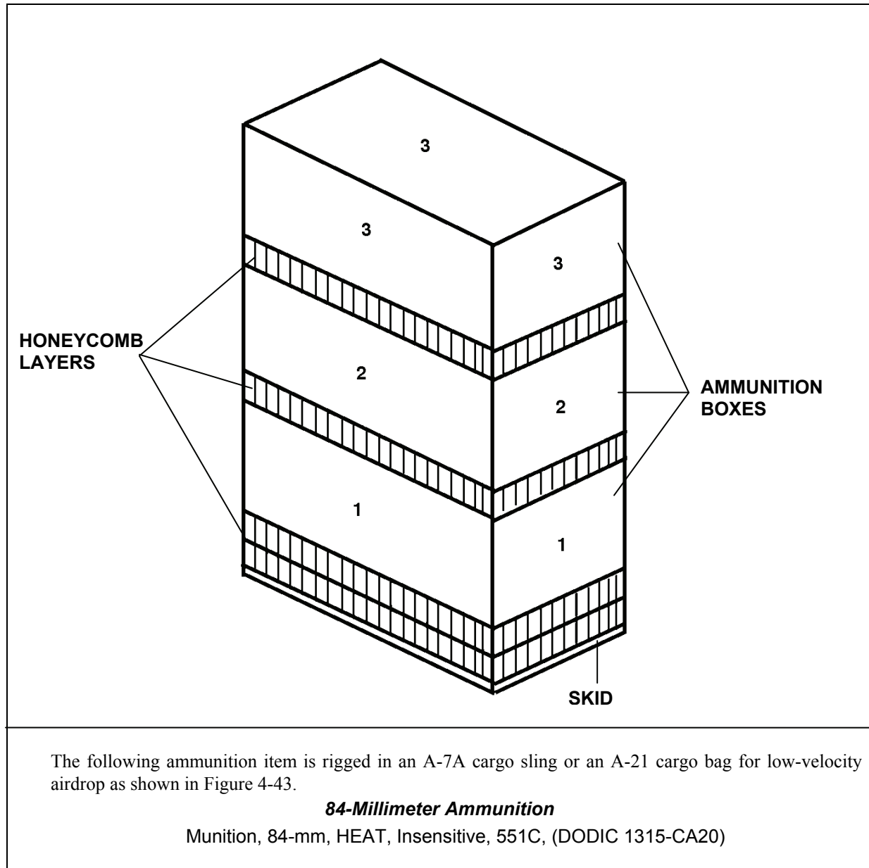
Figure 4-43. Ammunition Layout in an A-7A Cargo Sling or an A-21 Cargo Bag for Low-Velocity Airdrop
