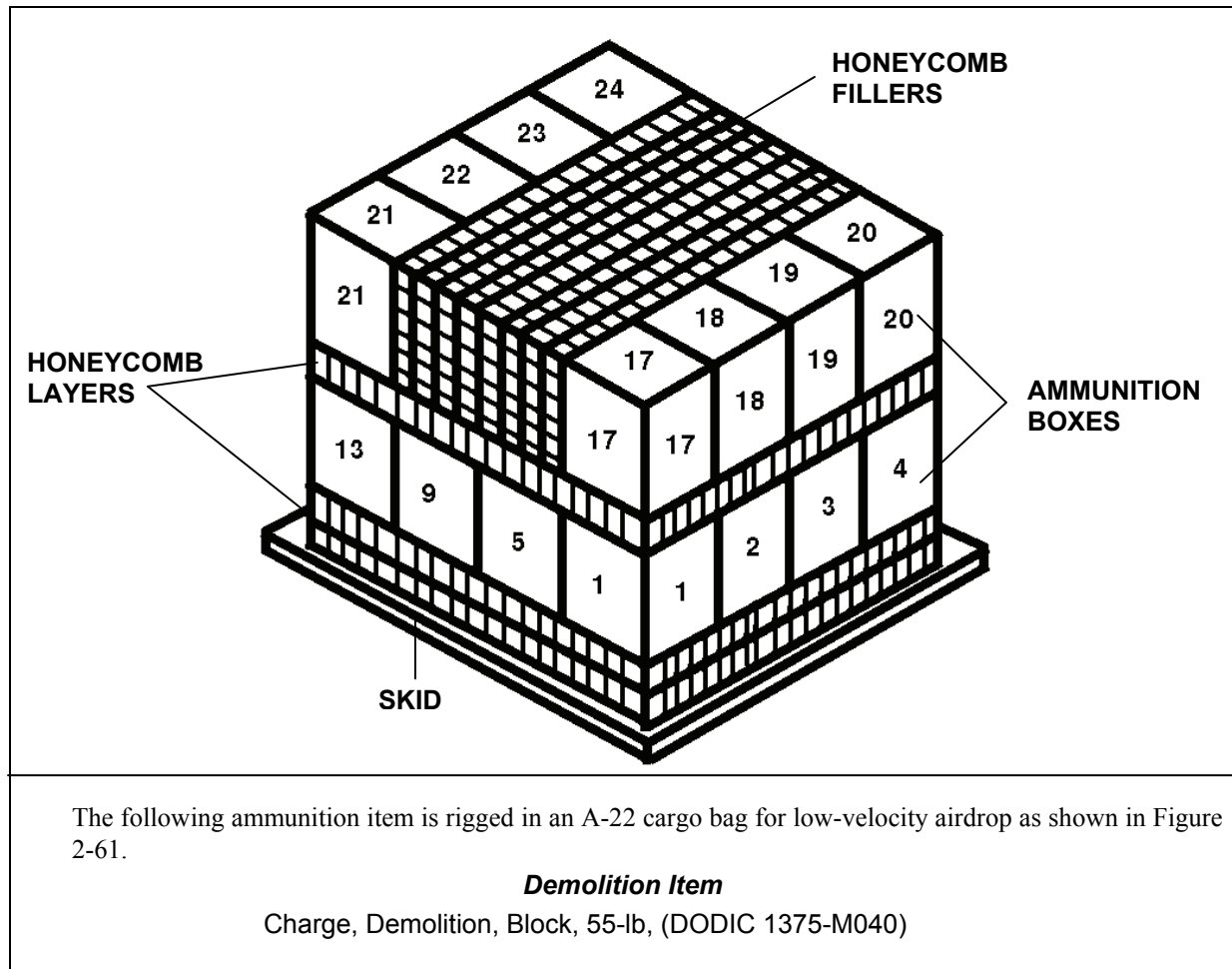
Figure 2-61. Ammunition Layout in an A-22 Cargo Bag for Low-Velocity Airdrop
