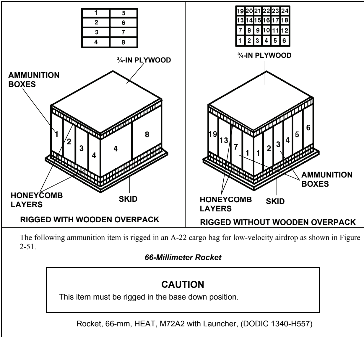
Figure 2-51. Ammunition Layout in an A-22 Cargo Bag for Low-Velocity Airdrop
