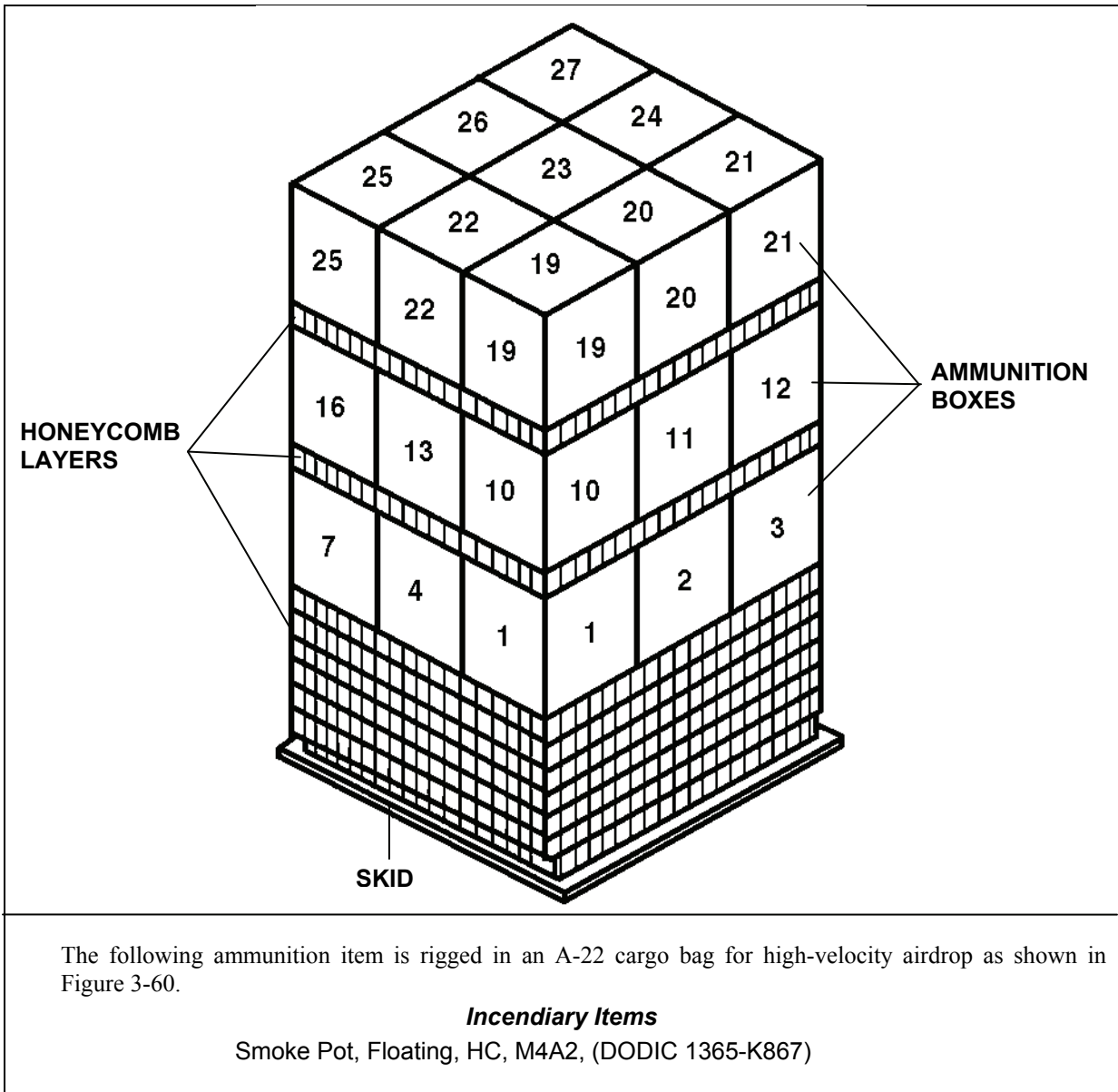
Figure 3-60. Ammunition Layout in an A-22 Cargo Bag for High-Velocity Airdrop
