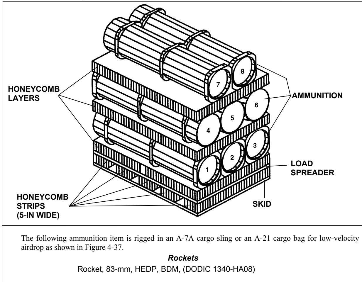
Figure 4-37. Ammunition Layout in an A-7A Cargo Sling or an A-21 Cargo Bag for Low-Velocity Airdrop
