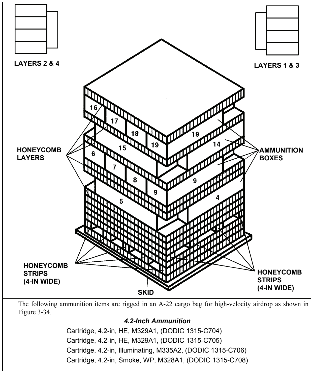
Figure 3-34. Ammunition Layout in an A-22 Cargo Bag for High-Velocity Airdrop
