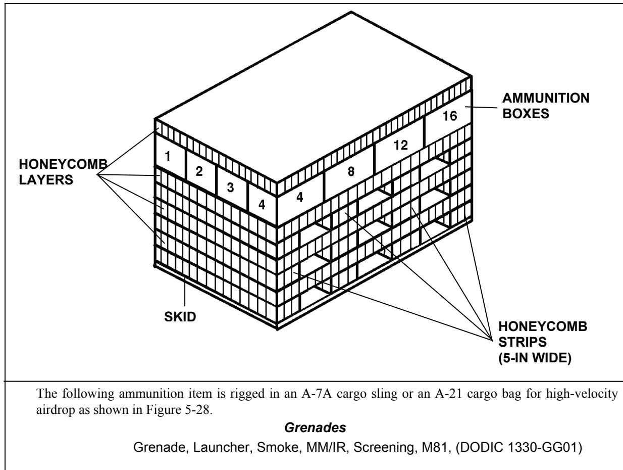
Figure 5-28. Ammunition Layout in an A-7A Cargo Sling or an A-21 Cargo Bag for High-Velocity Airdrop
