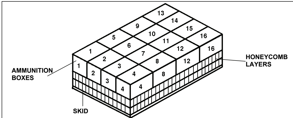
Figure 4-24. Ammunition Layout in an A-7A Cargo Sling or an A-21 Cargo Bag for Low-Velocity Airdrop
