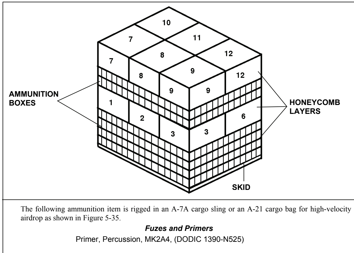
Figure 5-35. Ammunition Layout in an A-7A Cargo Sling or an A-21 Cargo Bag for High-Velocity Airdrop
