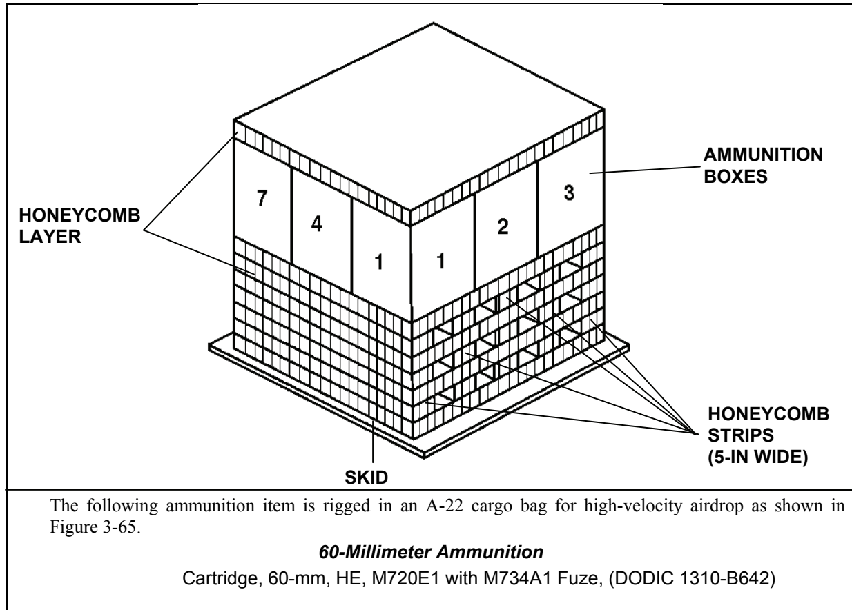
Figure 3-65. Ammunition Layout in an A-22 Cargo Bag for High-Velocity Airdrop
