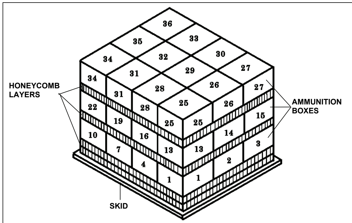
Figure 2-9. Ammunition Layout in an A-22 Cargo Bag for Low-Velocity Airdrop (continued)
