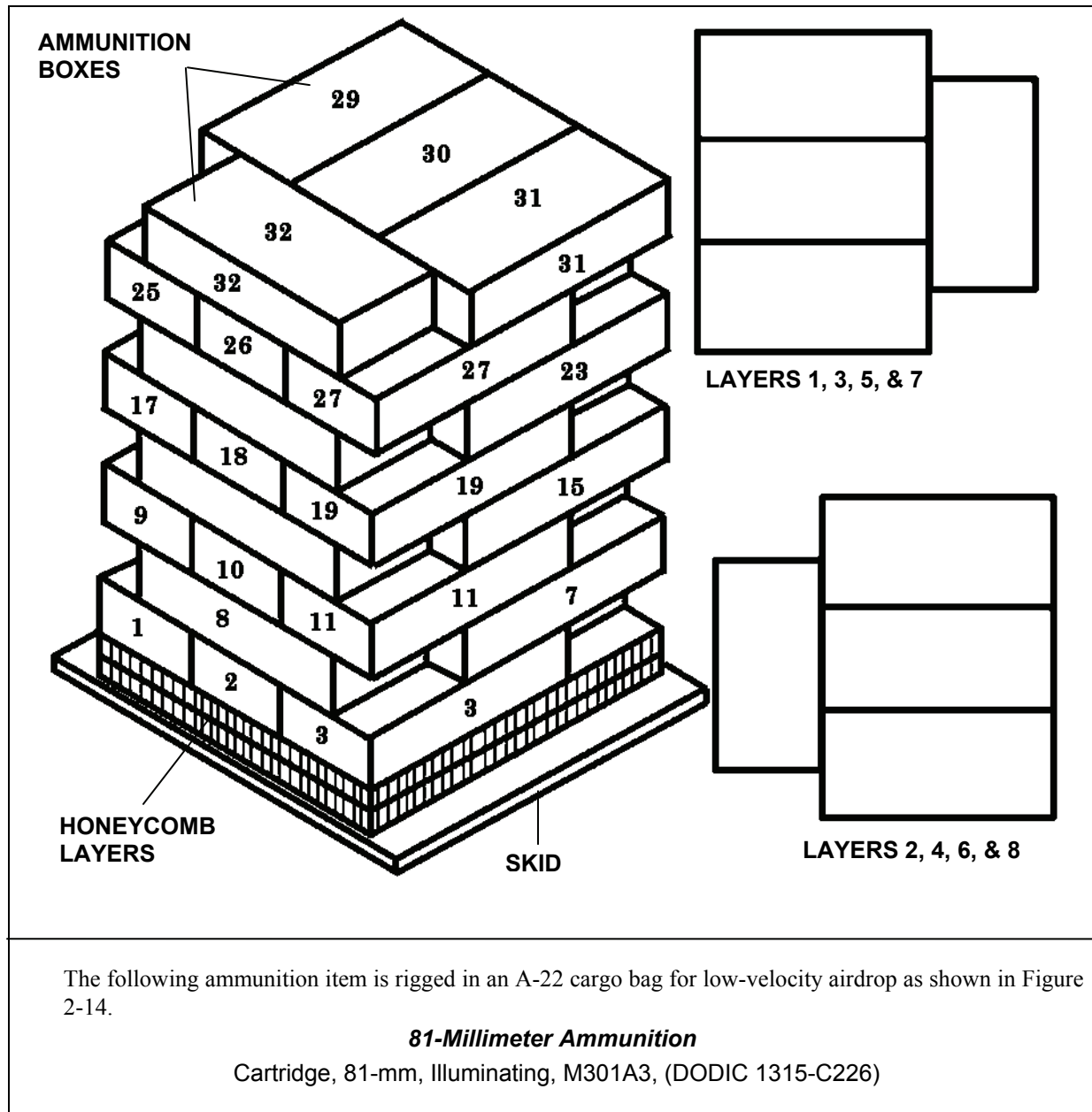
Figure 2-14. Ammunition Layout in an A-22 Cargo Bag for Low-Velocity Airdrop
