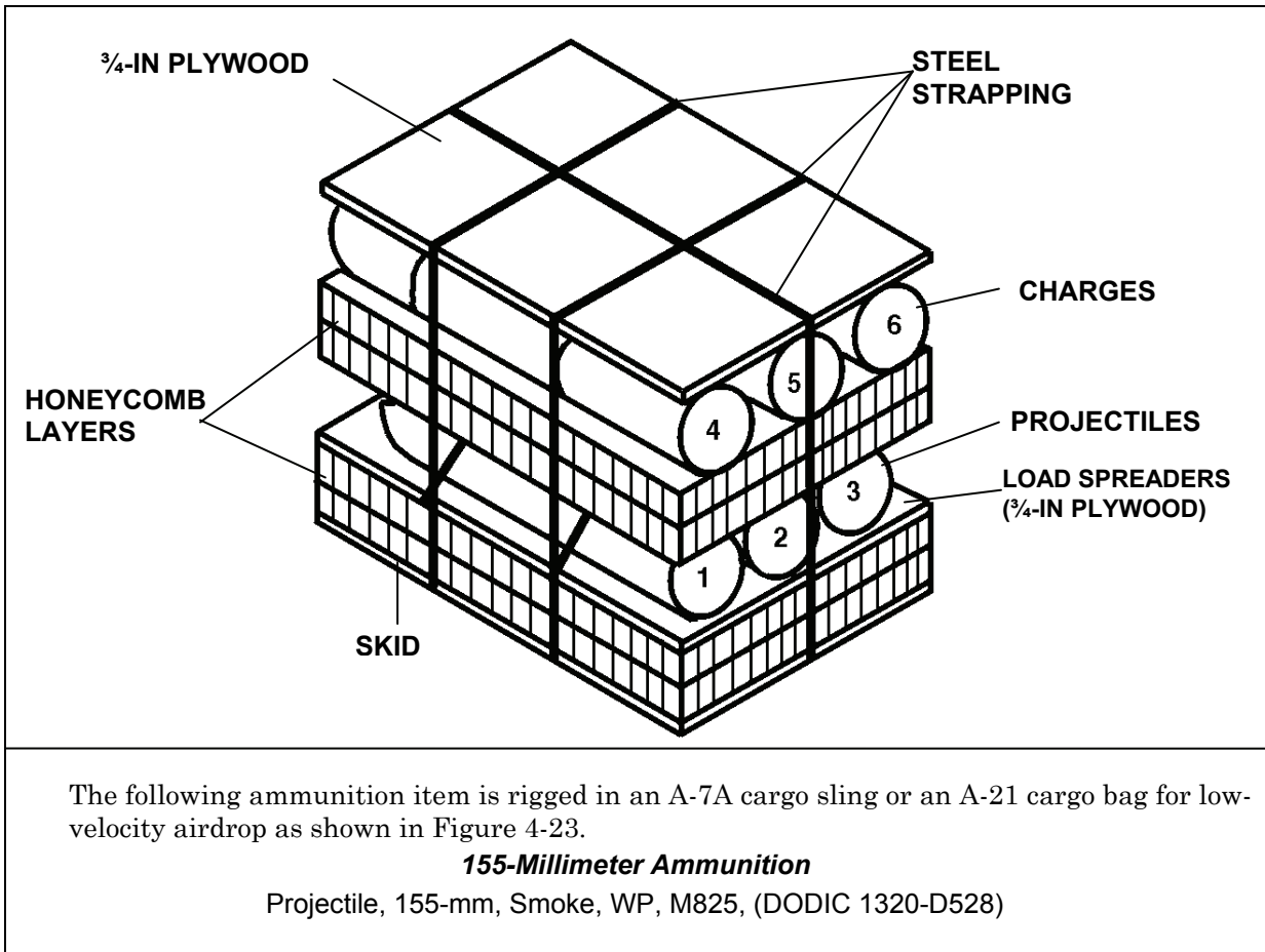
Figure 4-22. Ammunition Layout in an A-7A Cargo Sling or an A-21 Cargo Bag for Low-Velocity Airdrop
