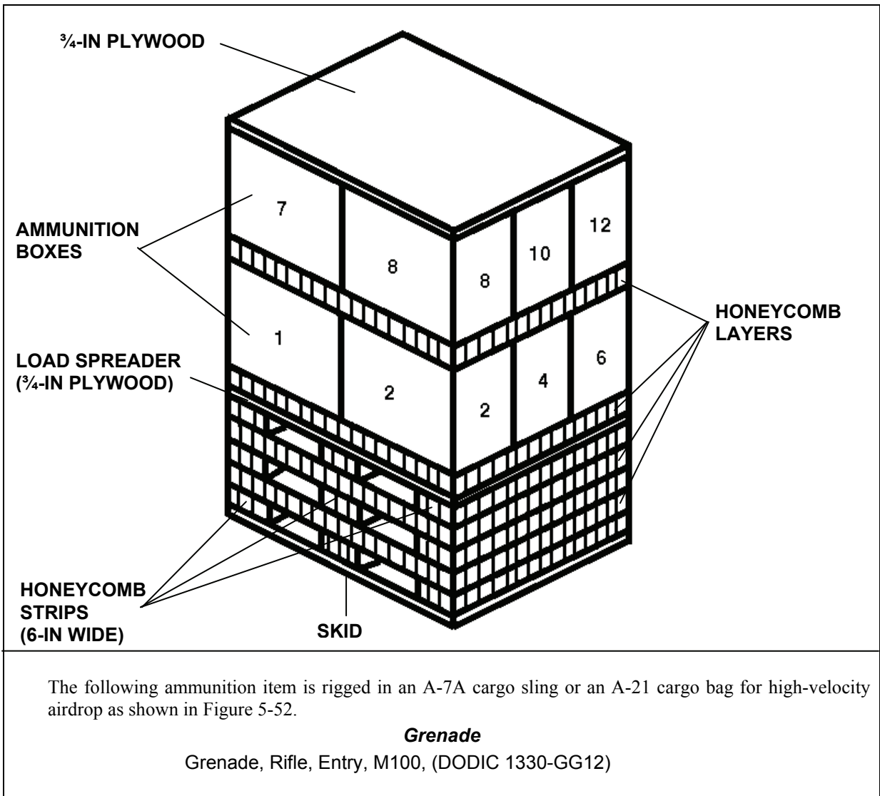
Figure 5-52. Ammunition Layout in an A-7A Cargo Sling or an A-21 Cargo Bag for High-Velocity Airdrop
