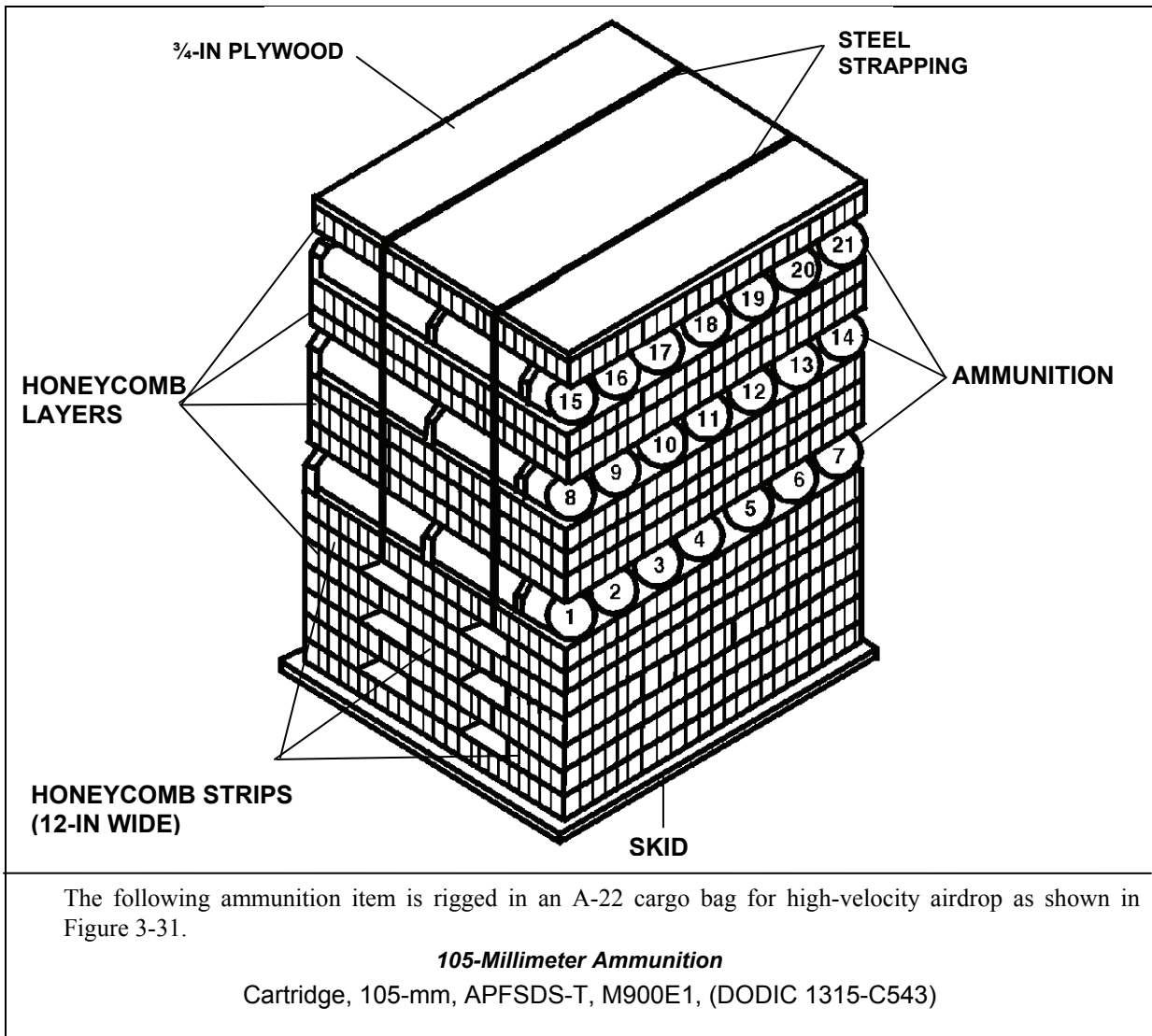
Figure 3-31. Ammunition Layout in an A-22 Cargo Bag for High-Velocity Airdrop
