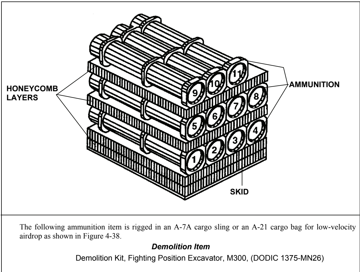
Figure 4-38. Ammunition Layout in an A-7A Cargo Sling or an A-21 Cargo Bag for Low-Velocity Airdrop
