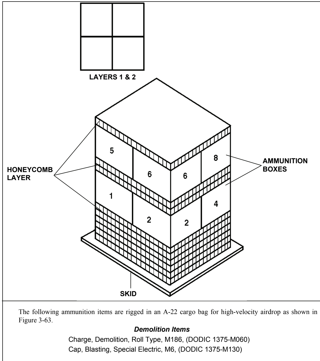
Figure 3-63. Ammunition Layout in an A-22 Cargo Bag for High-Velocity Airdrop
