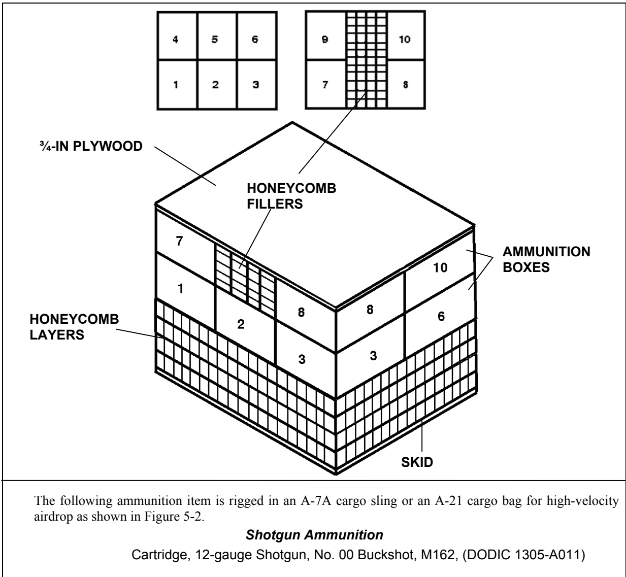
Figure 5-2. Ammunition Layout in an A-7A Cargo Sling or an A-21 Cargo Bag for High-Velocity Airdrop
