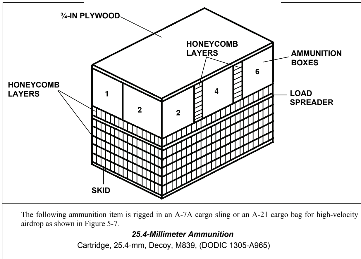
Figure 5-7. Ammunition Layout in an A-7A Cargo Sling or an A-21 Cargo Bag for High-Velocity Airdrop
