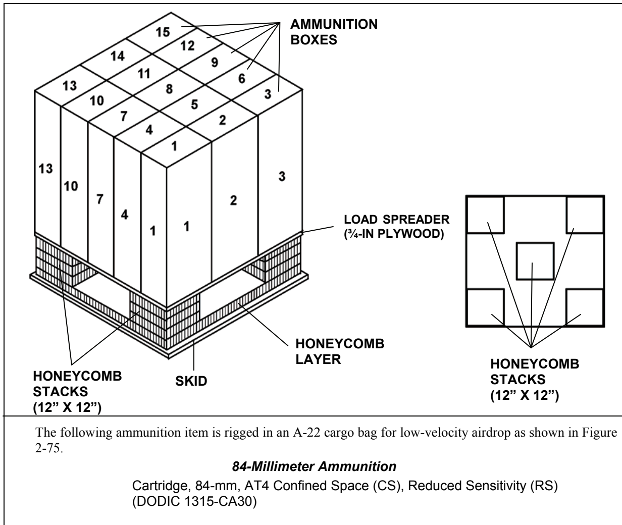
Figure 2-754. Ammunition Layout in an A-22 Cargo Bag for Low-Velocity Airdrop
