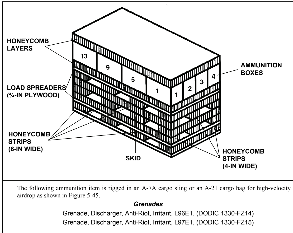
Figure 5-45. Ammunition Layout in an A-7A Cargo Sling or an A-21 Cargo Bag for High-Velocity Airdrop
