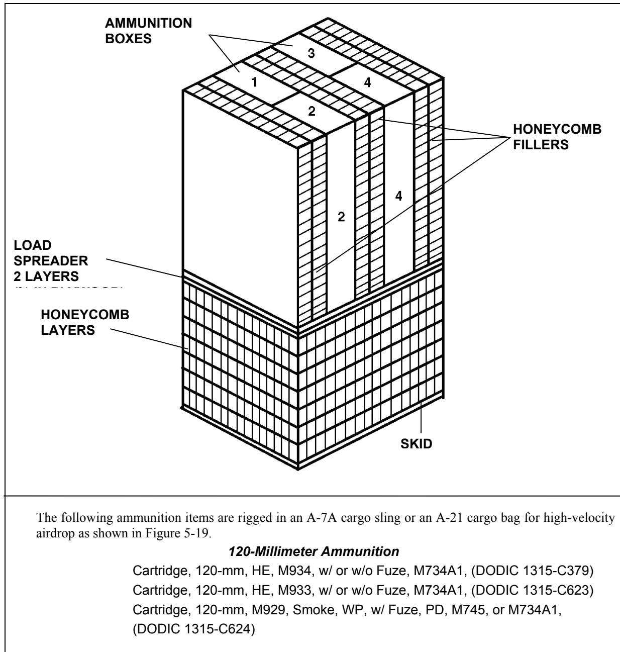
Figure 5-19. Ammunition Layout in an A-7A Cargo Sling or an A-21 Cargo Bag for High-Velocity Airdrop
