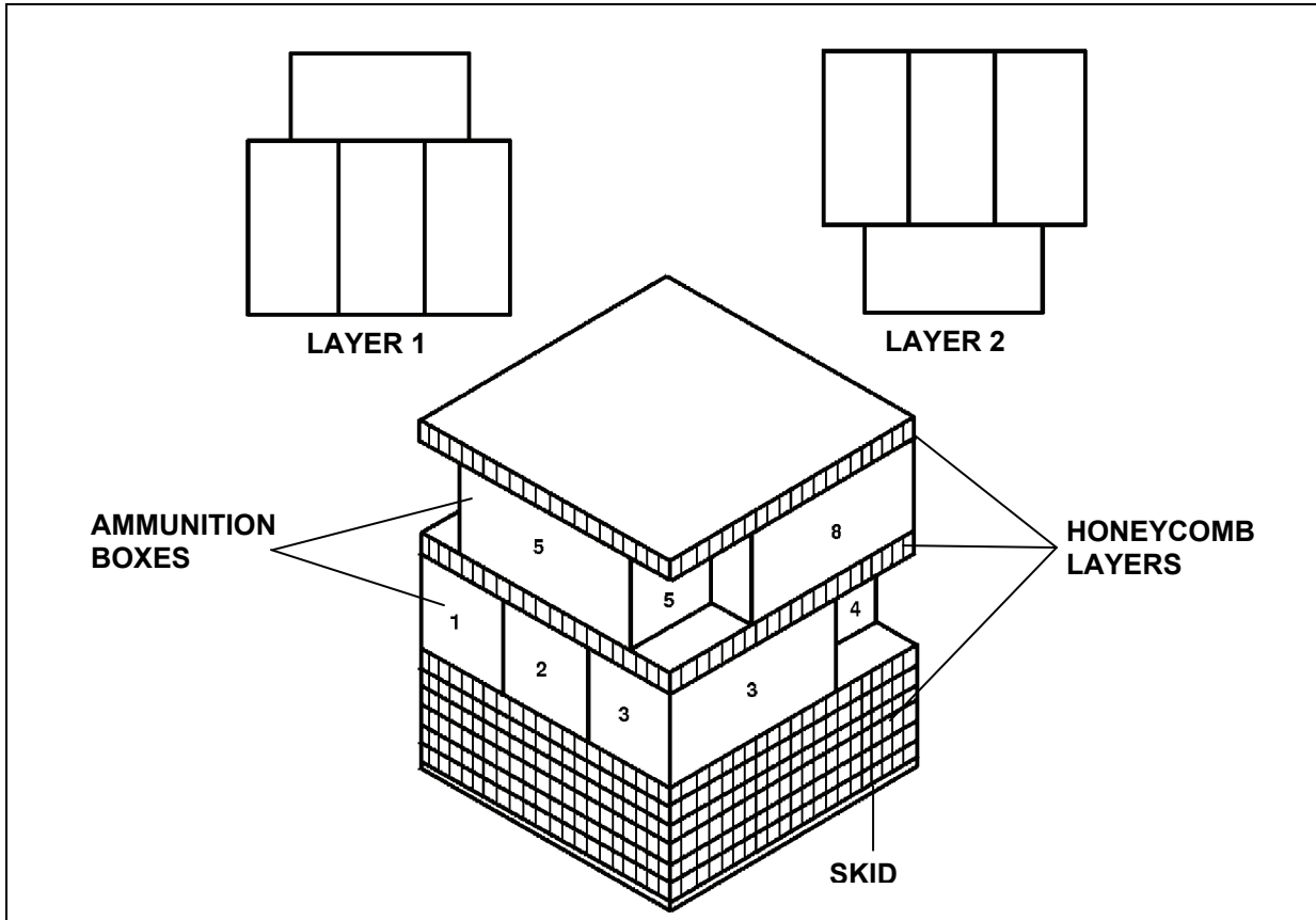
Figure 5-33. Ammunition Layout in an A-7A Cargo Sling or an A-21 Cargo Bag for High-Velocity Airdrop (continued)
