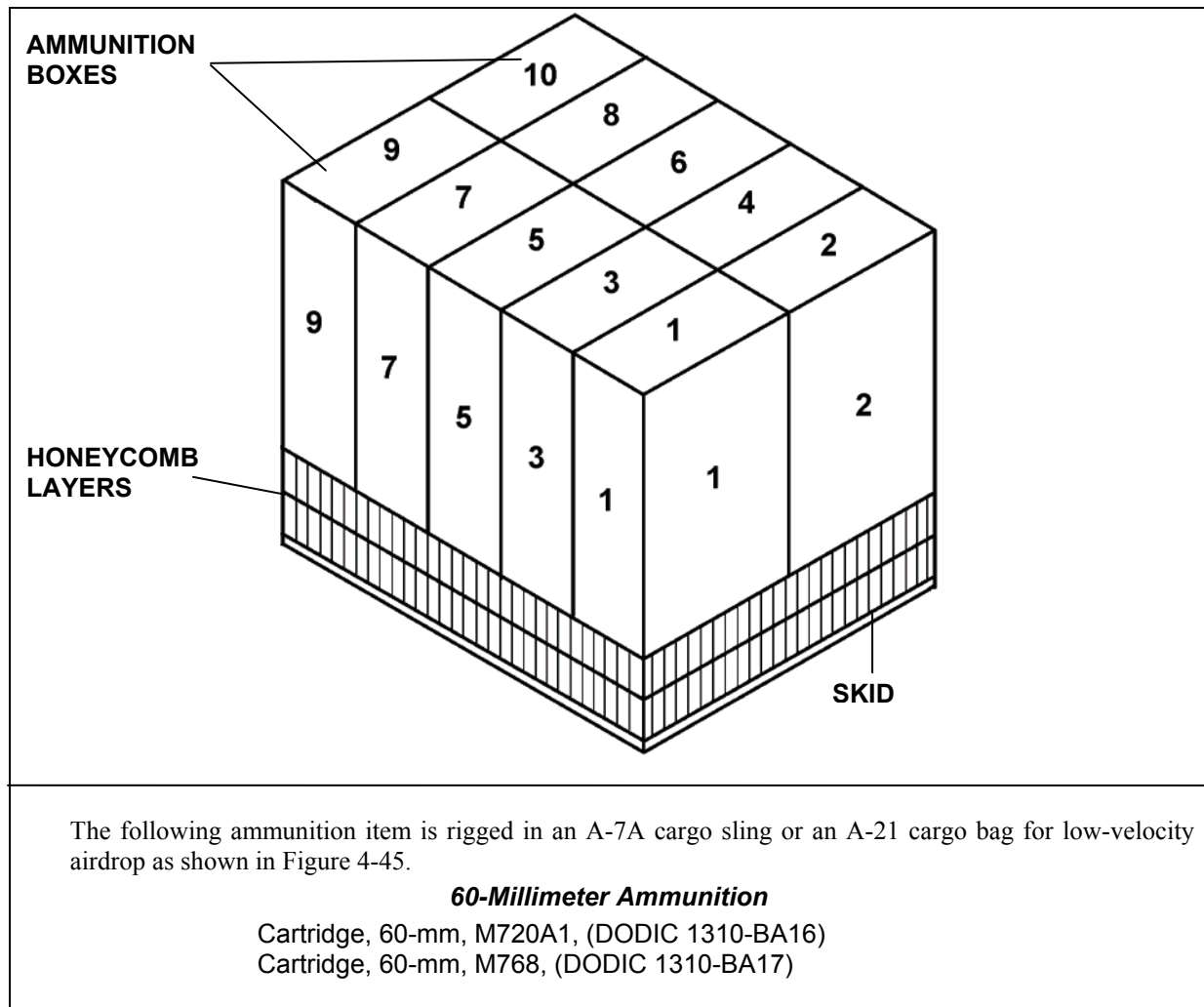
Figure 4-45. Ammunition Layout in an A-7A Cargo Sling or an A-21 Cargo Bag for Low-Velocity Airdrop
