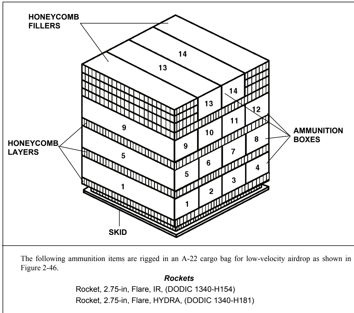
Figure 2-46. Ammunition Layout in an A-22 Cargo Bag for Low-Velocity Airdrop
