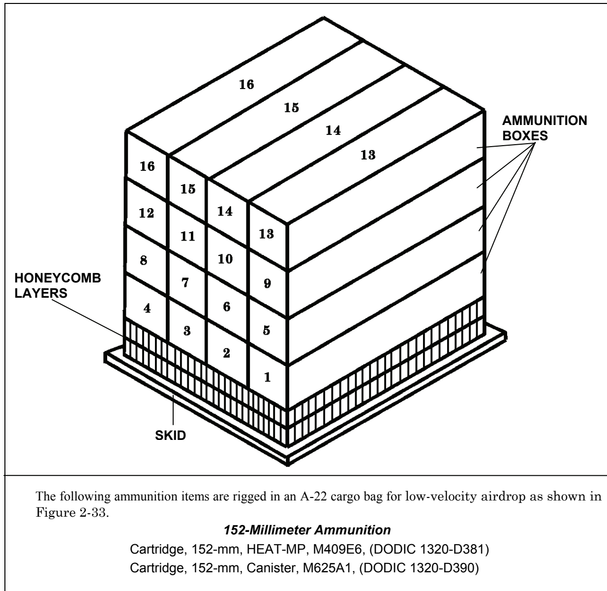
Figure 2-33. Ammunition Layout in an A-22 Cargo Bag for Low-Velocity Airdrop
