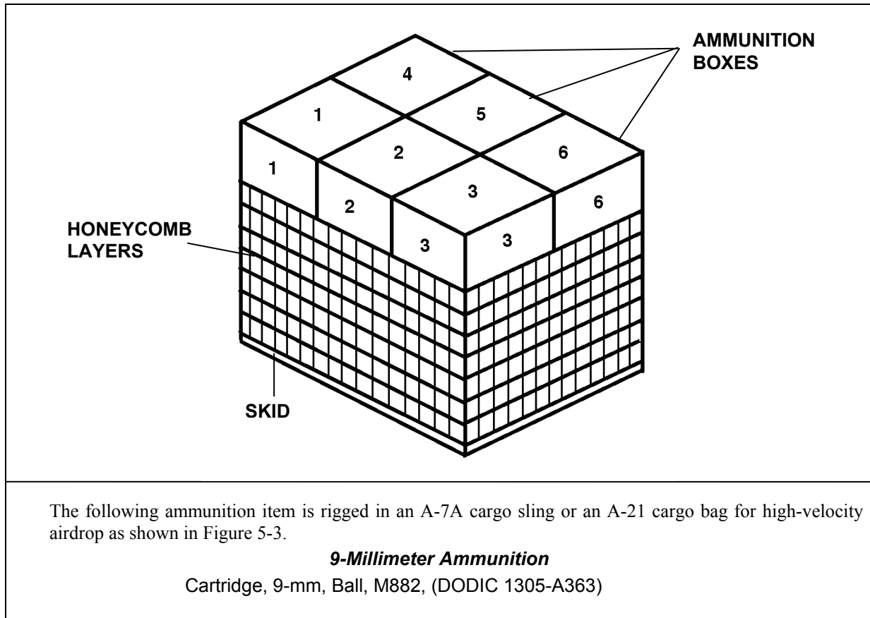
Figure 5-3. Ammunition Layout in an A-7A Cargo Sling or an A-21 Cargo Bag for High-Velocity Airdrop
