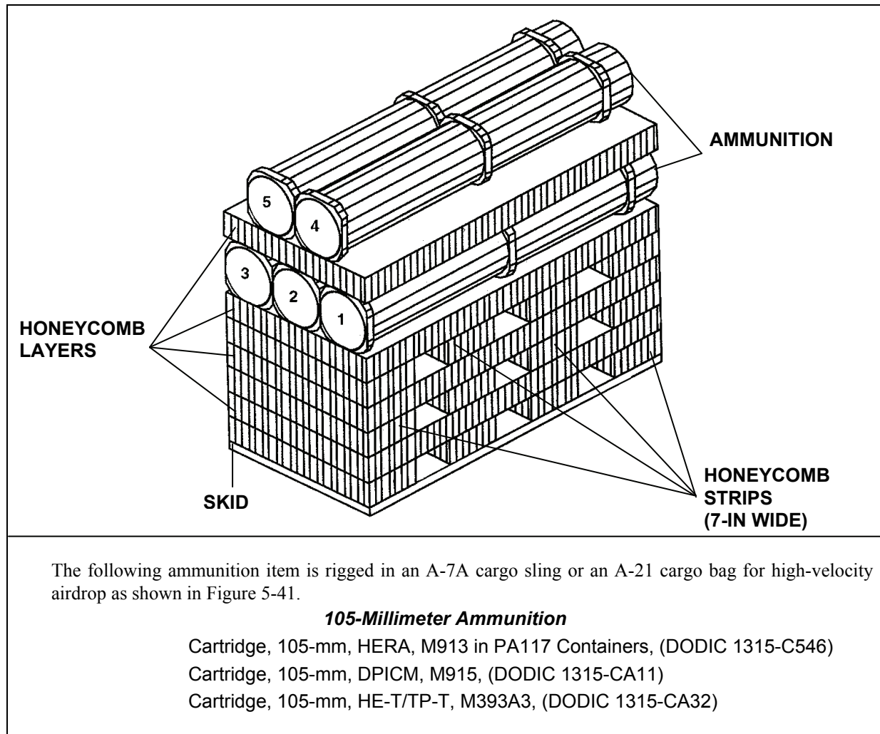
Figure 5-41. Ammunition Layout in an A-7A Cargo Sling or an A-21 Cargo Bag for High-Velocity Airdrop
