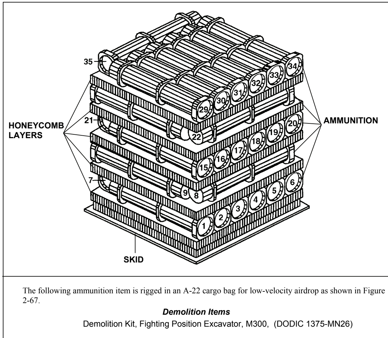
Figure 2-67. Ammunition Layout in an A-22 Cargo Bag for Low-Velocity Airdrop
