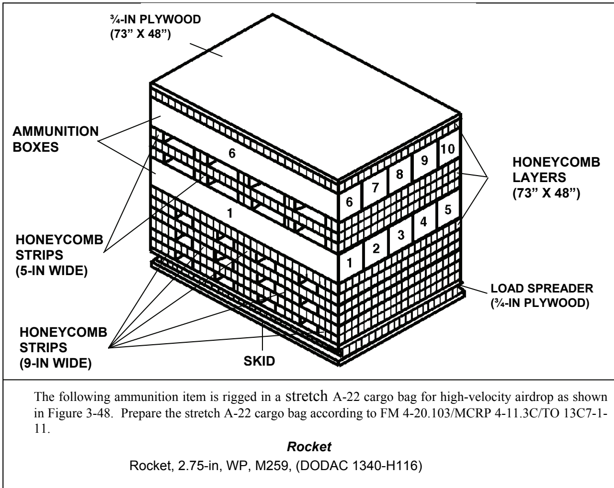
Figure 3-48. Ammunition Layout in a Stretch A-22 Cargo Bag for High-Velocity Airdrop
