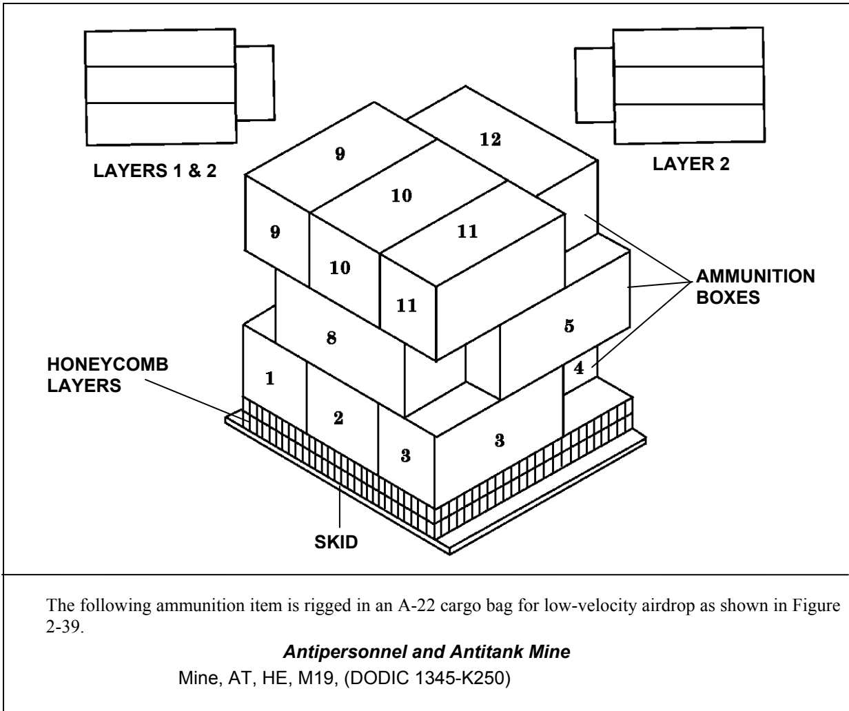
Figure 2-39. Ammunition Layout in an A-22 Cargo Bag for Low-Velocity Airdrop
