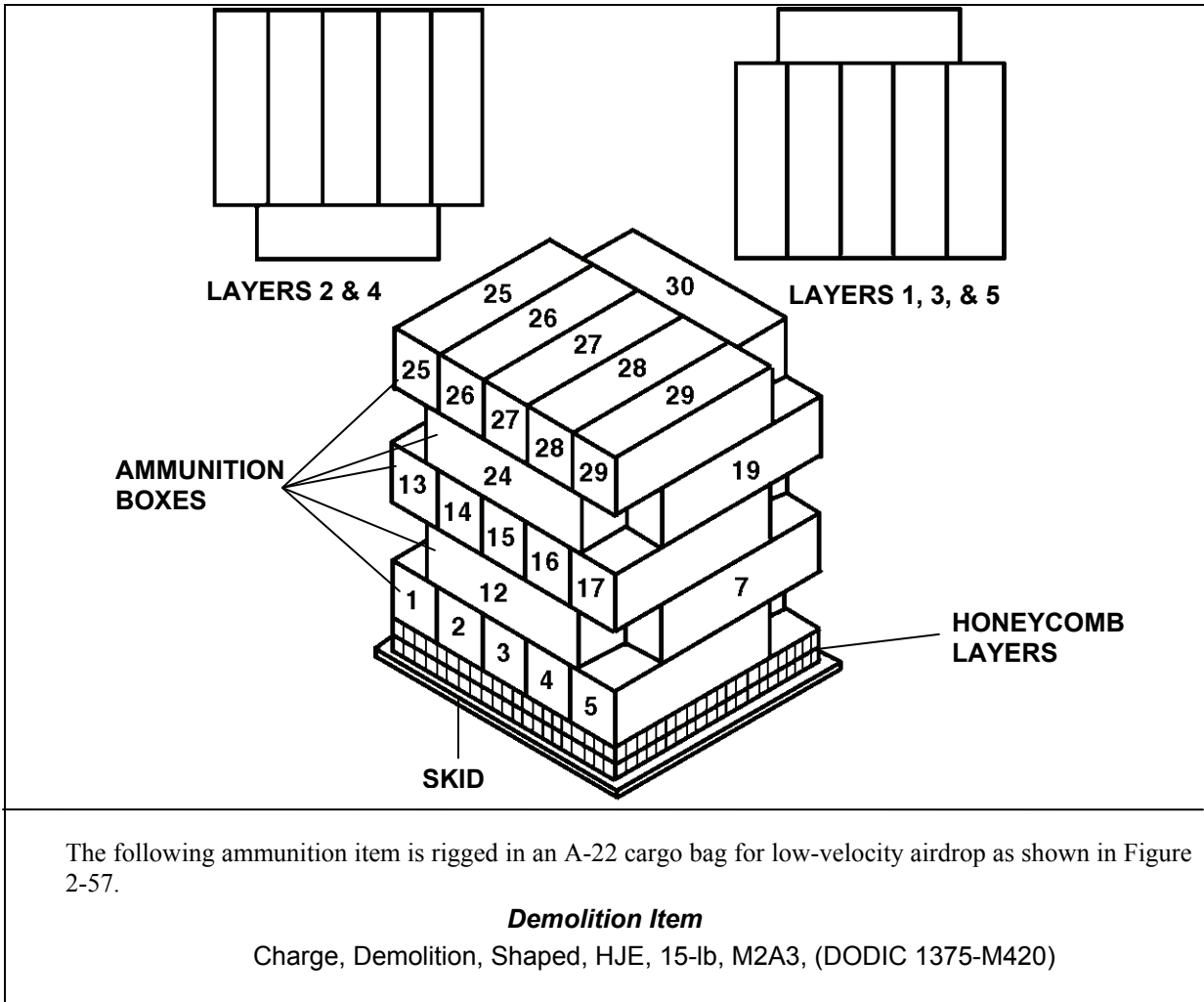
Figure 2-57. Ammunition Layout in an A-22 Cargo Bag for Low-Velocity Airdrop
