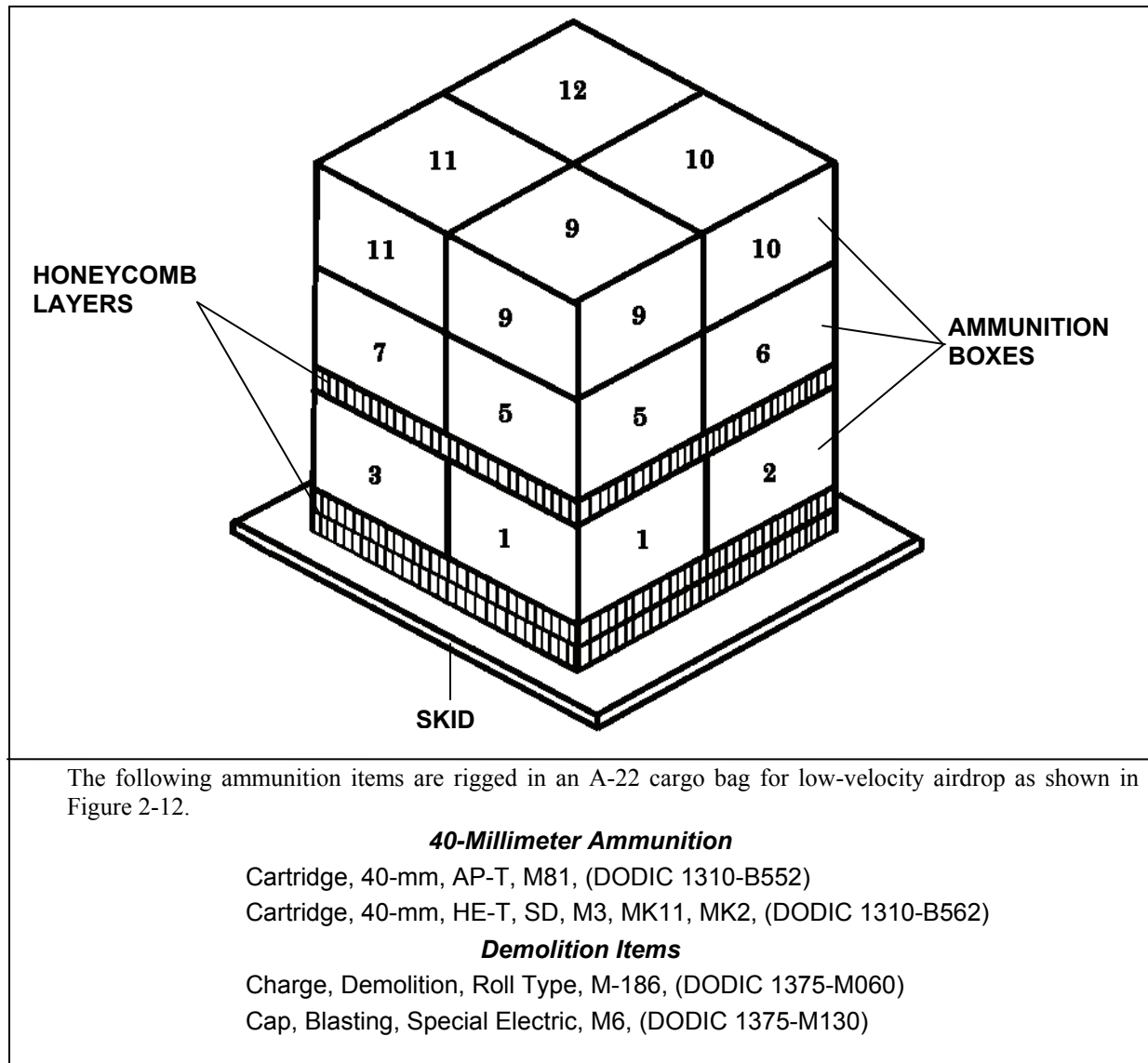
Figure 2-12. Ammunition Layout in an A-22 Cargo Bag for Low-Velocity Airdrop
