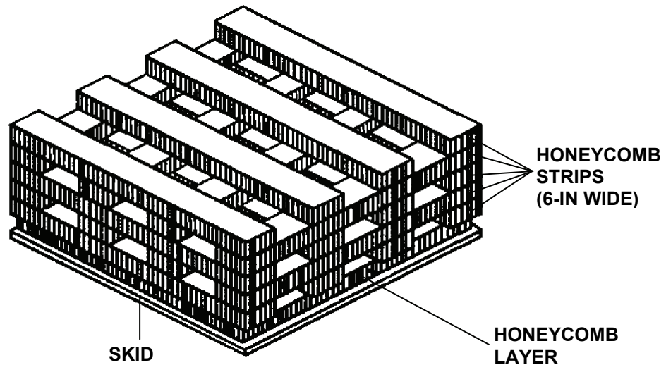
Figure 3-90. Honeycomb Stack and Rigging Steps for MDI Munitions in an A-22 Cargo Bag for High Velocity Airdrop
