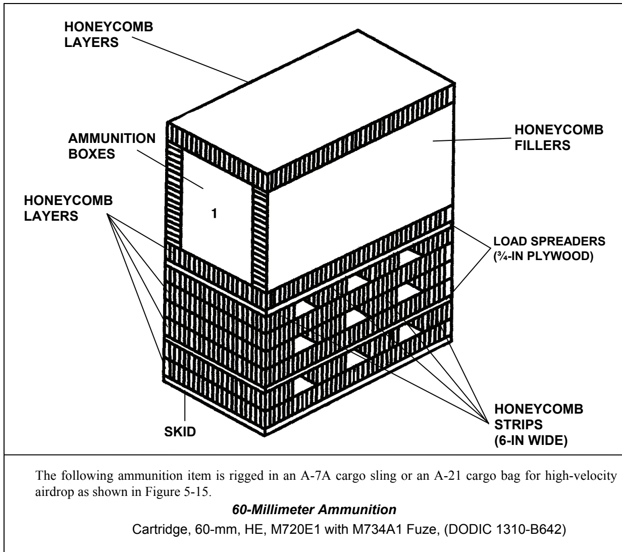
Figure 5-15. Ammunition Layout in an A-7A Cargo Sling or an A-21 Cargo Bag for High-Velocity Airdrop
