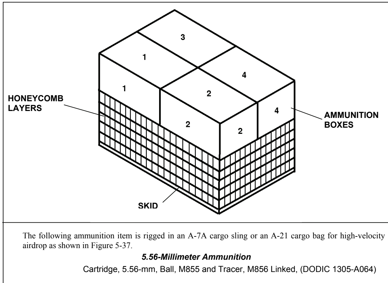
Figure 5-37. Ammunition Layout in an A-7A Cargo Sling or an A-21 Cargo Bag for High-Velocity Airdrop
