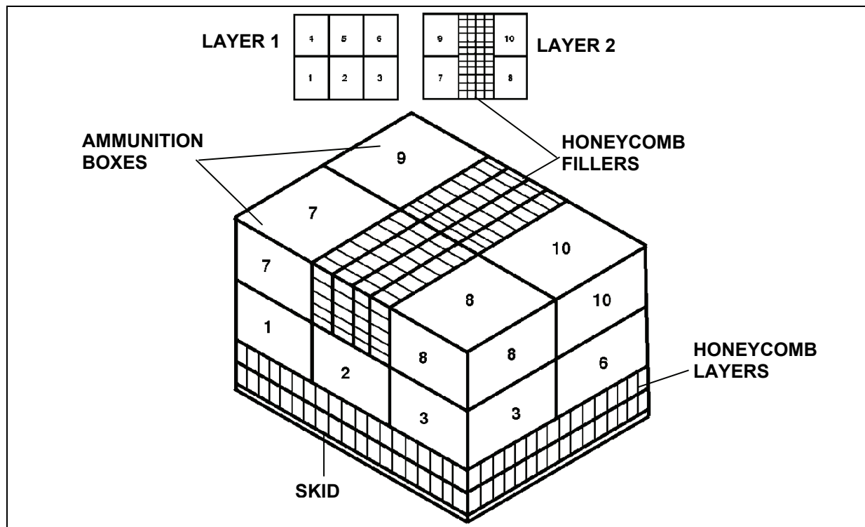
Figure 4-1. Ammunition Layout in an A-7A Cargo Sling or an A-21 Cargo Bag for Low-Velocity Airdrop (continued)
