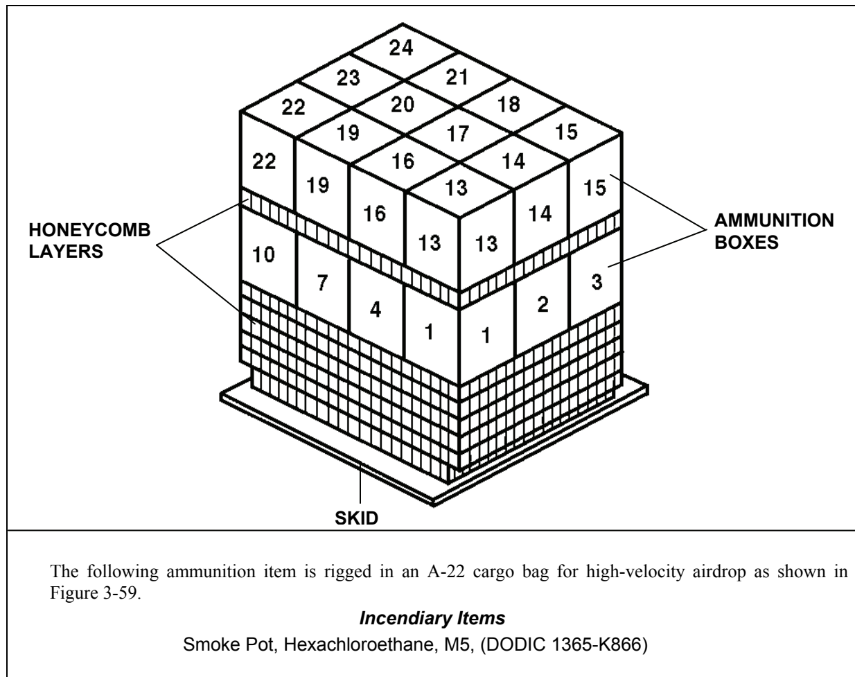
Figure 3-59. Ammunition Layout in an A-22 Cargo Bag for High-Velocity Airdrop
