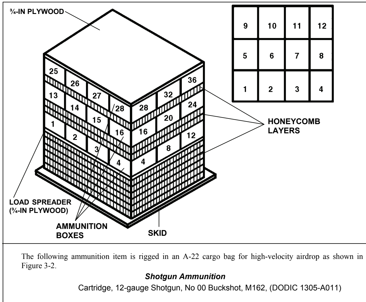
Figure 3-2. Ammunition Layout in an A-22 Cargo Bag for High-Velocity Airdrop
