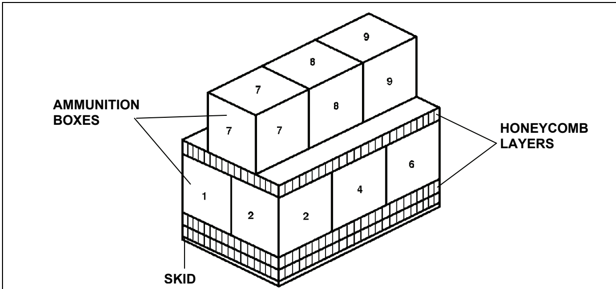
Figure 4-7. Ammunition Layout in an A-7A Cargo Sling or an A-21 Cargo Bag for Low-Velocity Airdrop (continued)
