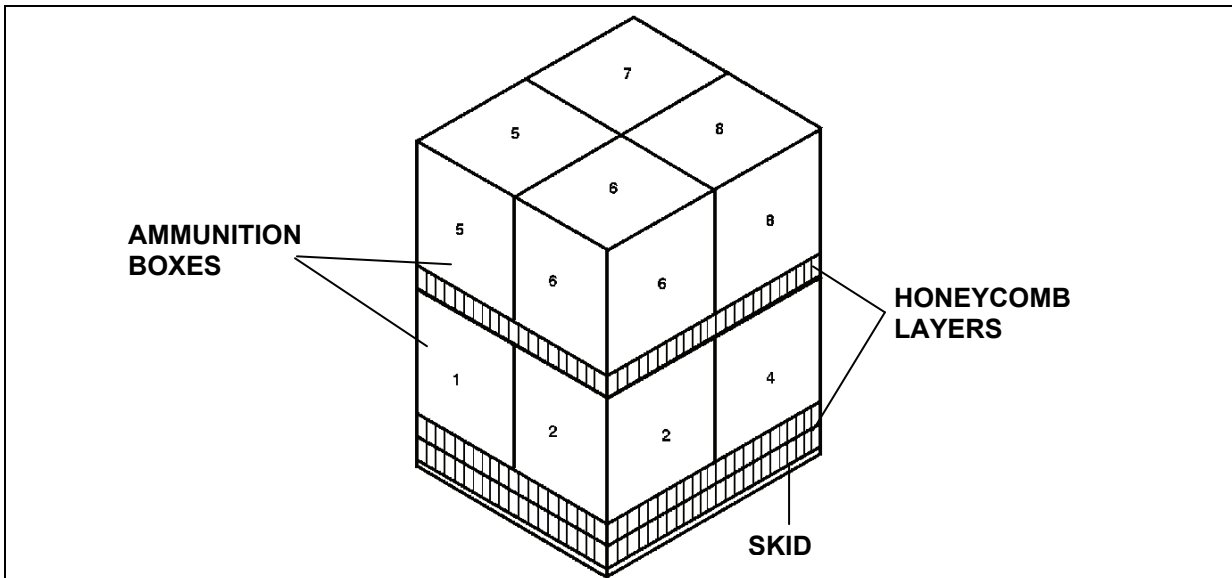
Figure 5-29. Ammunition Layout in an A-7A Cargo Sling or an A-21 Cargo Bag for High-Velocity Airdrop
