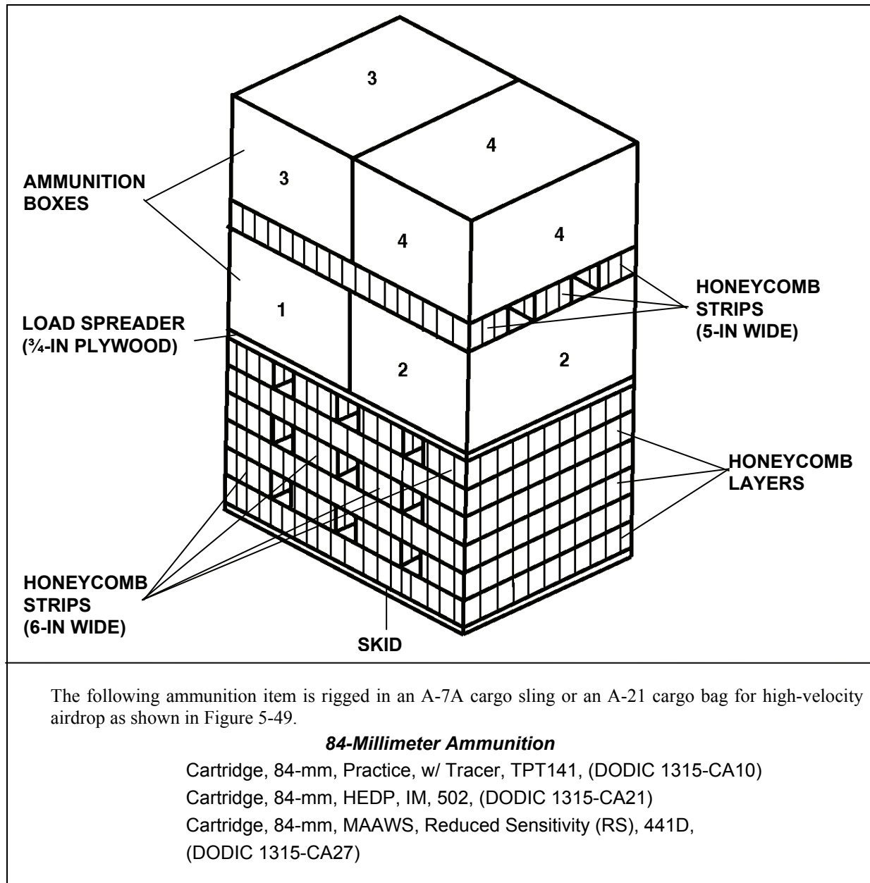
Figure 5-49. Ammunition Layout in an A-7A Cargo Sling or an A-21 Cargo Bag for High-Velocity Airdrop
