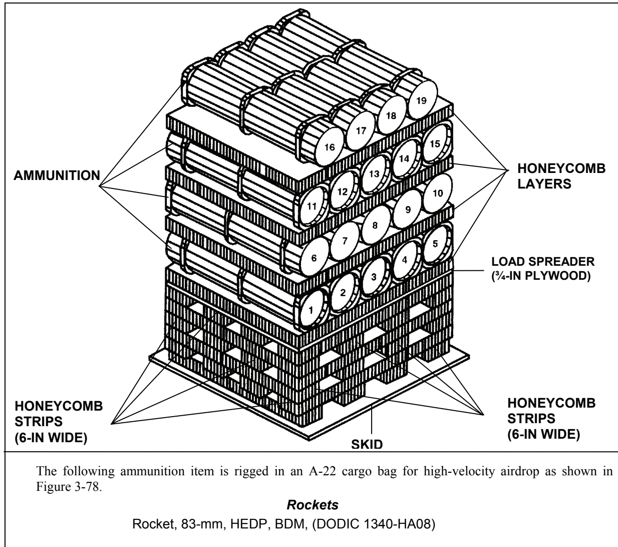
Figure 3-78. Ammunition Layout in an A-22 Cargo Bag for High-Velocity Airdrop
