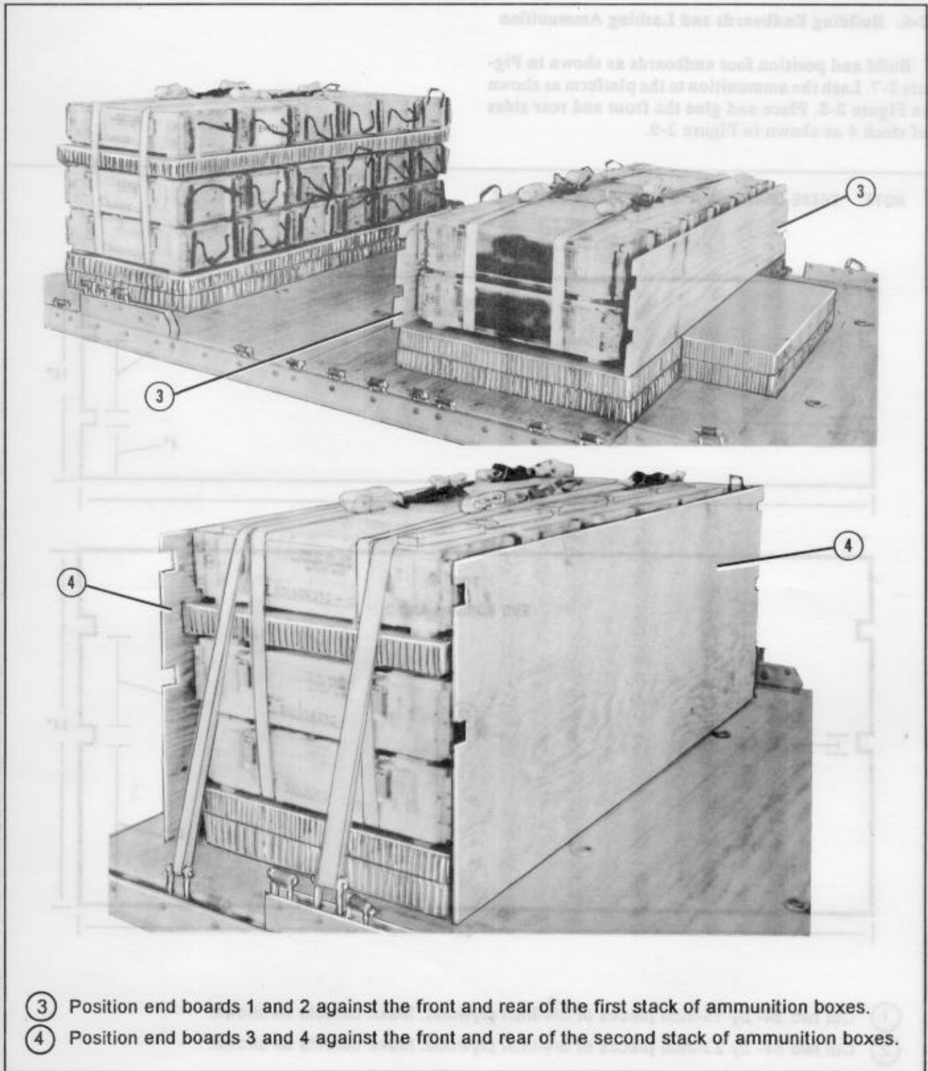
Figure 2-7. Endboards built and positioned (continued)
