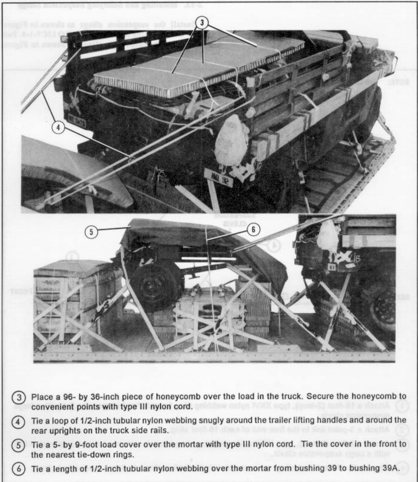
Figure 2-16. Honeycomb, cover, and ties installed (continued)
