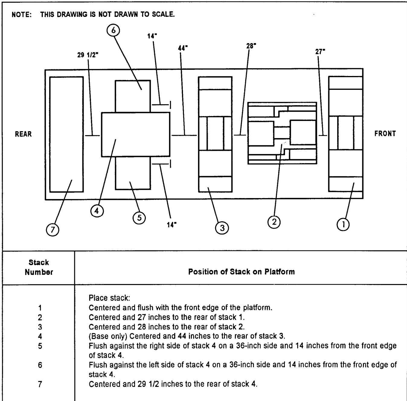
Figure 2-4. Honeycomb stacks placed on platform
