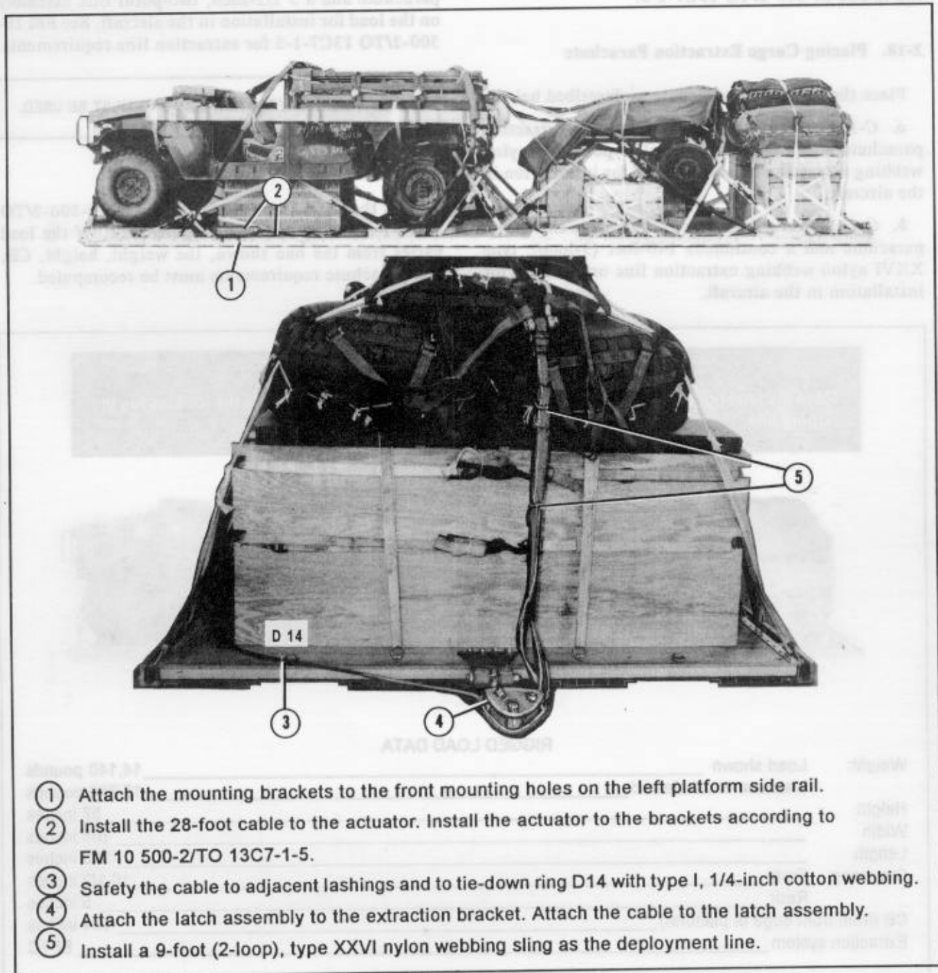
Figure 2-21. EFTC installed
