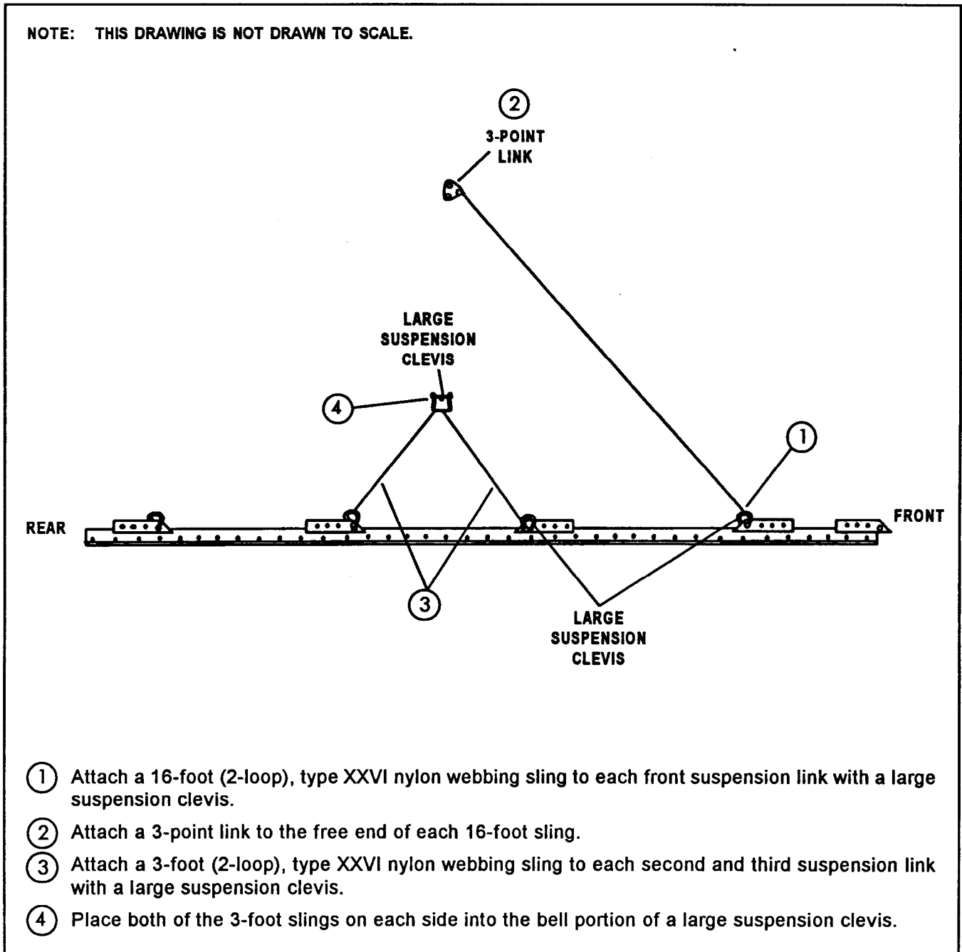
Figure 2-17. Suspension slings installed
