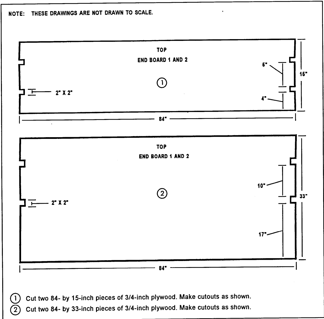
Figure 2-7. Endboards built and positioned
