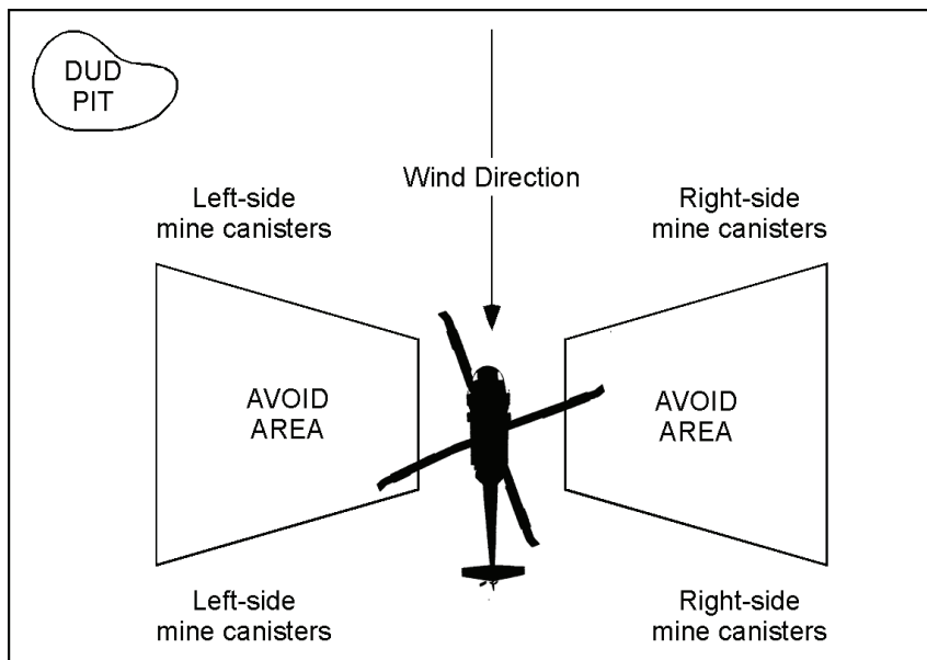
Figure 2-20. Example of a site layout for a Volcano arming point
