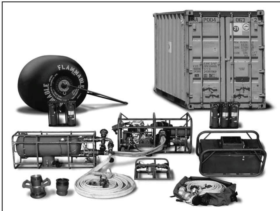
Figure 2-3. Advanced aviation forward area refueling system
