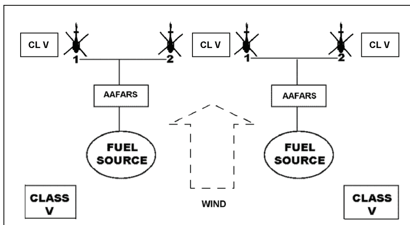
Figure 2-21. T-formation advanced aviation forward area refueling system setup
