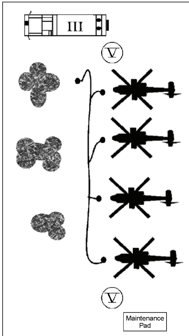
Figure 2-17. Simultaneous rearming and refueling forward arming and refueling point layout
