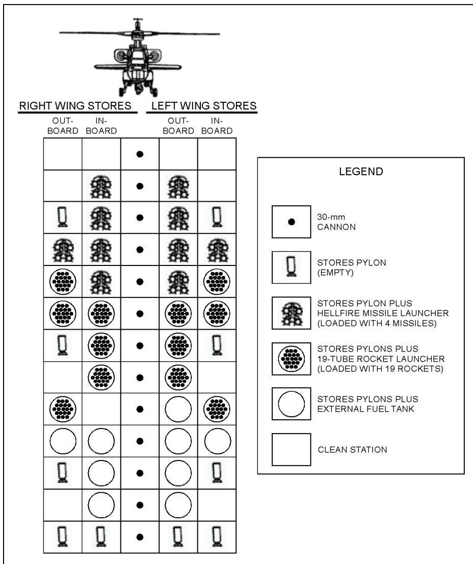
Figure 2-18. AH-64 armament configurations
