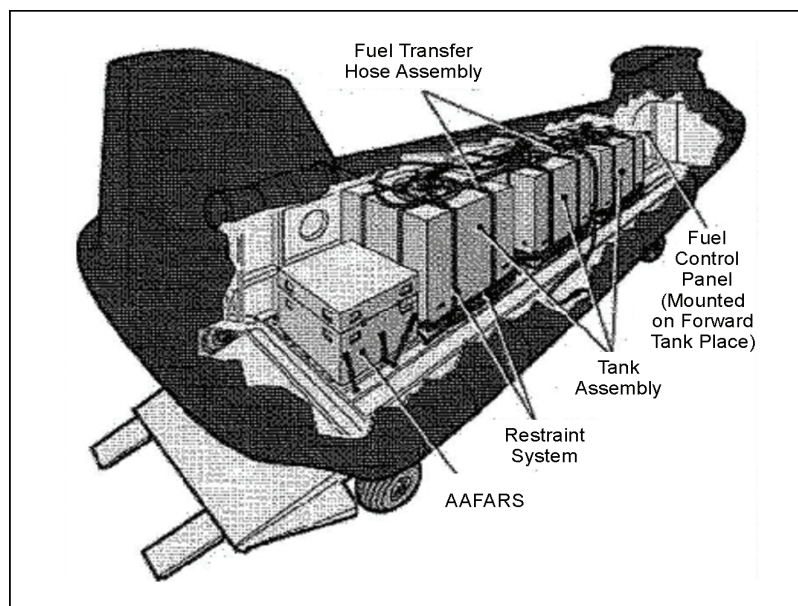
Figure 2-15. Extended range fuel system II functional components
