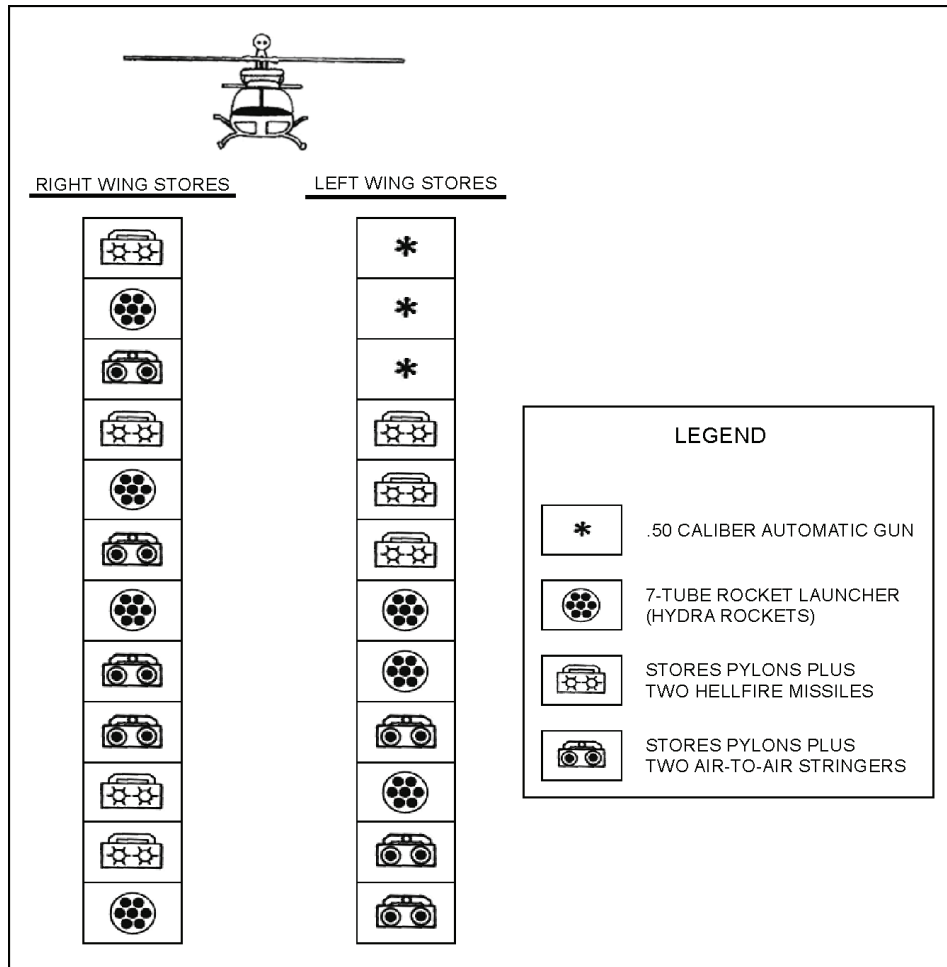
Figure 2-19. OH-58D authorized armament configurations
