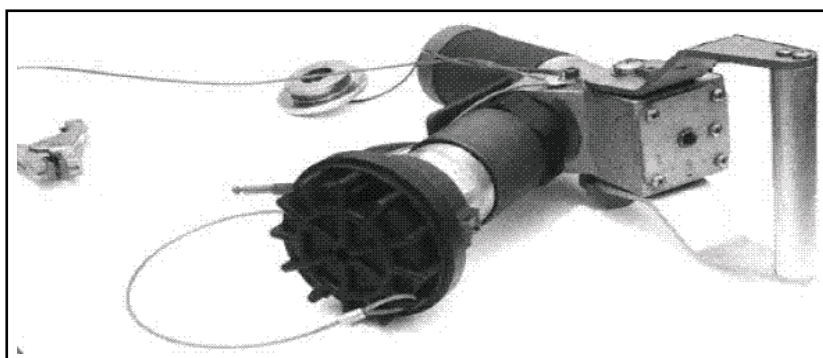
Figure 2-9. Model 125-1000 closed-circuit refueling nozzle
