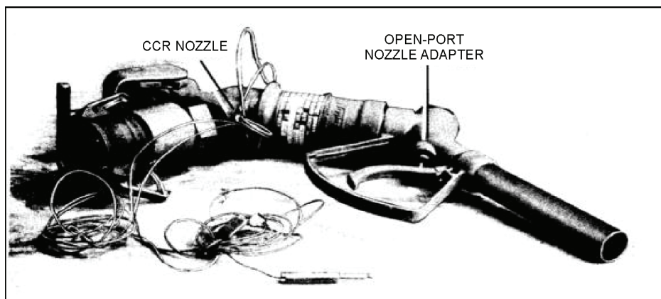
Figure 2-8. Open-port nozzle adapter
