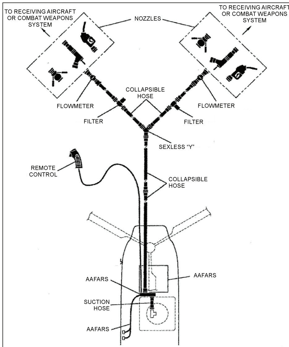
Figure 2-16. Typical layout for fat cow refueling points
