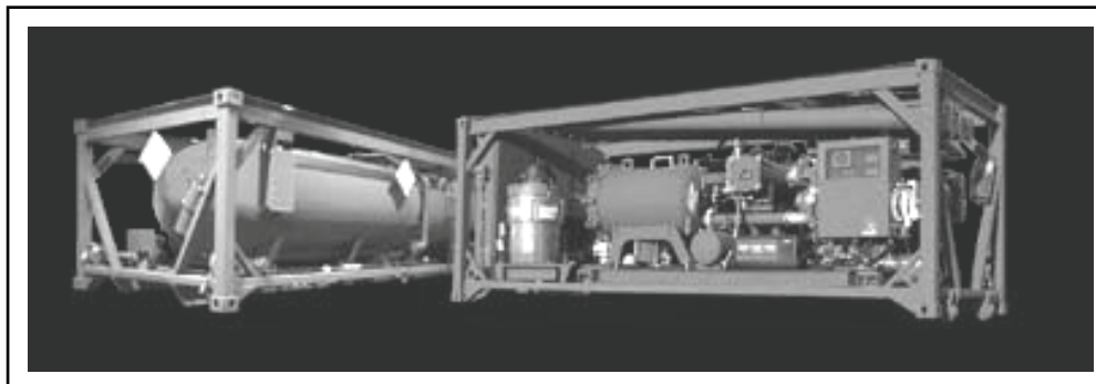
Figure 2-12. Modular fuel system
