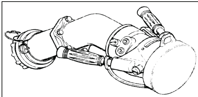
Figure 2-11. D-1 center point refueling nozzle
