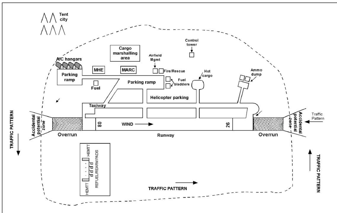
Figure 2-22. Notional long term forward arming and refueling point on an airfield
