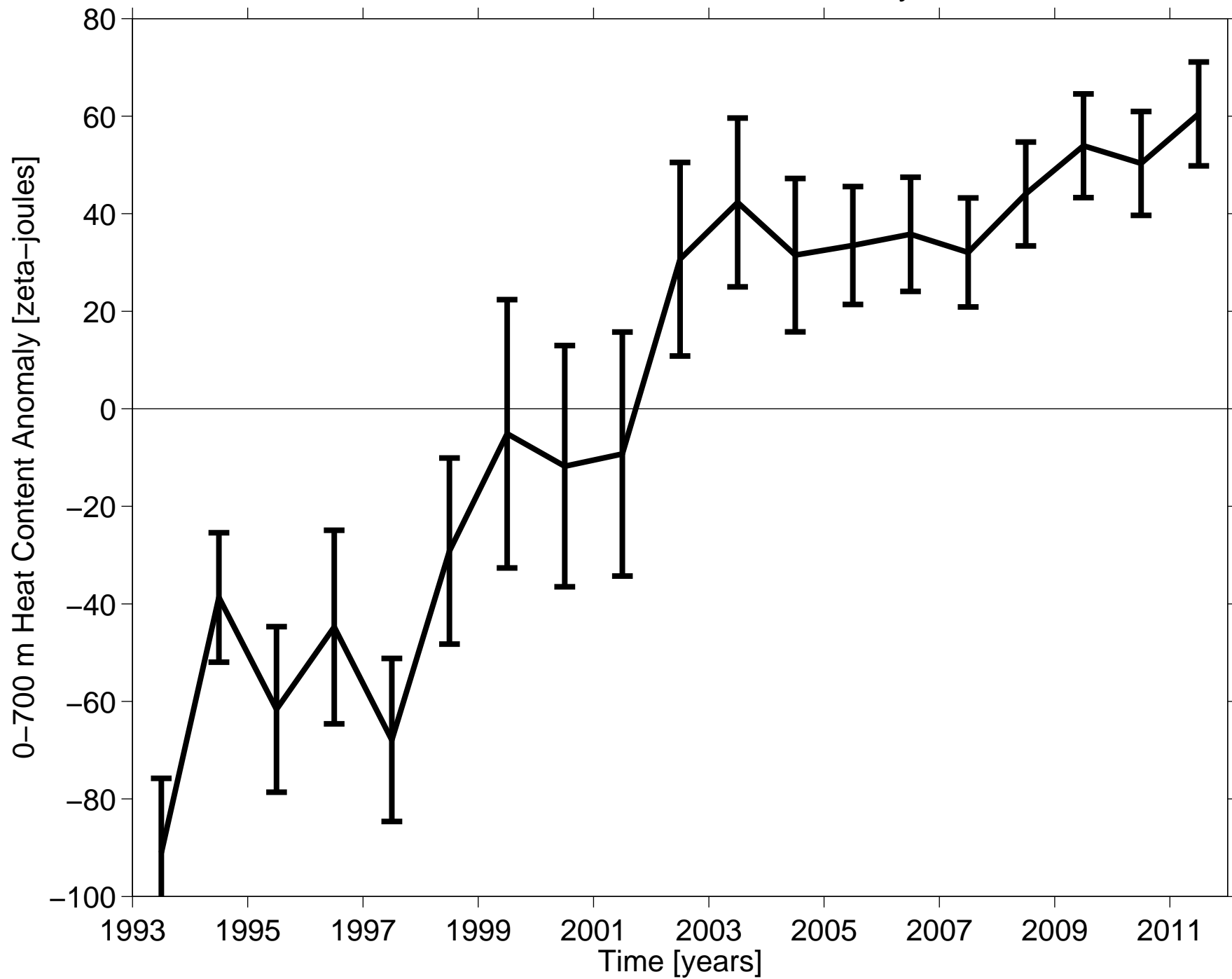
0-700m Heat Content Anomaly
