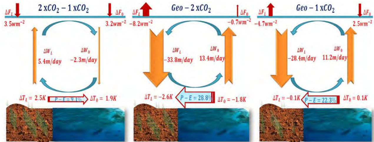
Figure A.4.1: Schematic diagram illustrating the changes in vertical motion at 500 mb over land and oceans when CO_2 is doubled (left panel, 2xCO_2-1xCO_2 ), albedo over land is enhanced (middle panel, enhanced albedo case: Geo- 2xCO_2 ) and when CO_2 is doubled and land albedo is enhanced (right panel, the geoengineered case: Geo- 1xCO_2 ) cases. Radiative forcings over land and oceans in each case are shown at the top. Vertical motion in height coordinates ( w , meter/day) is obtained from w = -\omega/(pg) where \omega is the model simulated pressure velocity. Changes in surface temperature and precipitation minus evaporation are also shown. Strong downward motion and the consequent decline in runoff and drying over land are indicated for the enhanced land albedo and geoengineering cases.
