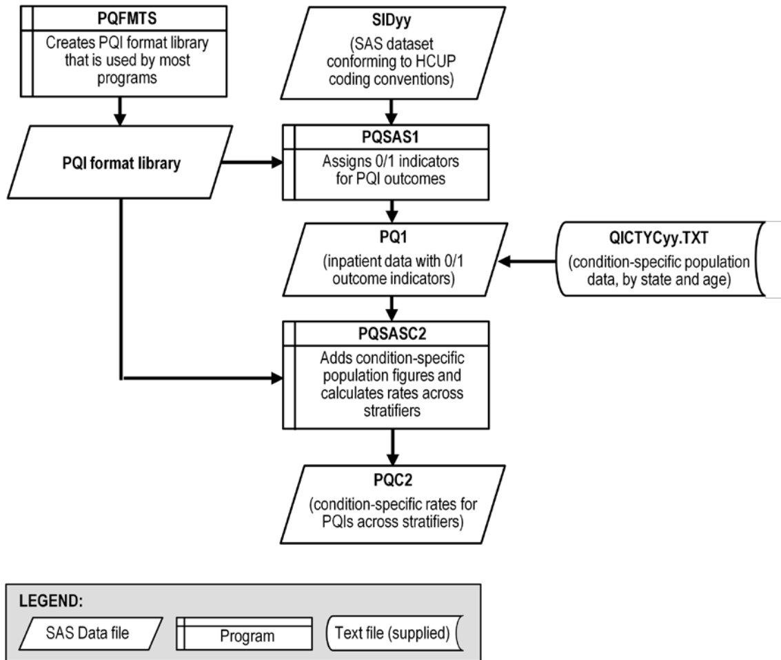
Figure 2. Processing steps for the PQI - Condition-specific
