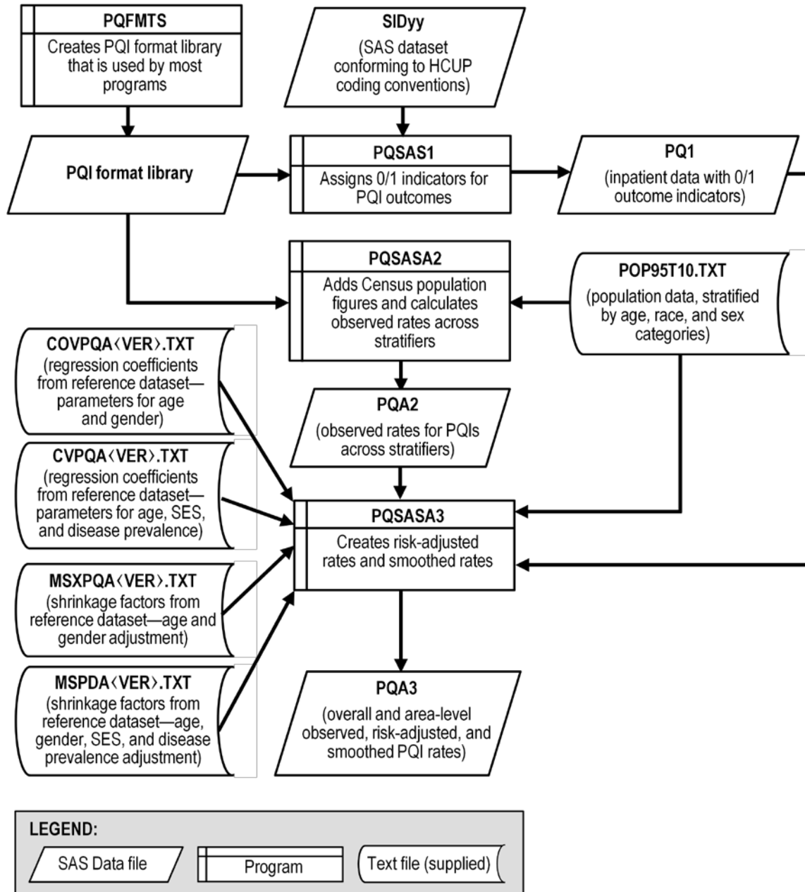
Figure 1. Processing steps for the PQI - Area
