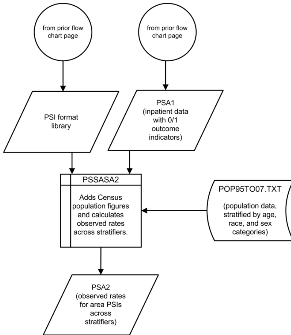
Figure 2. Processing Steps for the Patient Safety Indicators - Area
