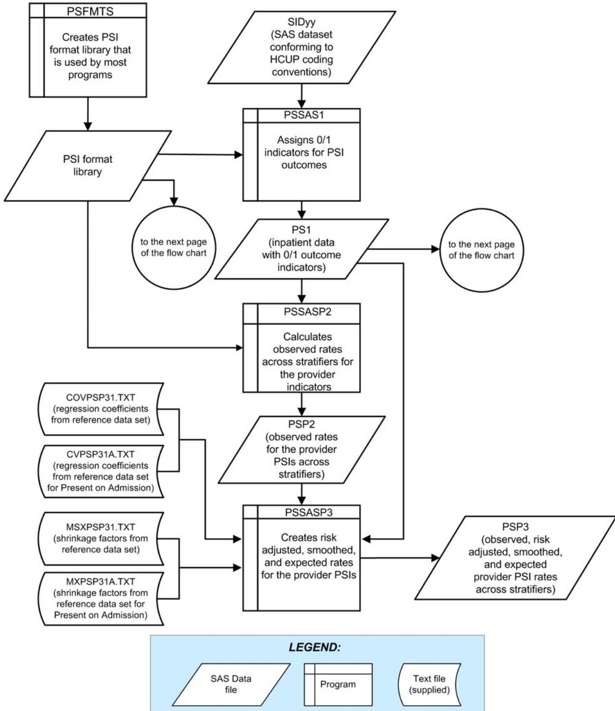
Figure 1. Processing Steps for the Patient Safety Indicators - Provider
