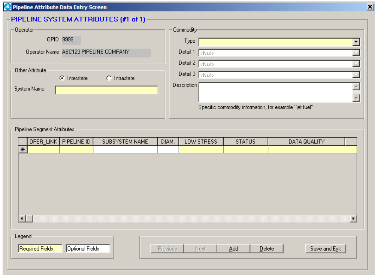
Figure 3-6. Pipeline attributes data entry screen.
