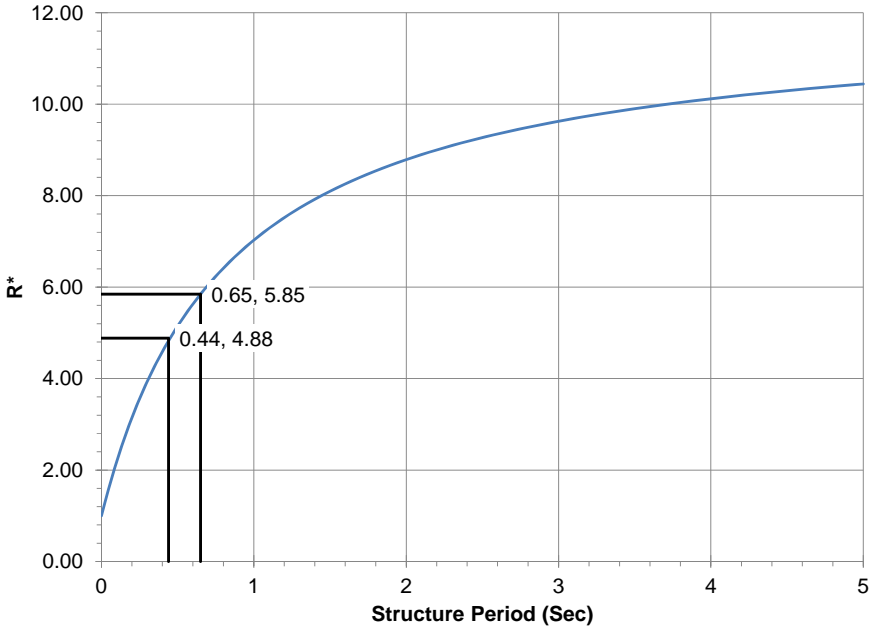
Figure 5-10 Variation in response modification coefficient, R^* , as a function of period.
