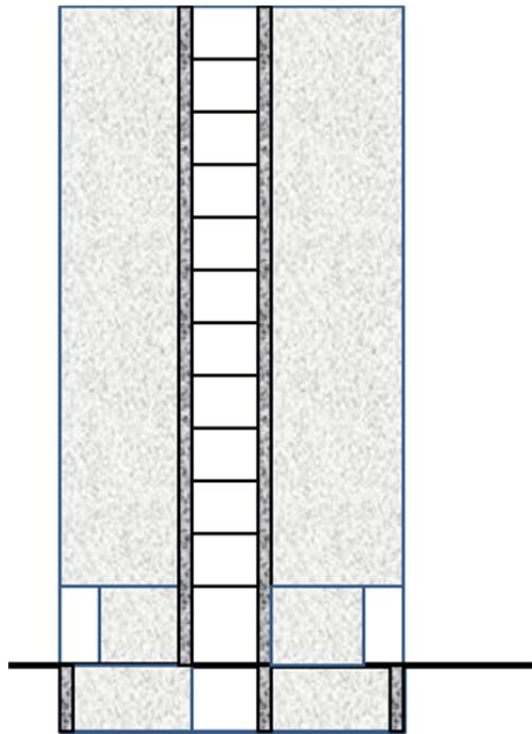
Figure 2-4 Typical cross-section of mid-rise residential building in Chile.
