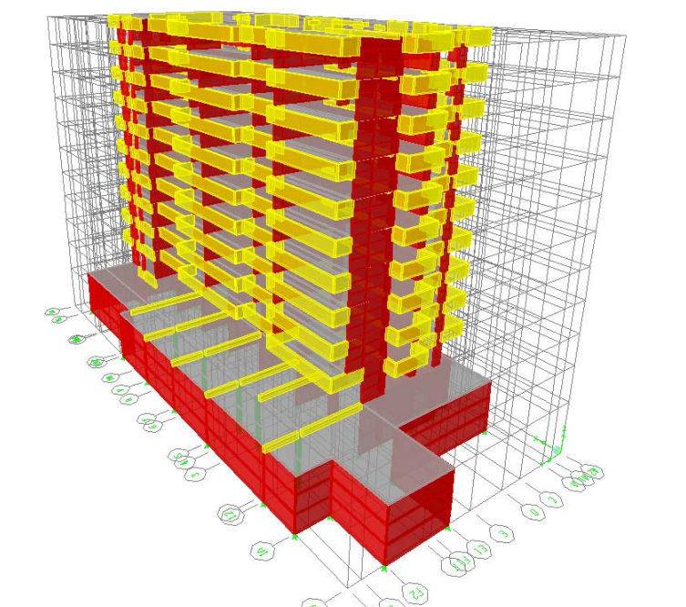
Figure 5-8 Three-dimensional ETABS model of the Chilean configuration of the case study building.
