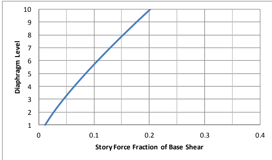
Figure 3-11 Story force distribution as a fraction of base shear, for a hypothetical 10-story structure with T=1 second.
