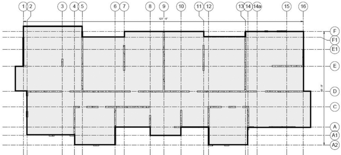
Figure 5-1 Typical floor plan, Chilean case study building.
