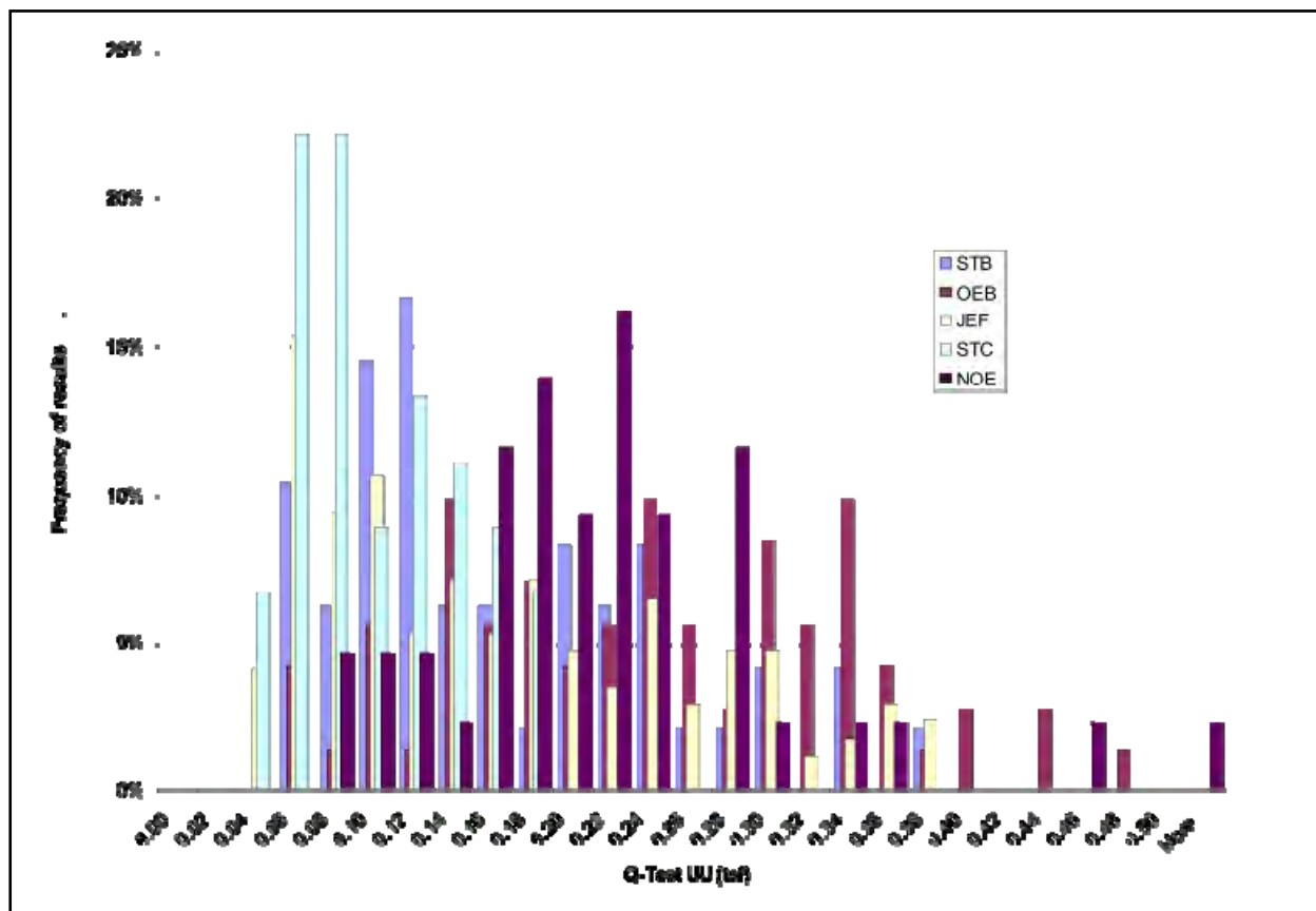
Figure 55. Histograms of undrained strength data (Q-tests), by parish, from USACE GDM of various projects.
