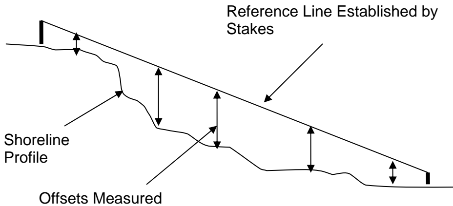
Figure 4.2b Elevation Profile Measurement Approach B
