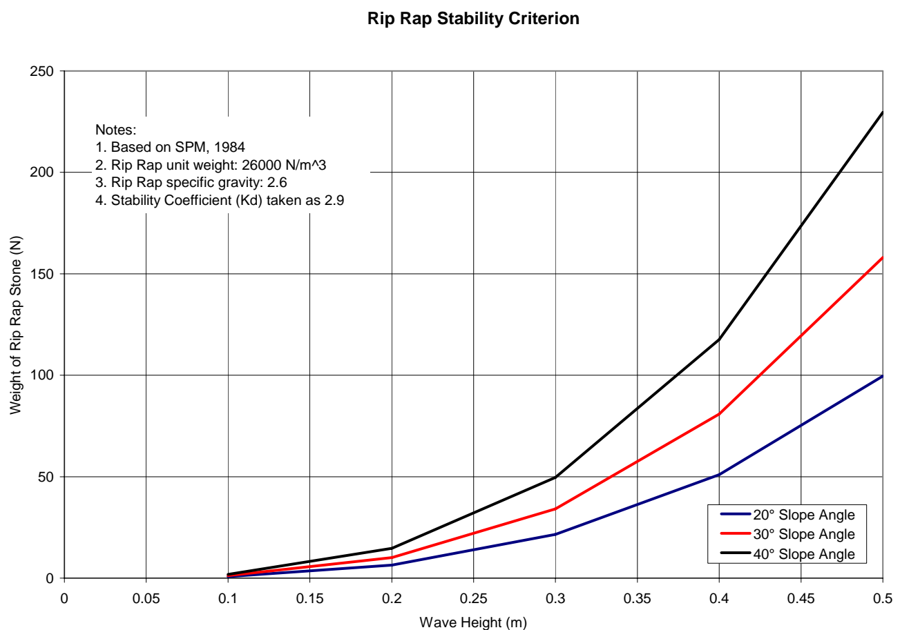
Figure 4.7 Rip-Rap Stability Function (Stanley Island, May 14, 2008)
