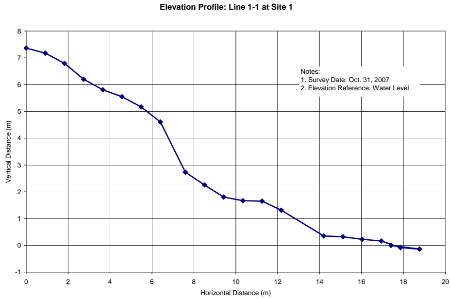
Figure 4.2a Elevation Profile Measurement Approach A
