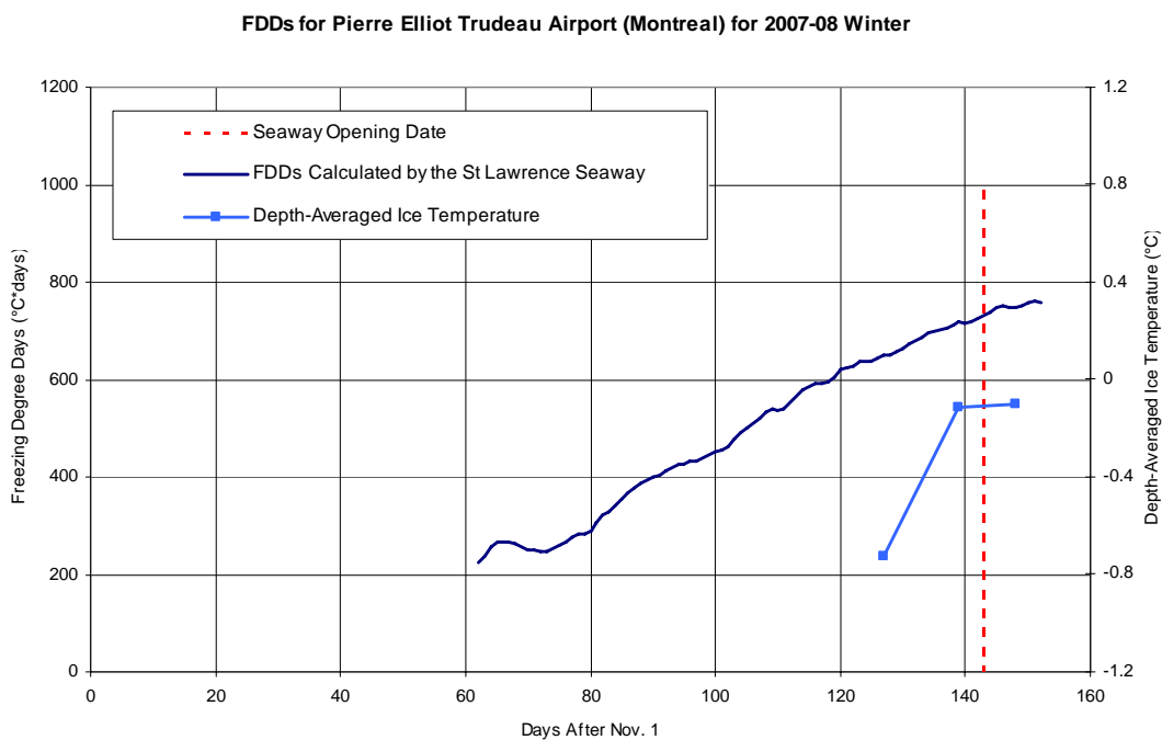
Figure 5.15 Freezing Degree Days (2007/2008 Annual Report)
