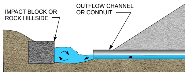
9.35e IMPACT BLOCK STILLING MECHANISM
