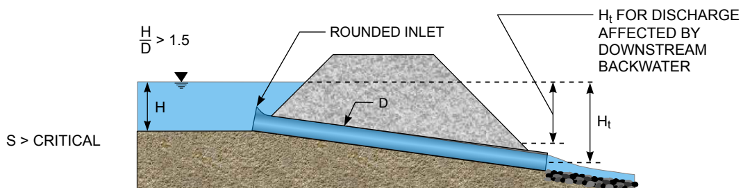
9.32d STEEP SLOPE CONTROL AT OUTLET EFFECTIVE HEAD = H_t - \Sigma LOSSES
