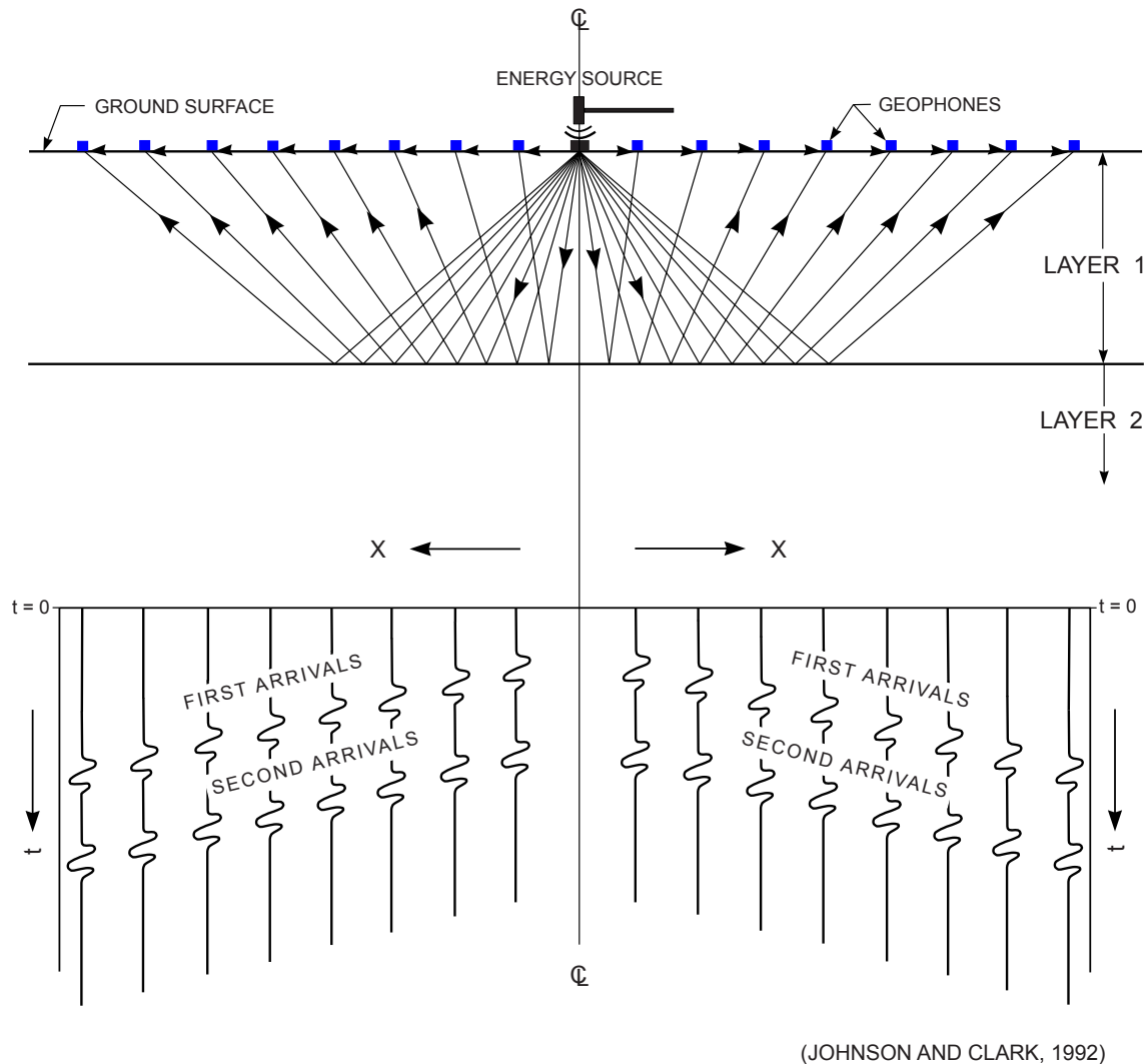
FIGURE 6.17 SEISMIC REFLECTION PRINCIPLE AND SCHEMATIC OF REFLECTION DATA RECORD
