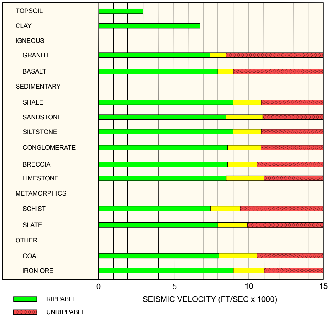
FIGURE 6.16 CORRELATION OF RIPPABILITY WITH P-WAVE VELOCITY FOR CATERPILLAR D9
