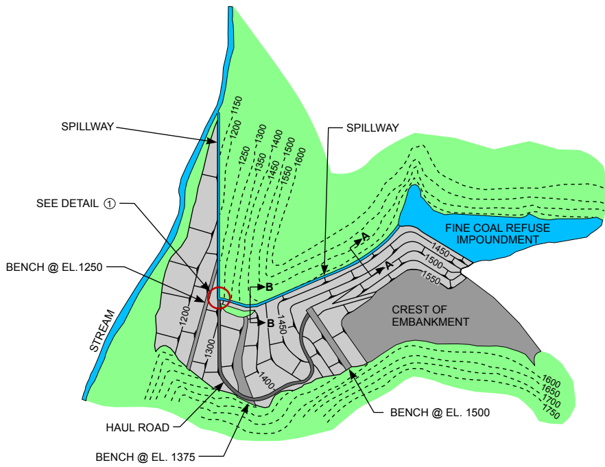
9.41a PLAN
