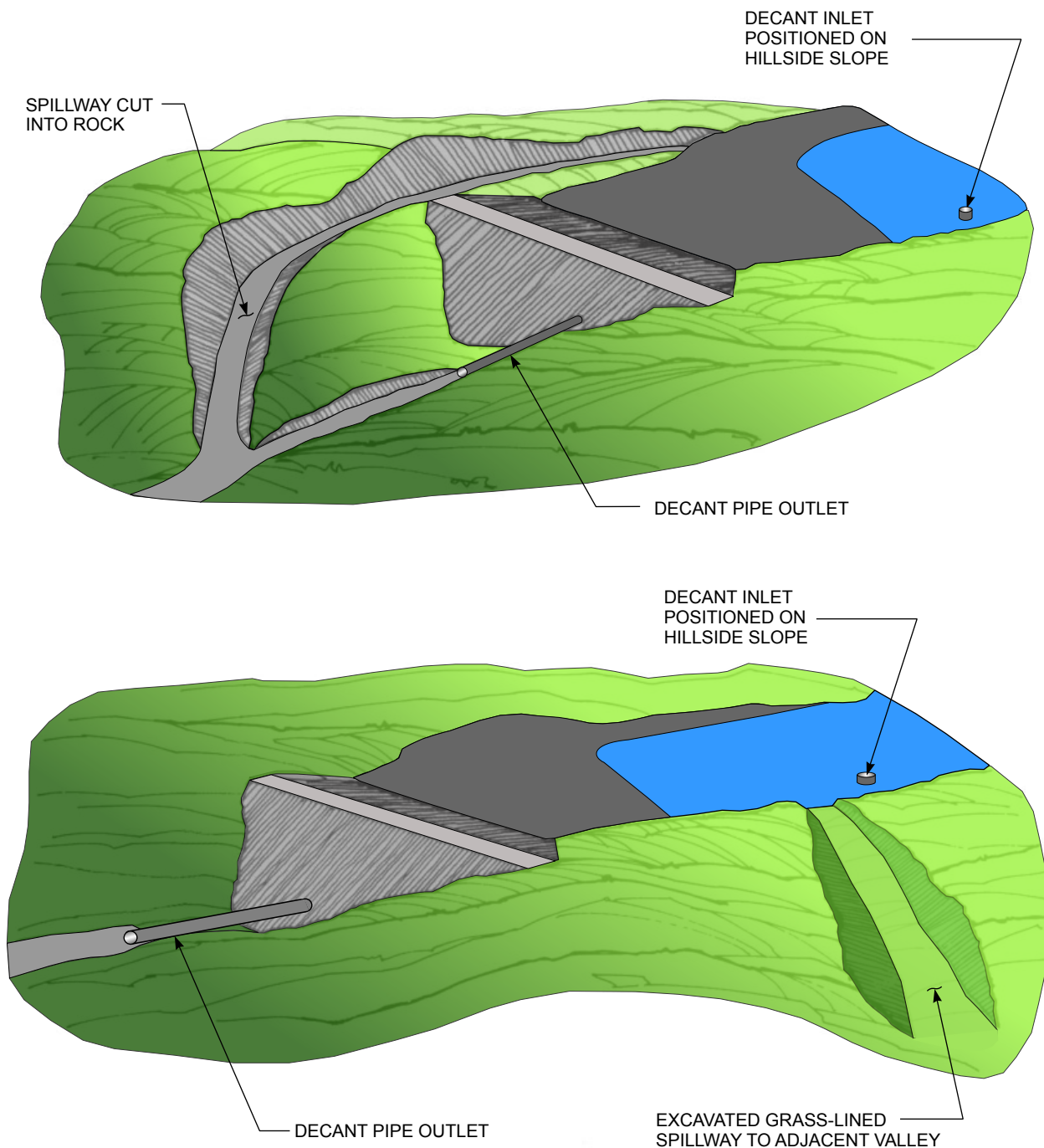
FIGURE 9.6 TYPICAL DECANT AND SPILLWAY SYSTEMS
