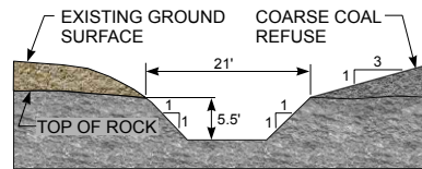
9.41d SECTION B - B
