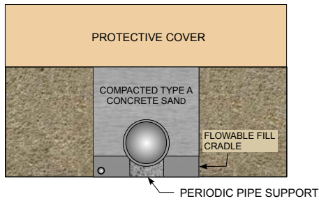
9.40c SECTION A - A
