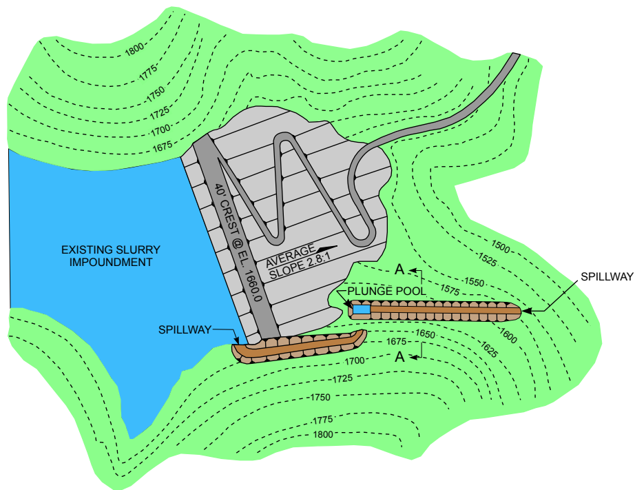
9.43a PLAN
