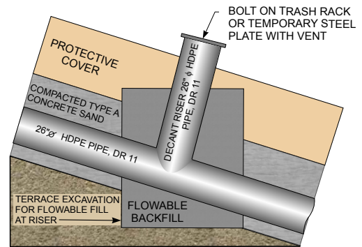
9.40f SECTION D - D
