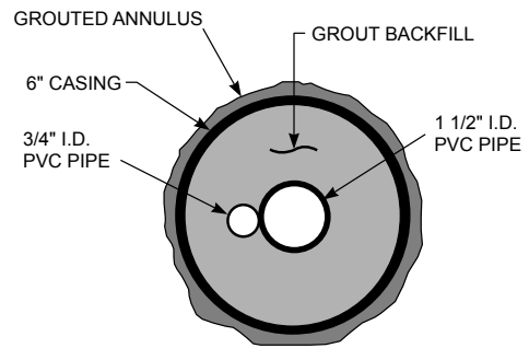
SECTION A - A (SEE DETAIL 2)
