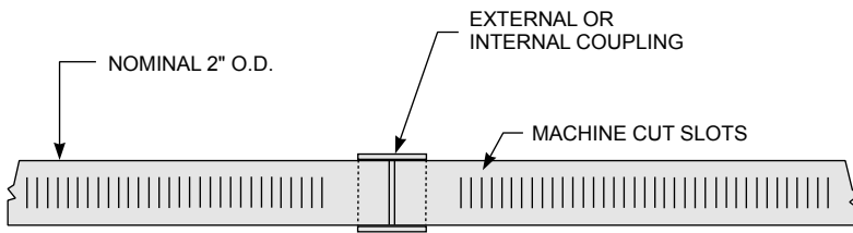
DETAIL 1 - 1 1/2" I.D. PVC PIPE WITH 0.02" MACHINE-CUT SLOTS
