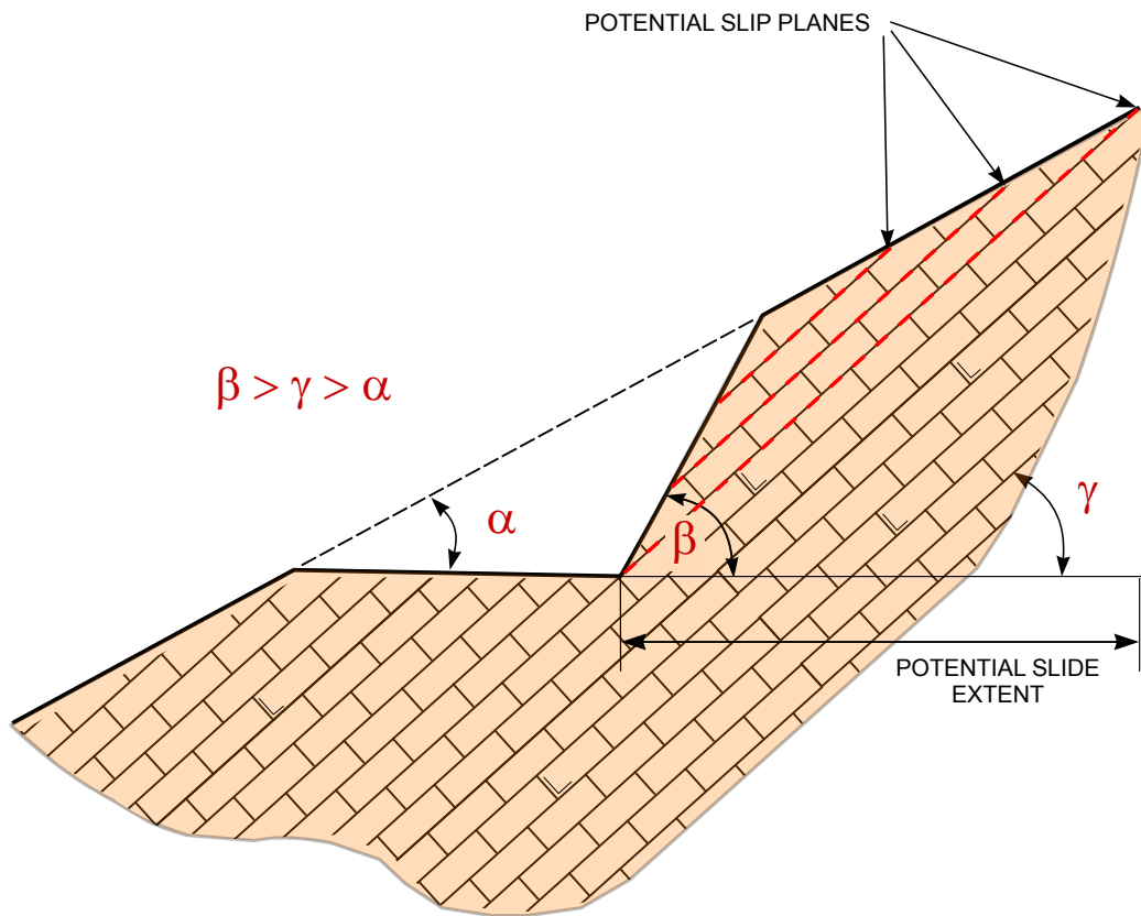
6.58a EXTENT OF POTENTIAL SLIDE (SMALL)
