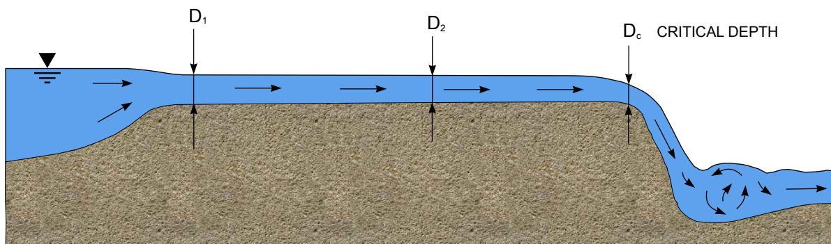
9.28c MILD SLOPE WITH STEEP DROP
