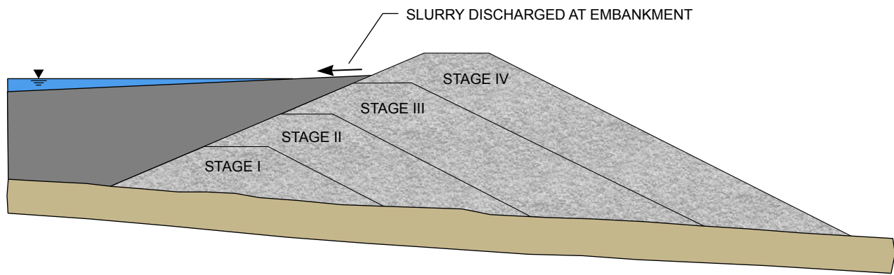
FIGURE 3.6 DOWNSTREAM STAGING METHOD
