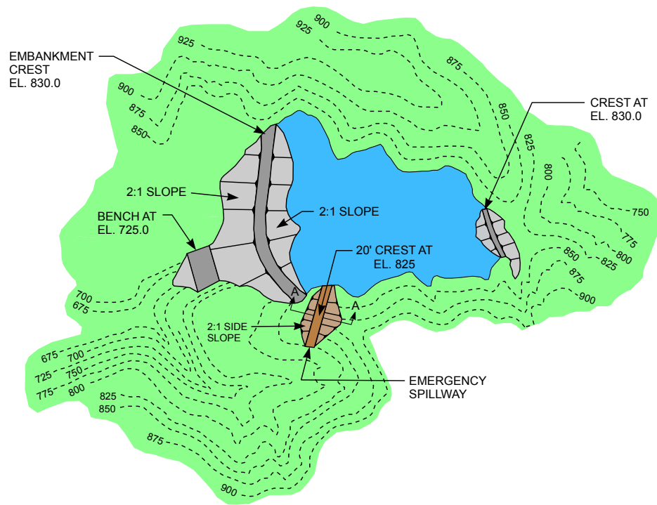
9.42a PLAN
