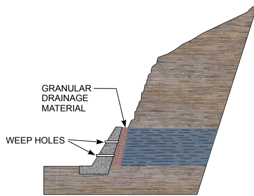
RETAINING WALL
