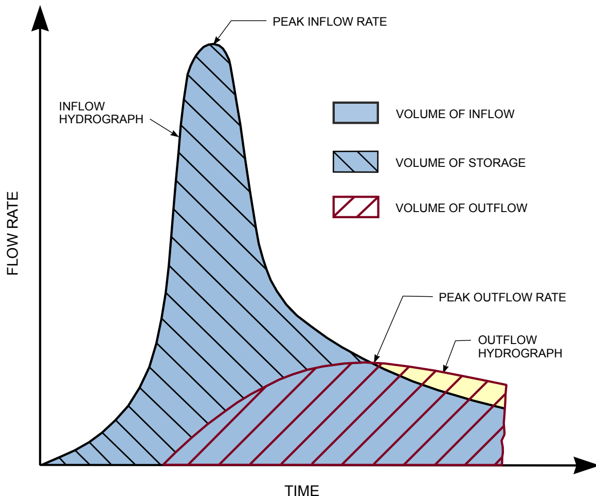
FIGURE 9.3 TYPICAL IMPOUNDMENT INFLOW AND OUTFLOW HYDROGRAPHS
