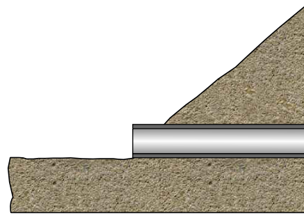
9.33b PROJECTING INLET
