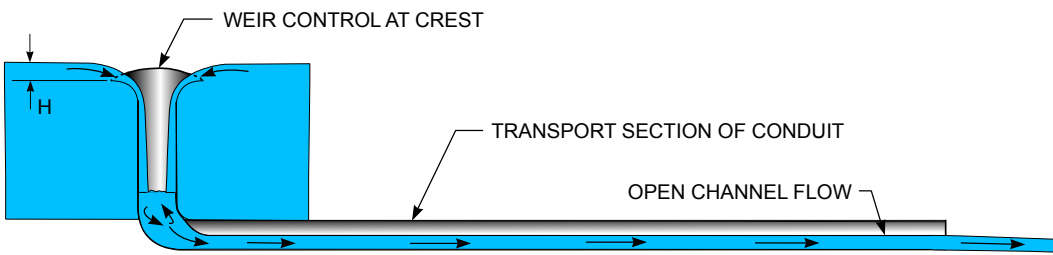
9.34a CURVE A - CREST CONTROL
