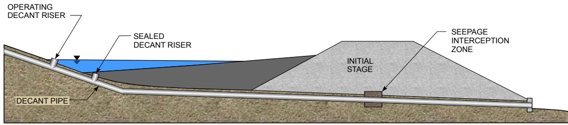
9.40a PROFILE
