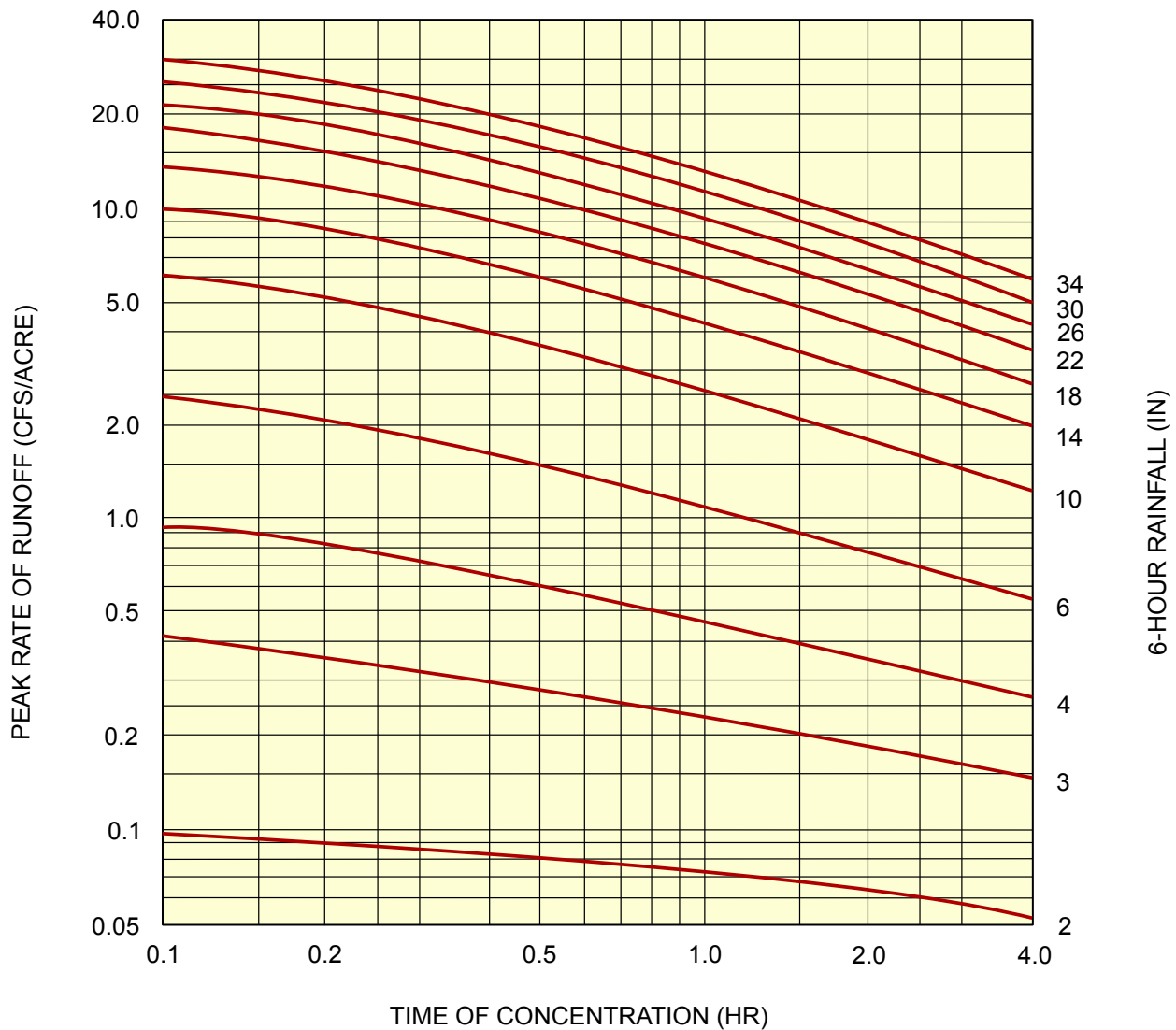
FIGURE 9.21 ESTIMATED PEAK RUNOFF RATE FOR 6-HOUR DESIGN STORM AND CN = 70
