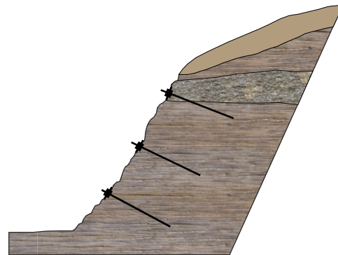
ROCK BOLTS
