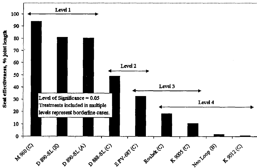
Figure 39. Overall effectiveness groupings for Tremonton, Utah transverse joint seal treatments.
