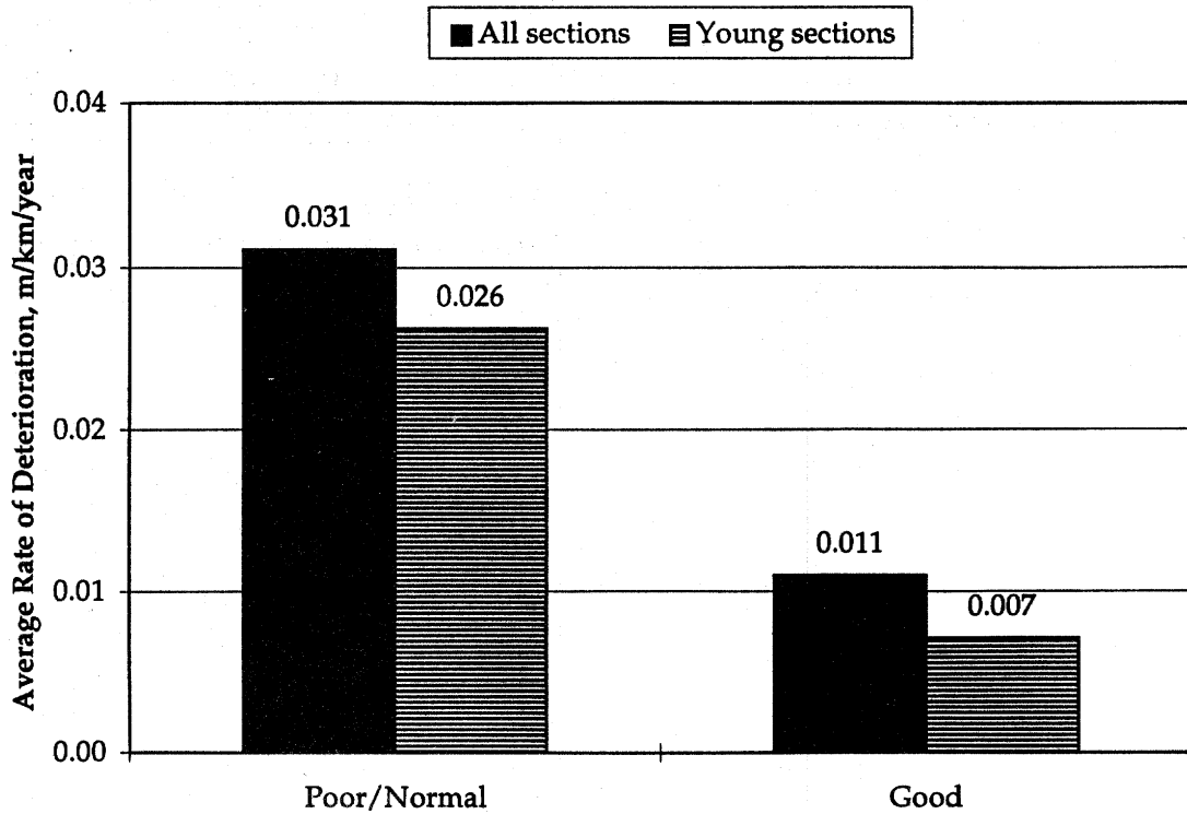
Figure 64. Comparison of average rate of deterioration, \alpha , for CRCP.
