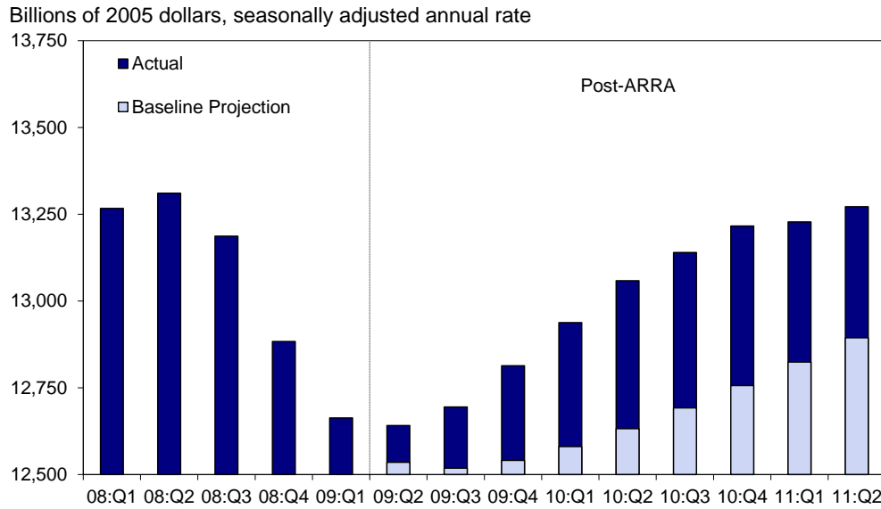
Figure 4. Real GDP: Actual and Baseline Projected Levels
