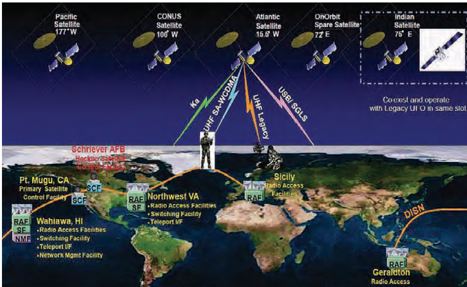
MUOS Architecture
