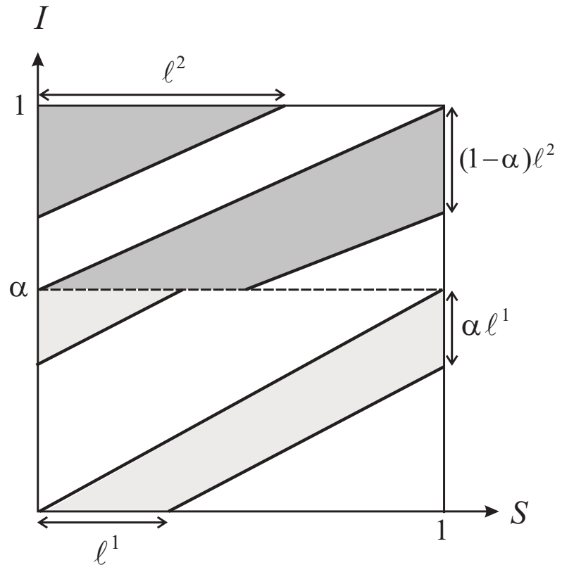
Figure 1: Allocation Rule
