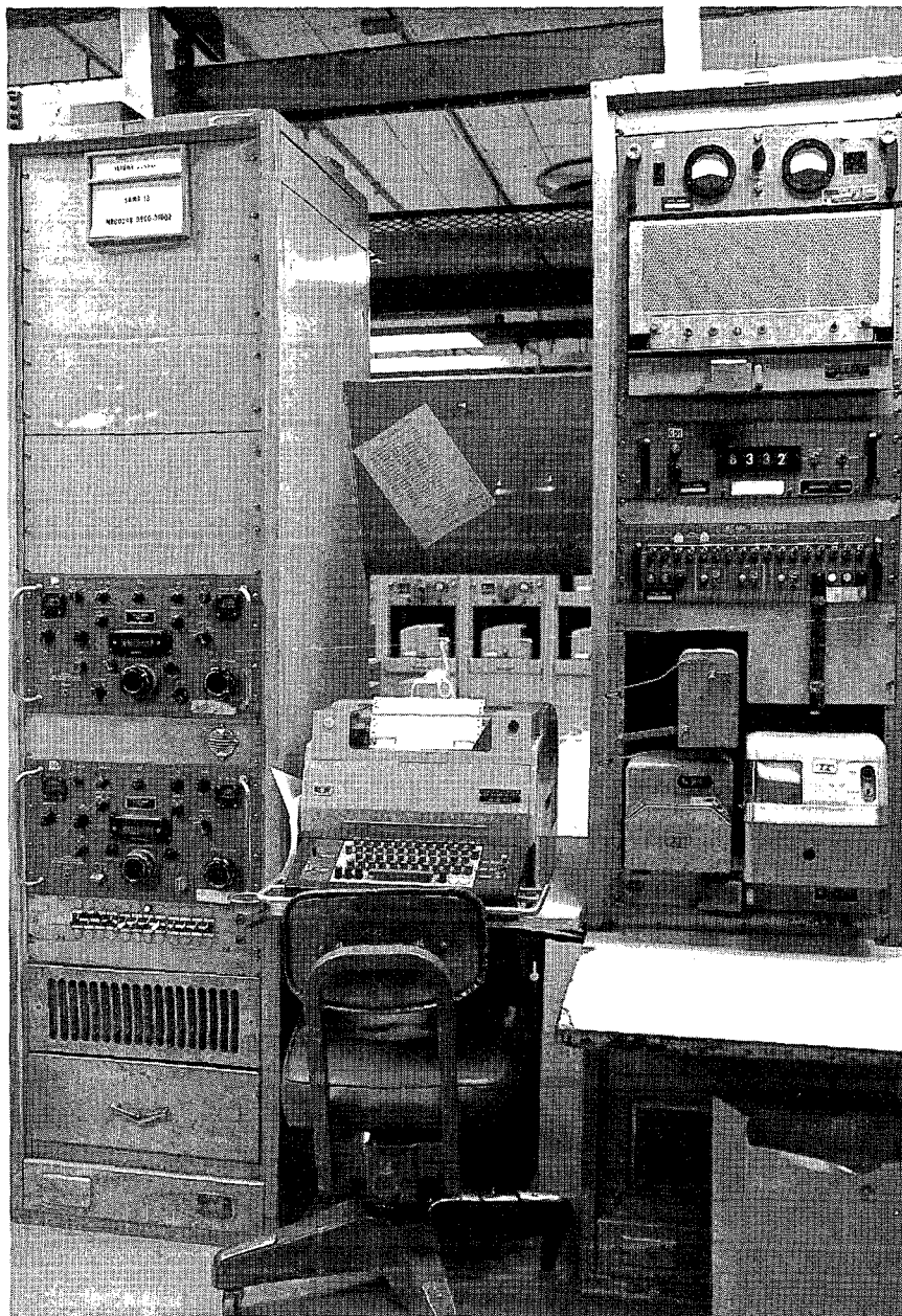
AG-22 - Configured Morse Position at [redacted] (R-390 receivers are in the left-hand rack; MOD-35 in the center; and tape unit on the right)
