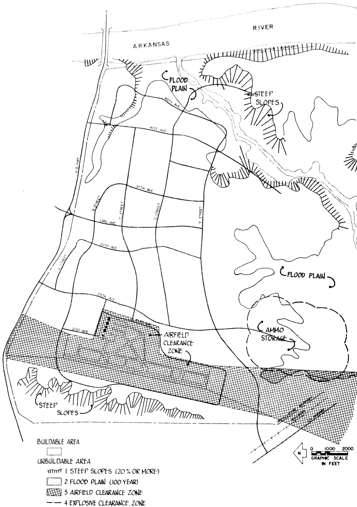
Figure 2-6. Buildable areas.
