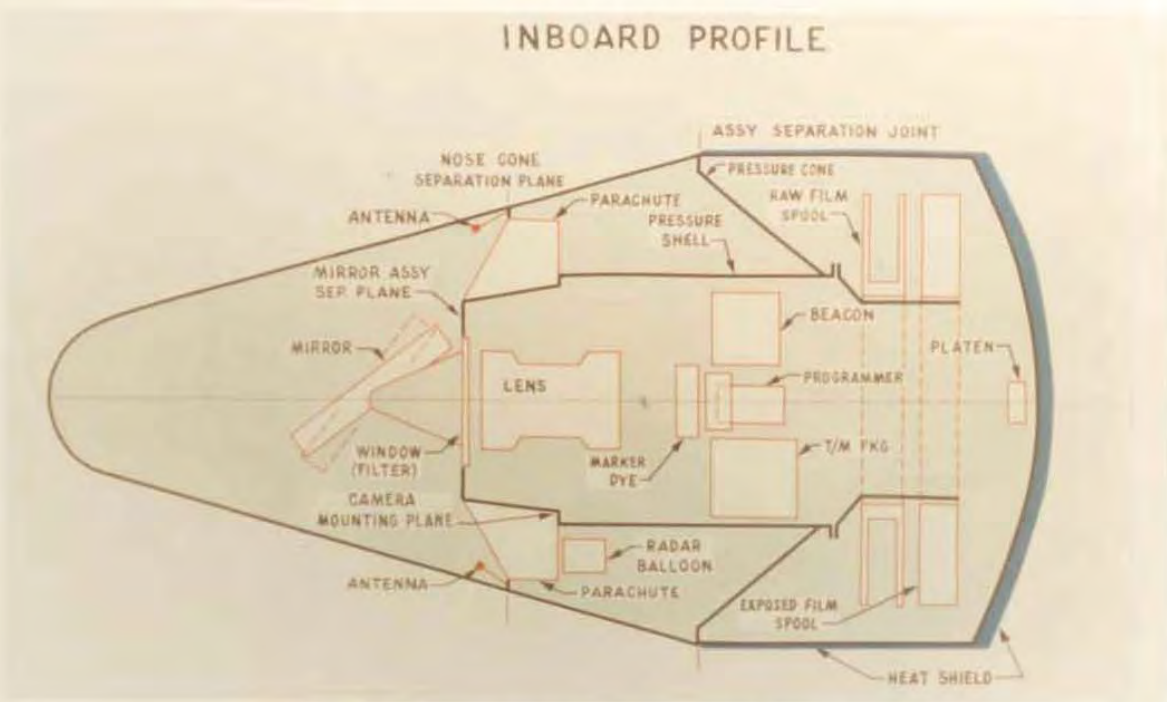
Fig. 1-8b — SAMOS E-5 Recovery Capsule
