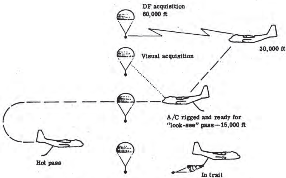
Fig. 3-10 — Typical air recovery sequence
