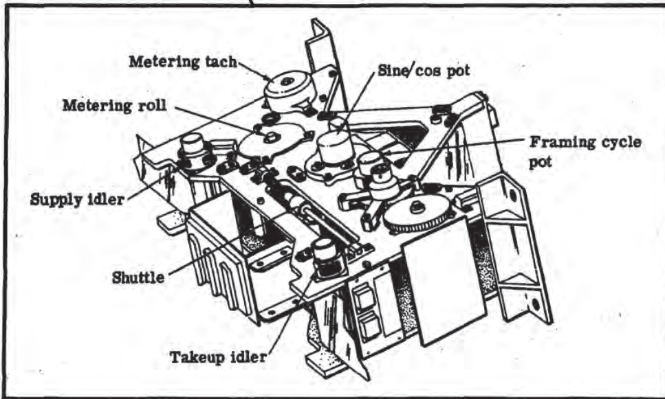
Fig. 2-17 — Stellar camera film transport
