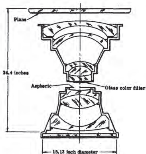
Fig. 2-3 — 12-inch metric lens
