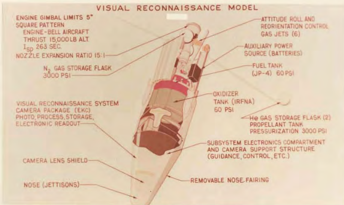
Fig. 1-4a — WS-117L Vehicle System
