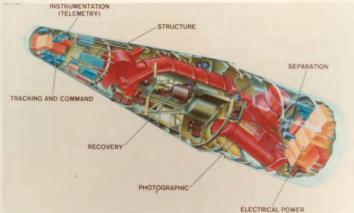
Fig. 1-9 — E-6 Reconnaissance Satellite Subsystems
