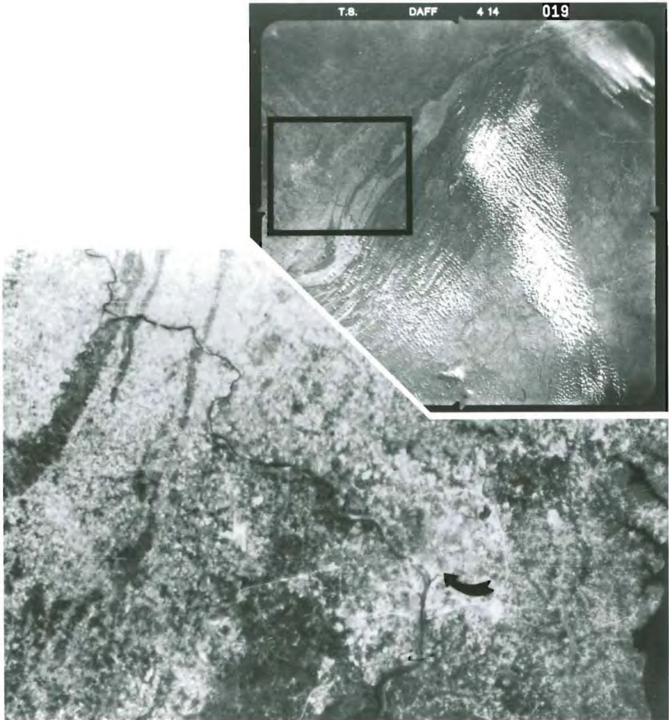
Fig. 1-31 — KH-5 Army Mapping Camera System imagery (CORONA-ARGON); contact (partial frame) and 7x enlargement
