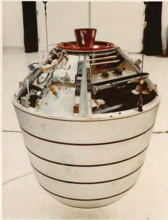
Fig. 1-16 a — Mark V reentry vehicle
