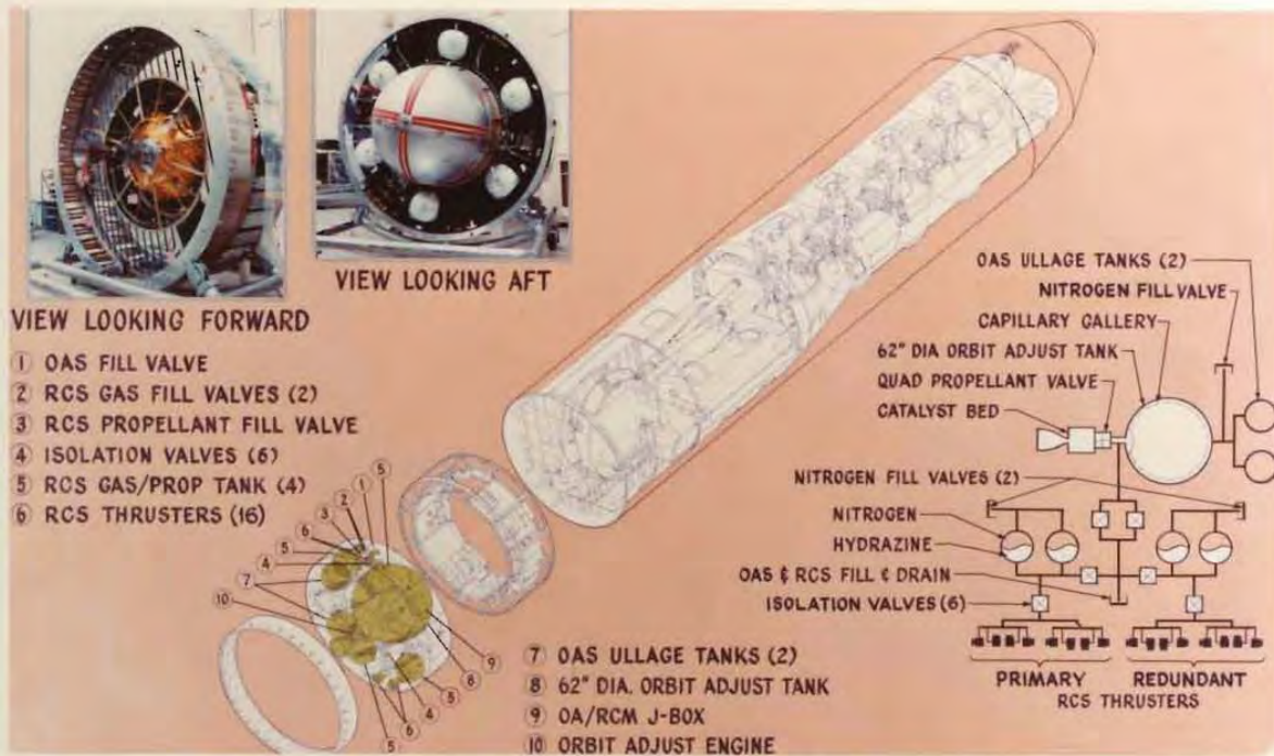
Fig. 1-8 — Orbit adjust and reaction control
