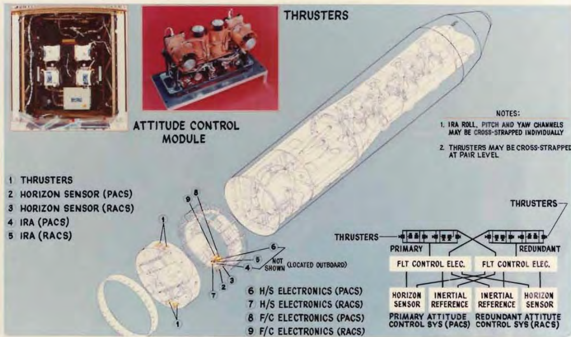
Fig. 1-7 — Attitude control
