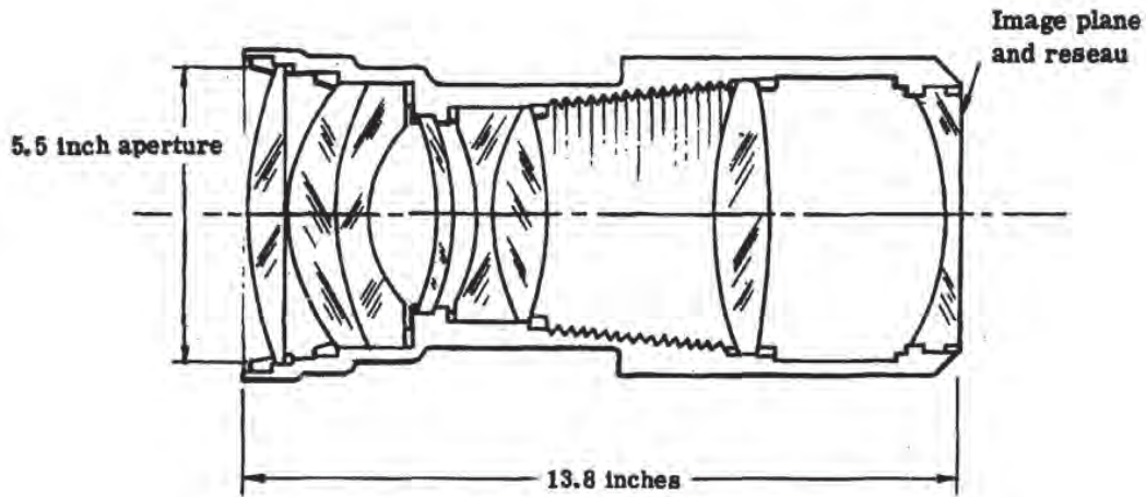
Fig. 2-4 — 10-inch stellar lens
