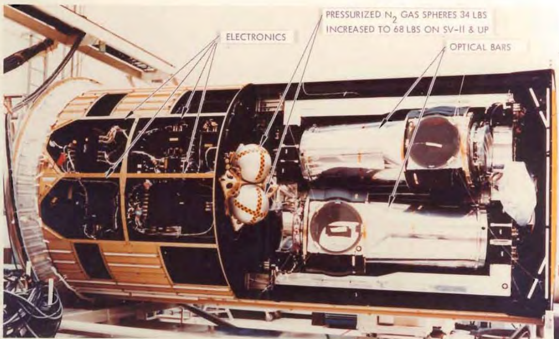
Fig. 1-14 — Two camera assembly
