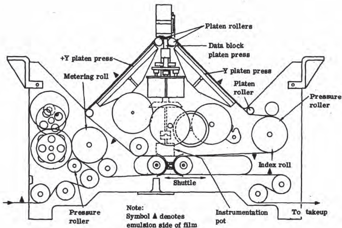
Fig. 2-18 — Stellar transport film flow
