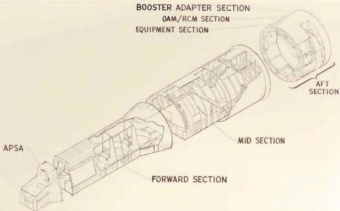
Fig. 1-5 — Satellite Basic Assembly structure
