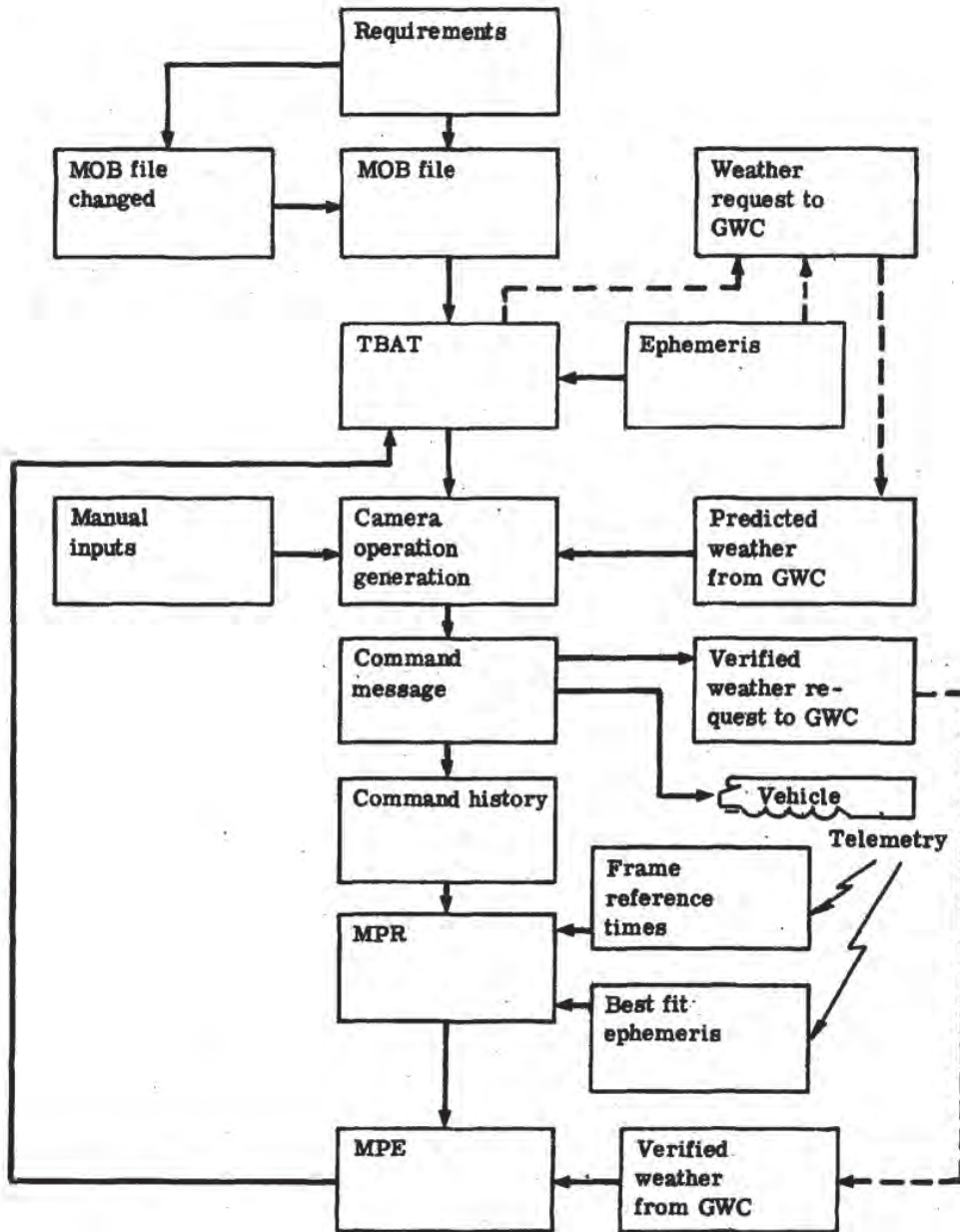
Fig. 3-8 — Mapping Camera operational data flow
