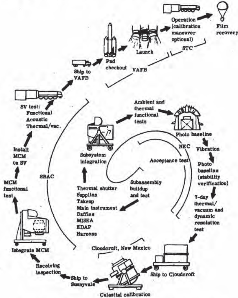
Fig. 2-20 — Mapping camera integration and operational flow
