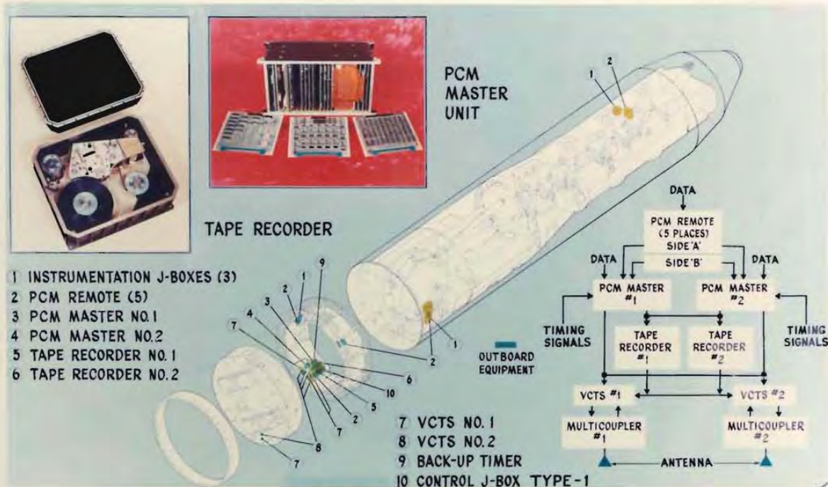
Fig. 1-10 — Telemetry and tracking
