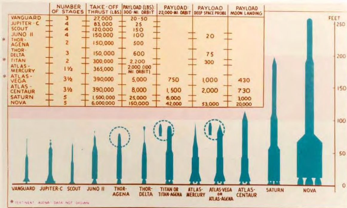
Fig. 1-2b — U.S. space vehicles as viewed in 1959
