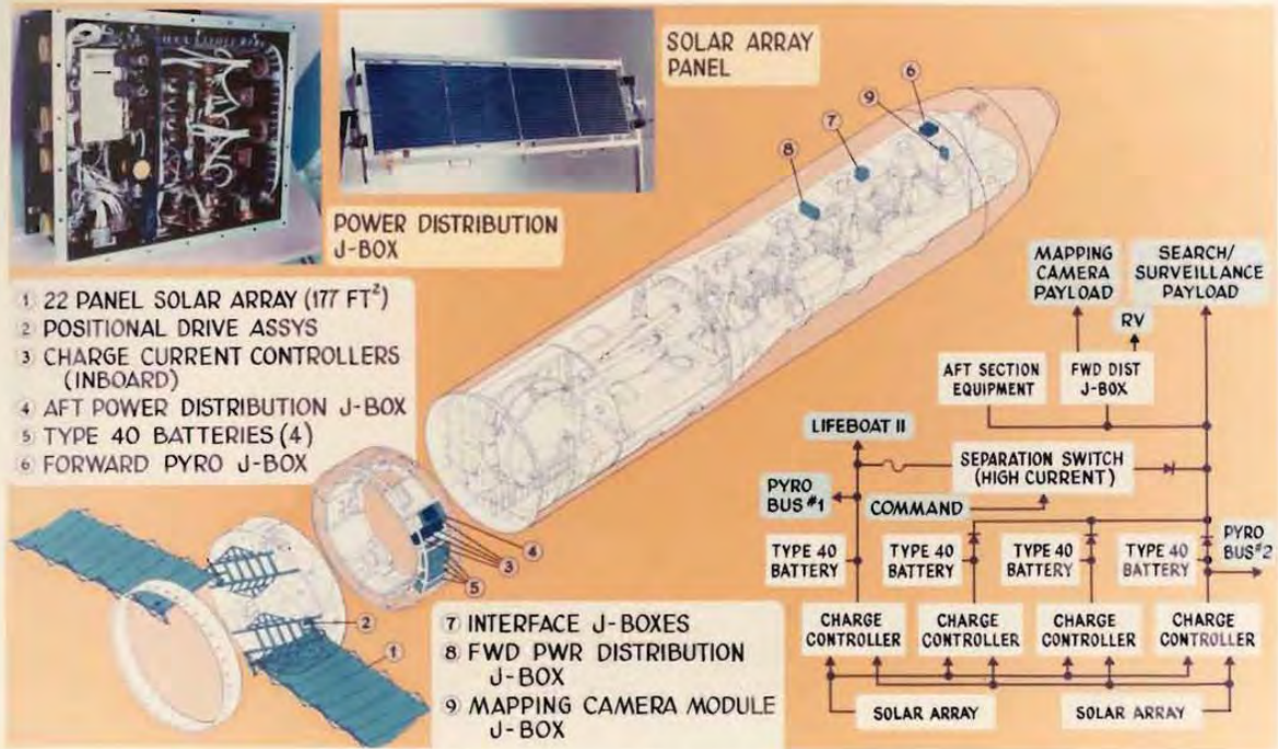
Fig. 1-9 — Electrical distribution and power
