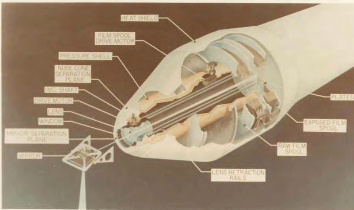
Fig. 1-8a — SAMOS E-5 Recovery Camera Payload
