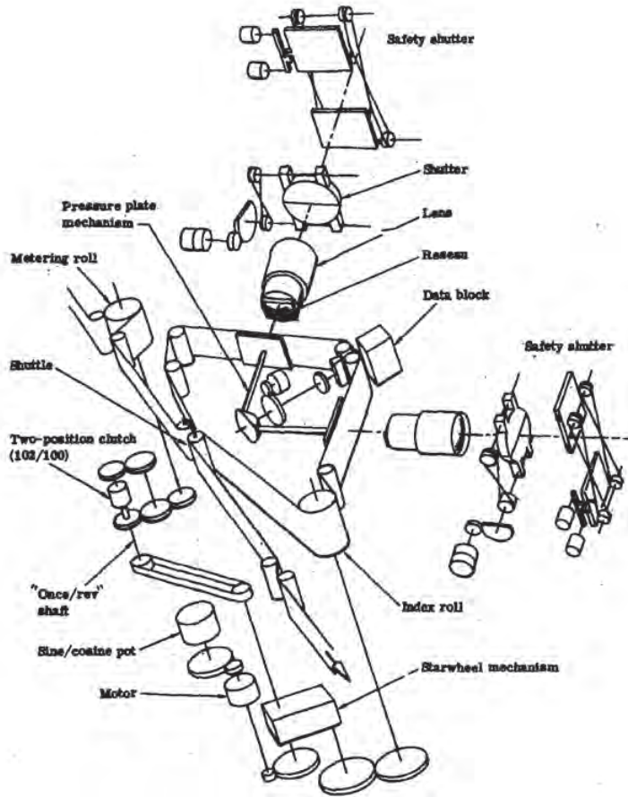
Fig. 2-10 — Stellar camera mechanical arrangement
