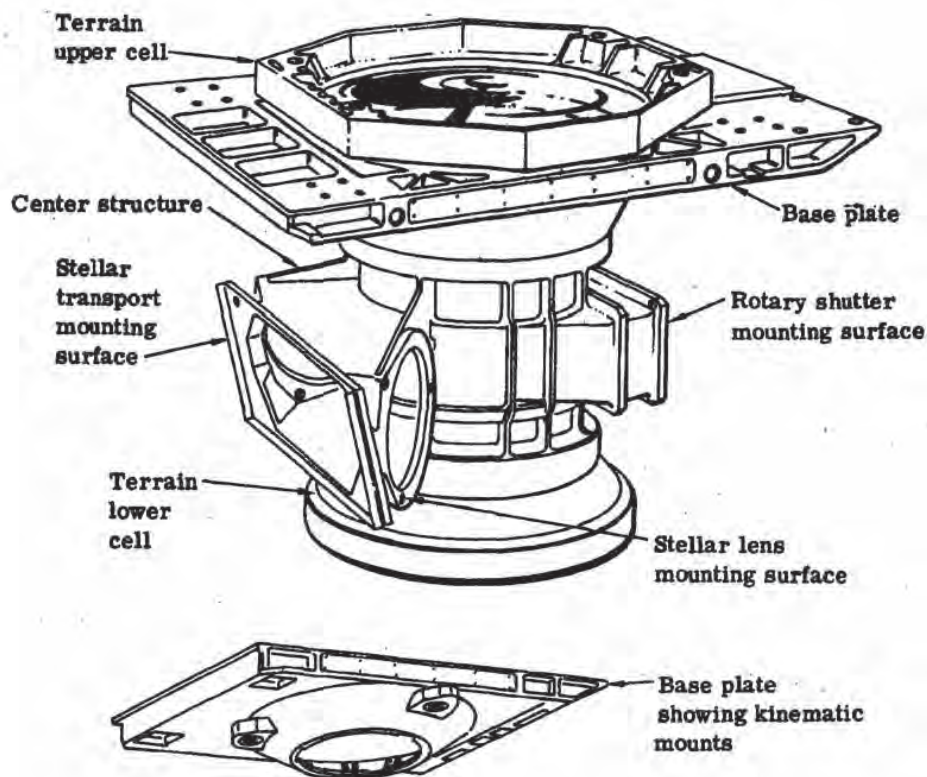
Fig. 2-6 — MC center structure and mechanical interface
