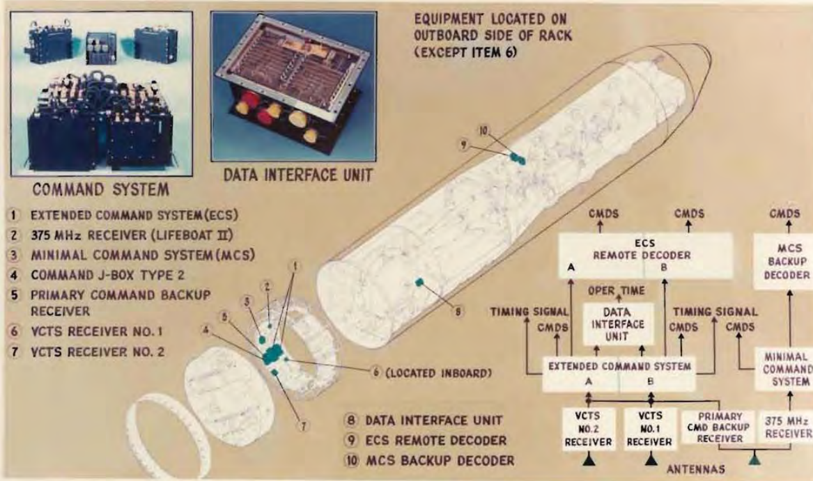
Fig. 1-11 -- Command and timing
