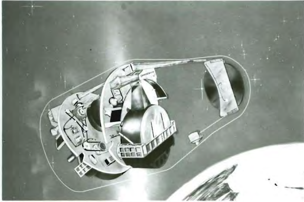
Fig. 1-14 — MURAL (KH-4) Twin Panoramic Camera System
