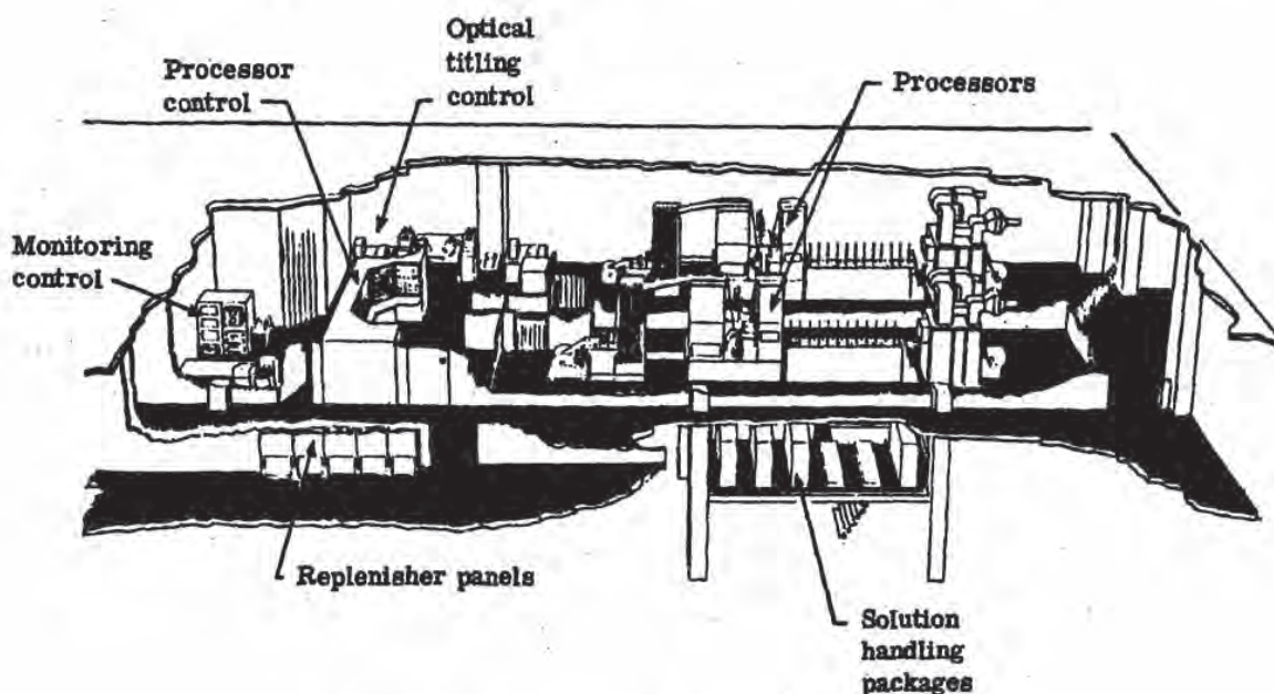
Fig. 4-7 — Ontario processing complex
