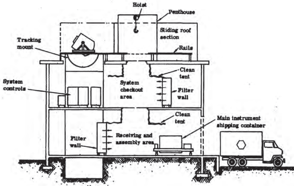
Fig. 2-23 — Cloudcroft Facility
