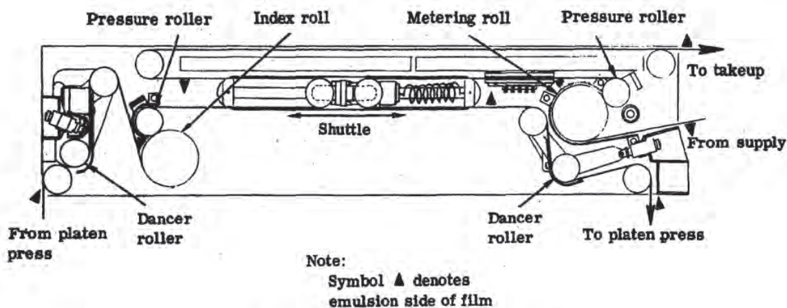
Fig. 2-16 — Terrain transport film flow
