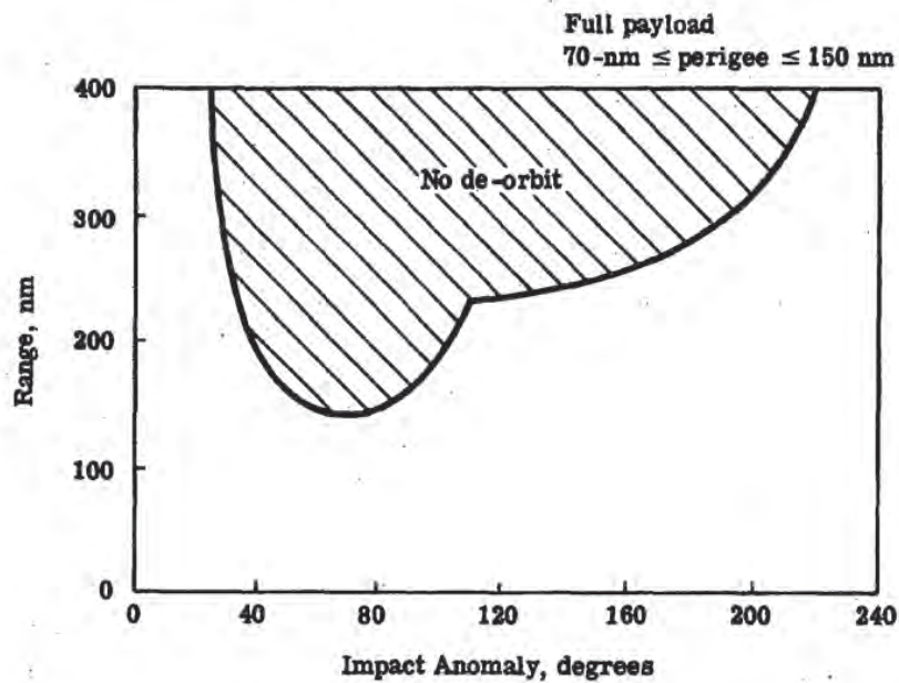
Fig. 1-19 — Operational flight envelope
