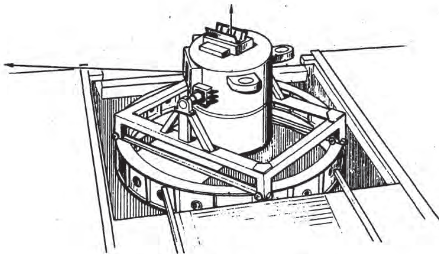
Fig. 2-24 — Cloudcroft calibration enclosure
