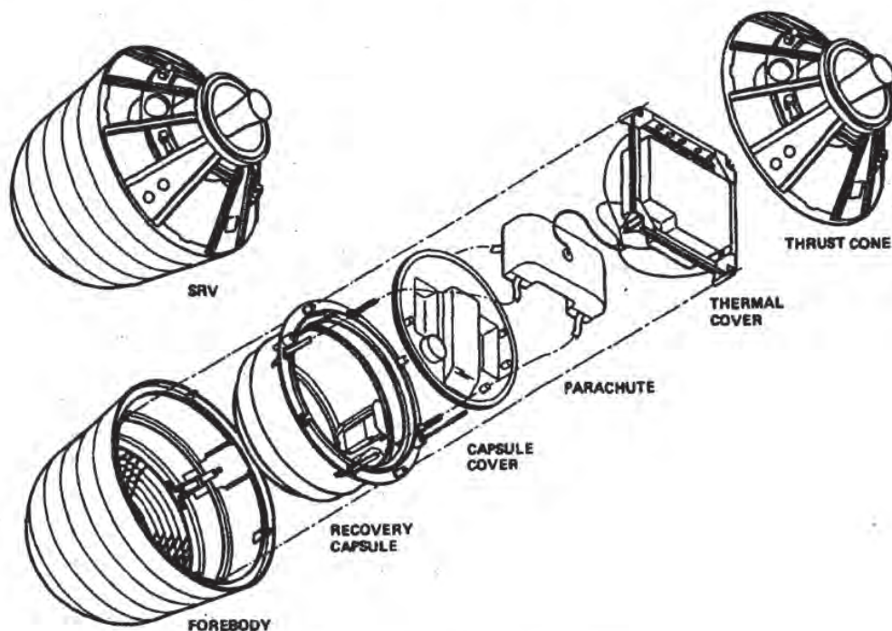
Fig. 1-20 — Mark V SRV (exploded view)
