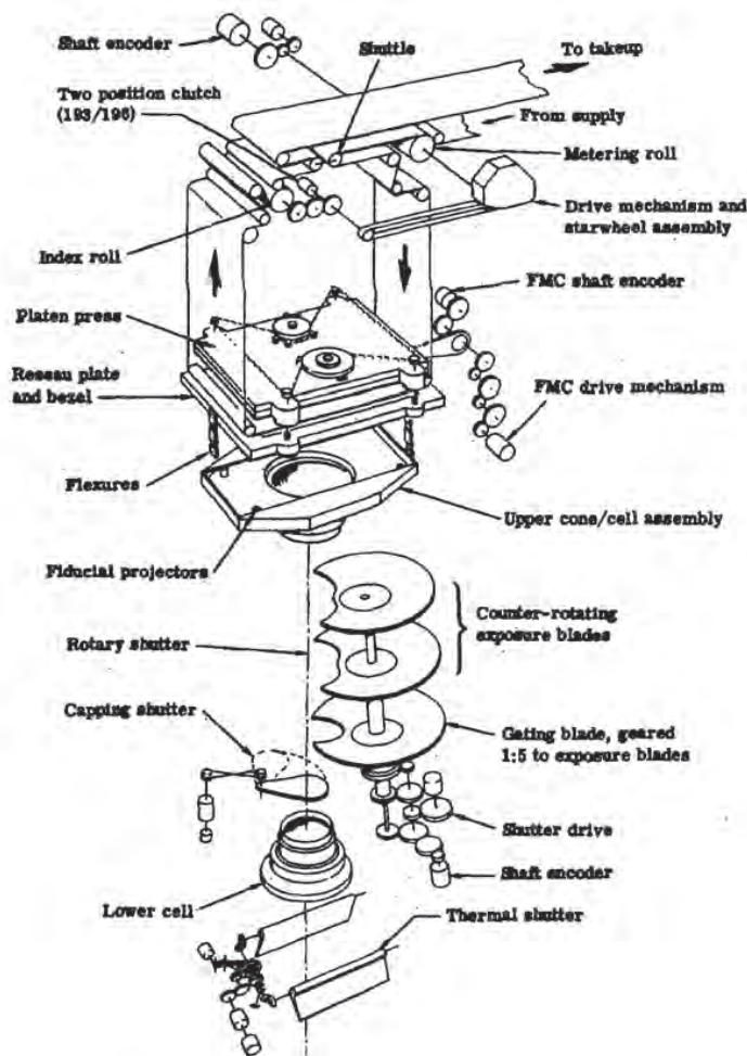
Fig. 2-7 — Terrain camera mechanical arrangement
