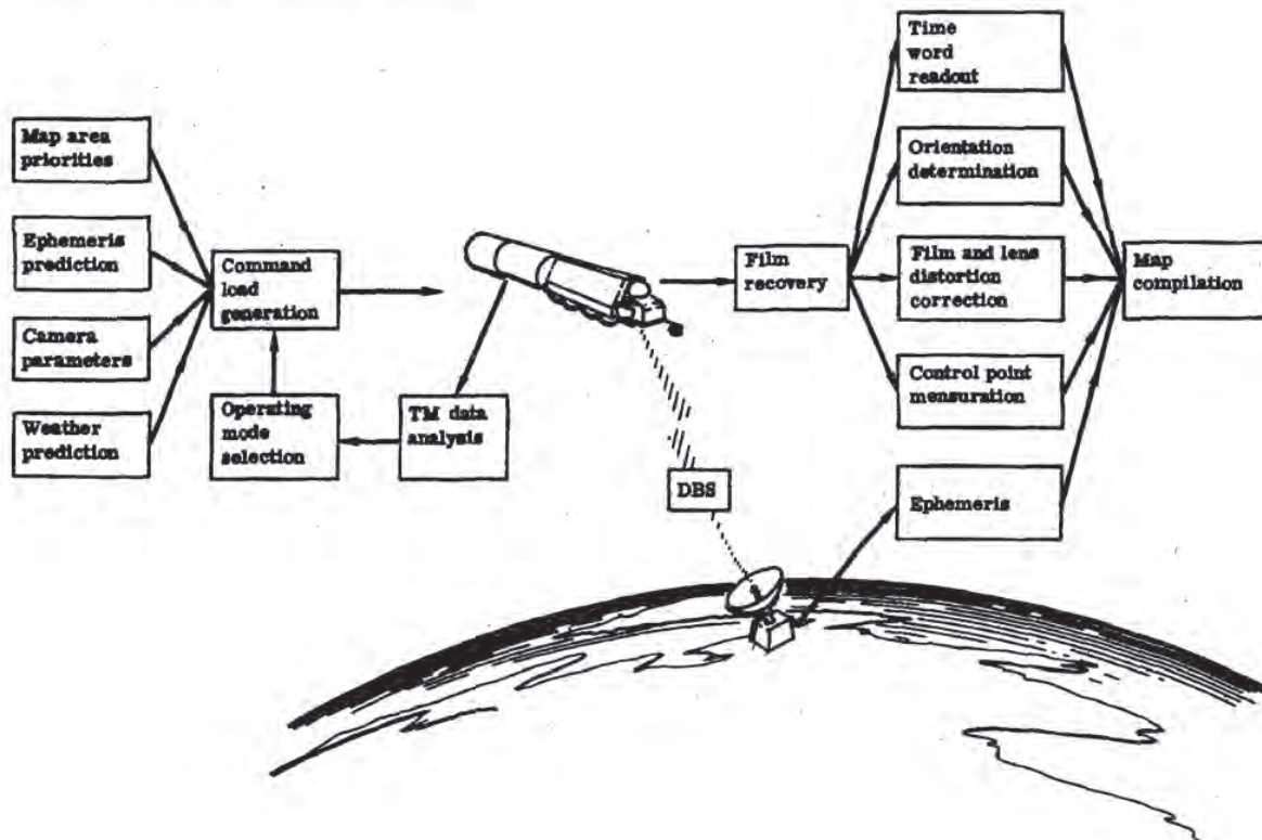
Fig. 3-7 — Mapping Camera operational data flow
