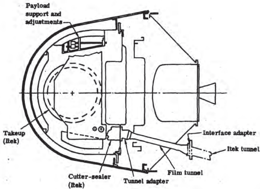
Fig. 1-17b — SRV inboard profile
