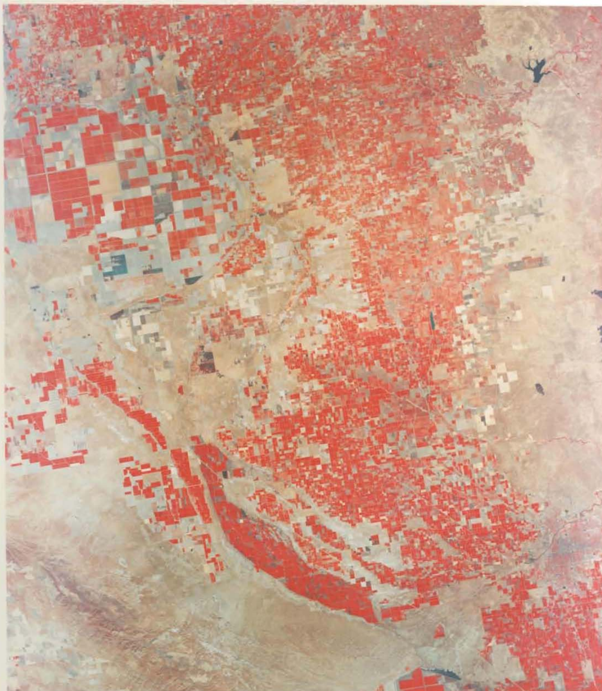
Fig. 8-6 — Experimental photography—IR color; SO-131; contact print
