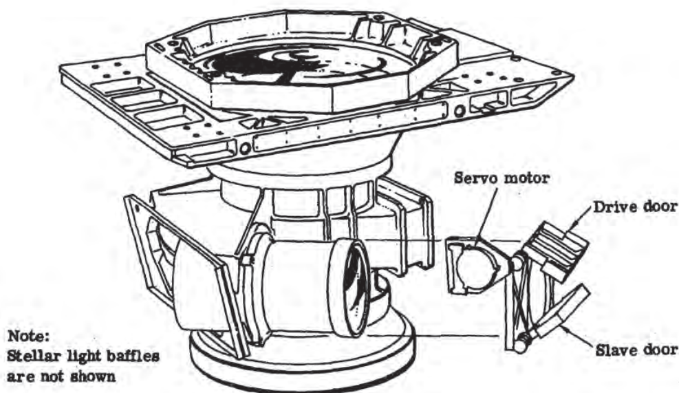
Stellar shutter arrangement
