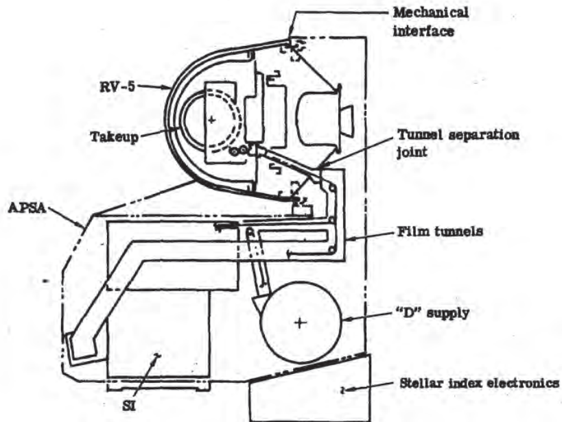
Fig. 1-17a — Mapping Camera Module
