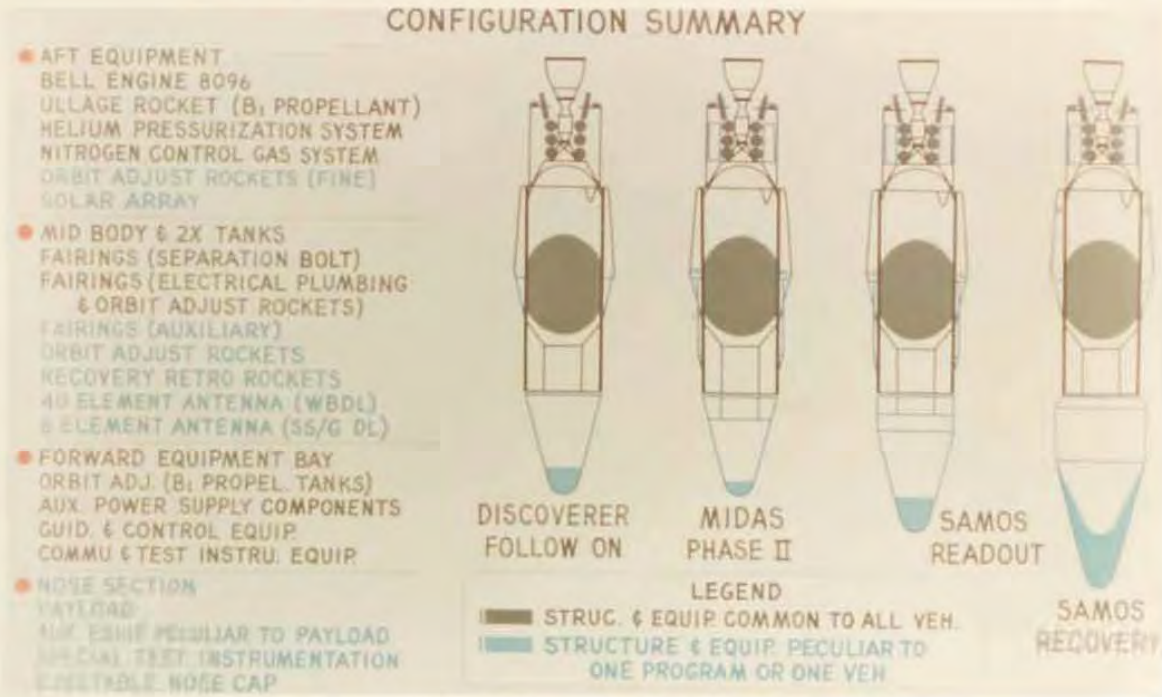
Fig. 1-2a — Standardized Agena as viewed in 1959
