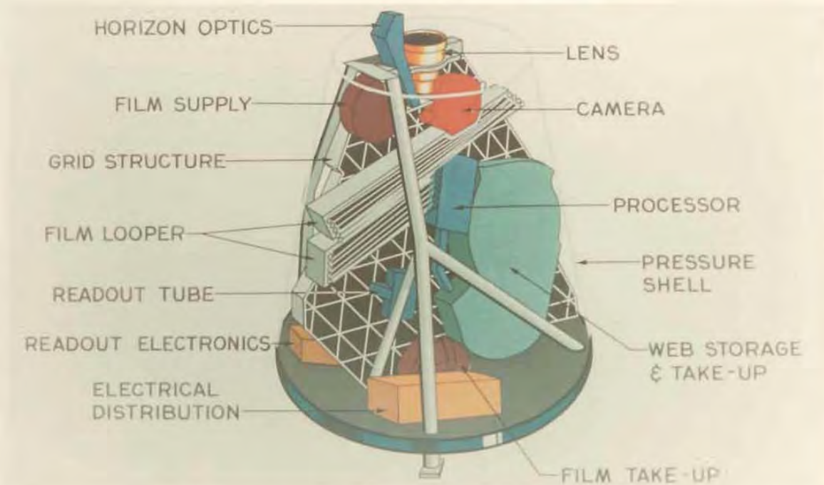
Fig. 1-5 — E-1 Visual Reconnaissance Component Test Model
