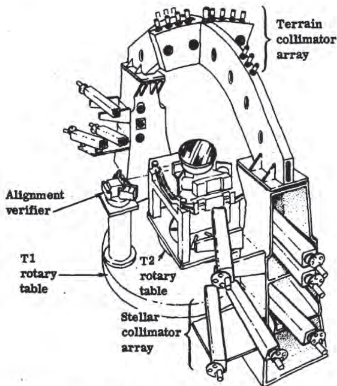
Fig. 2-21 — Distortion boresight test unit (DBTU)
