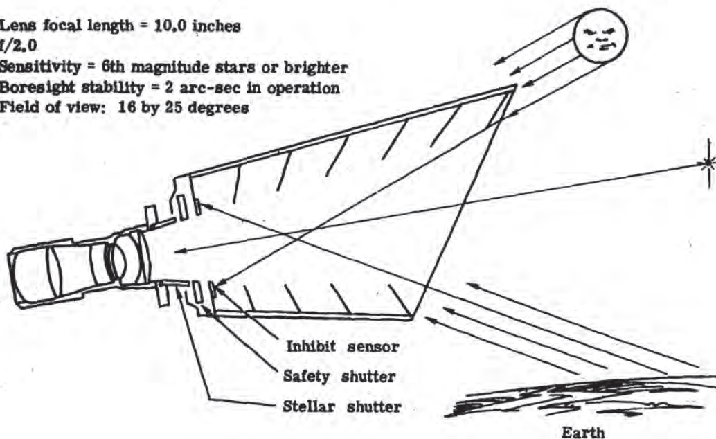
Stellar baffle configuration
