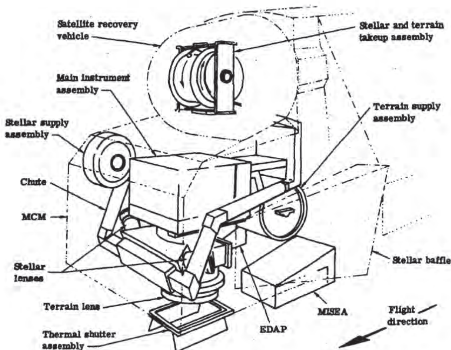
Fig. 2-2 — Mapping Camera major assemblies
