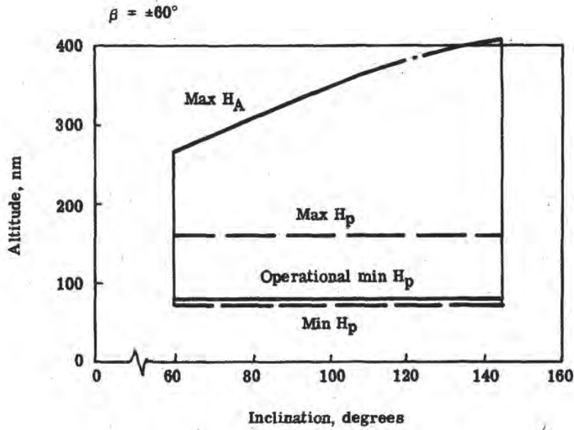
Fig. 1-18 — Mission flight envelope
