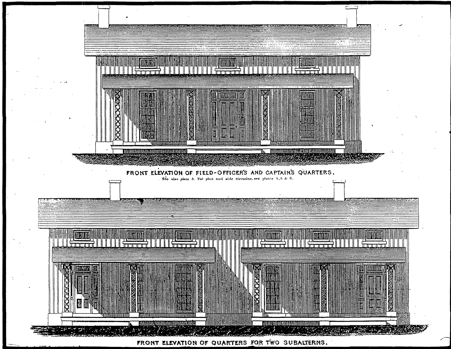
Figure III-130. Proposed 1860 plans for officers quarters. From Regulations Concerning Barracks and Quarters for the Army of the United States 1860 . Washington, D.C.: George W. Bowman, 1861
