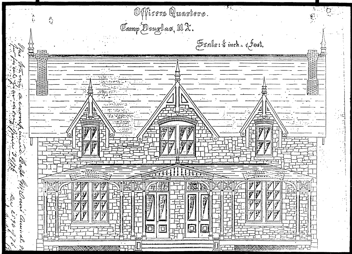
Figure III-134. 1886 officer housing (Building 22112, Ft. Huachuca, Arizona), above . 1876 version of standardized company officers quarters at Ft. Douglas, Utah (From National Archives, Record Group 77, Fortifications File, Ft. Douglas, Utah.), below
