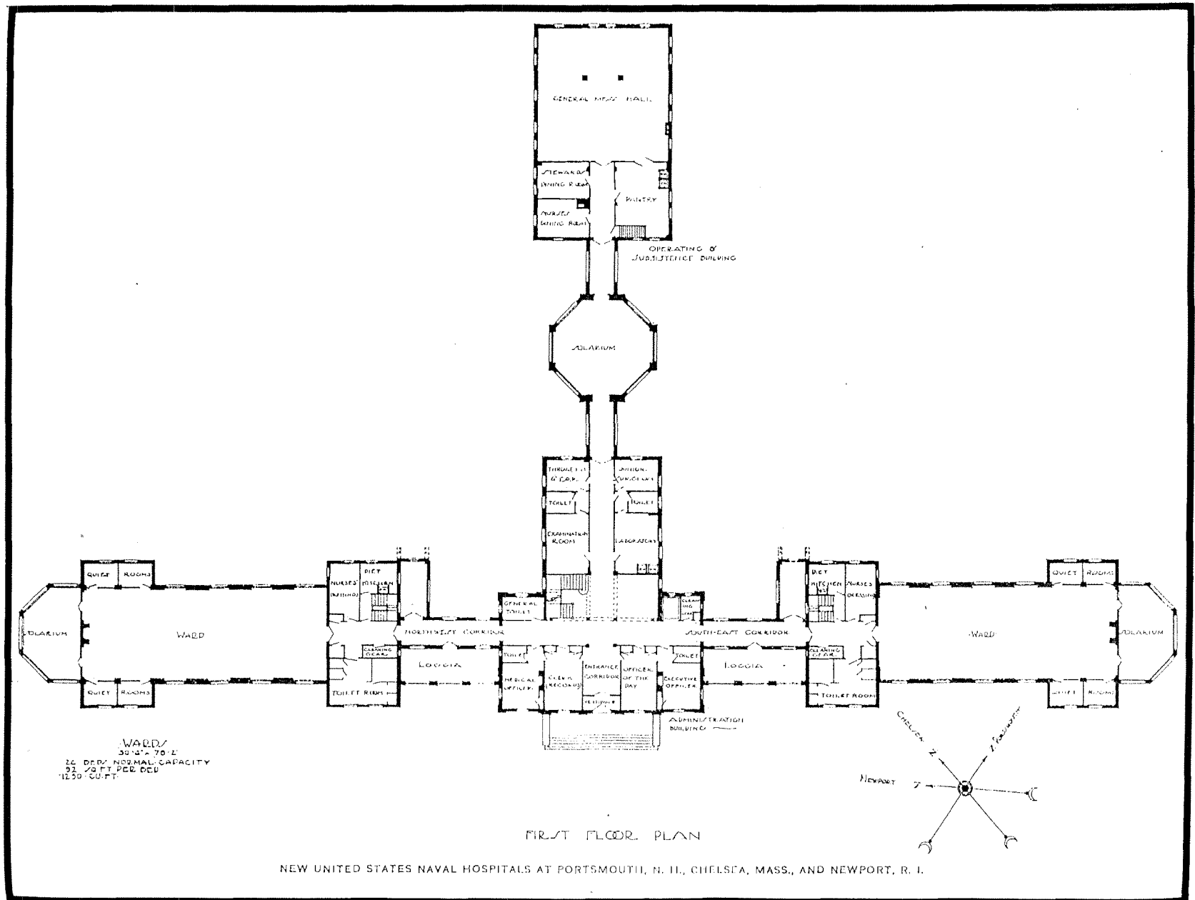
Figure III-48. Plan of naval hospitals constructed at Newport, Rhode Island; Portsmouth, New Hampshire; and, Chelsea, Massachusetts. (From A.W. Dunbar, A Description of Recent Hospital Construction in the United States Navy .)
