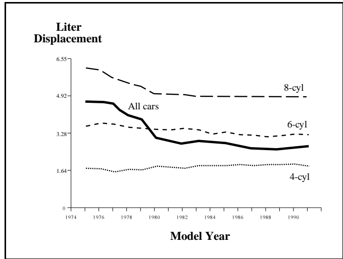
Figure 13. Engine Displacement, by Number of Cylinders: 1975-1991
