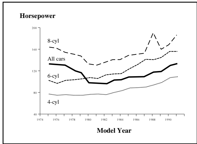
Figure 14. Engine Horsepower, by Number of Cylinders: 1975-1991
