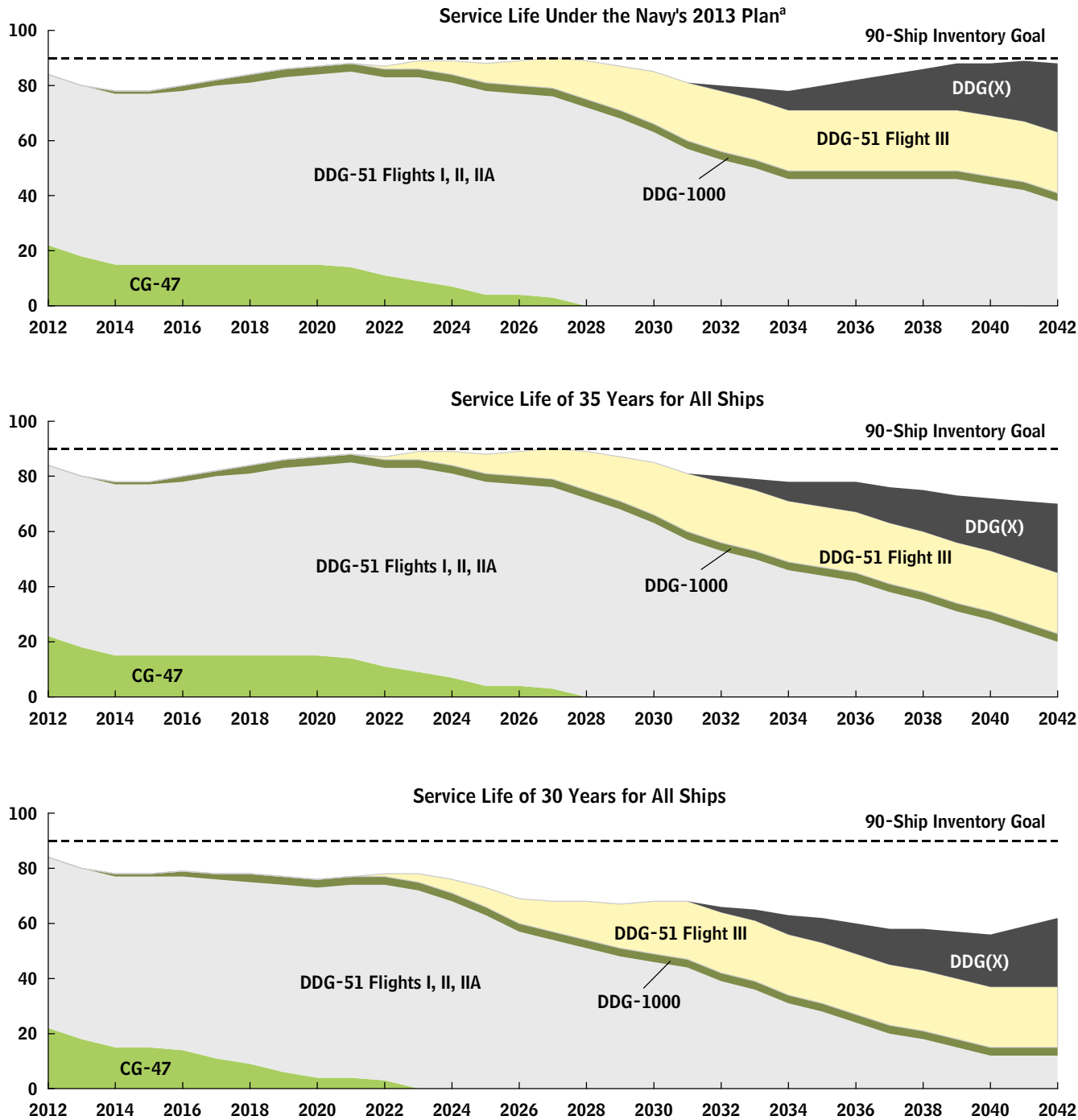
Figure 7. Return to Reference Inventory of Large Surface Combatants Under Various Scenarios for Service Life
