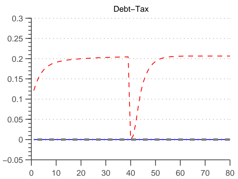
Figure 2: Non-linear Impulse Responses
