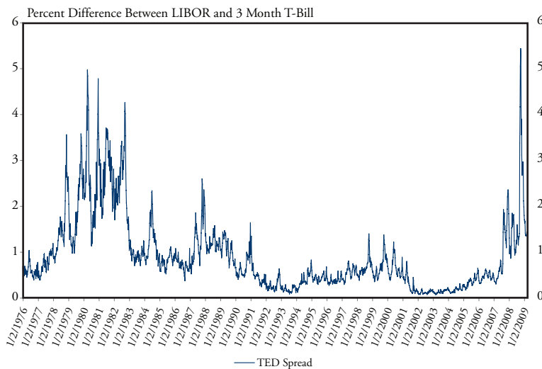
CHART 4 TED SPREAD FROM JANUARY 2, 1976 TO MAY 22, 2009
