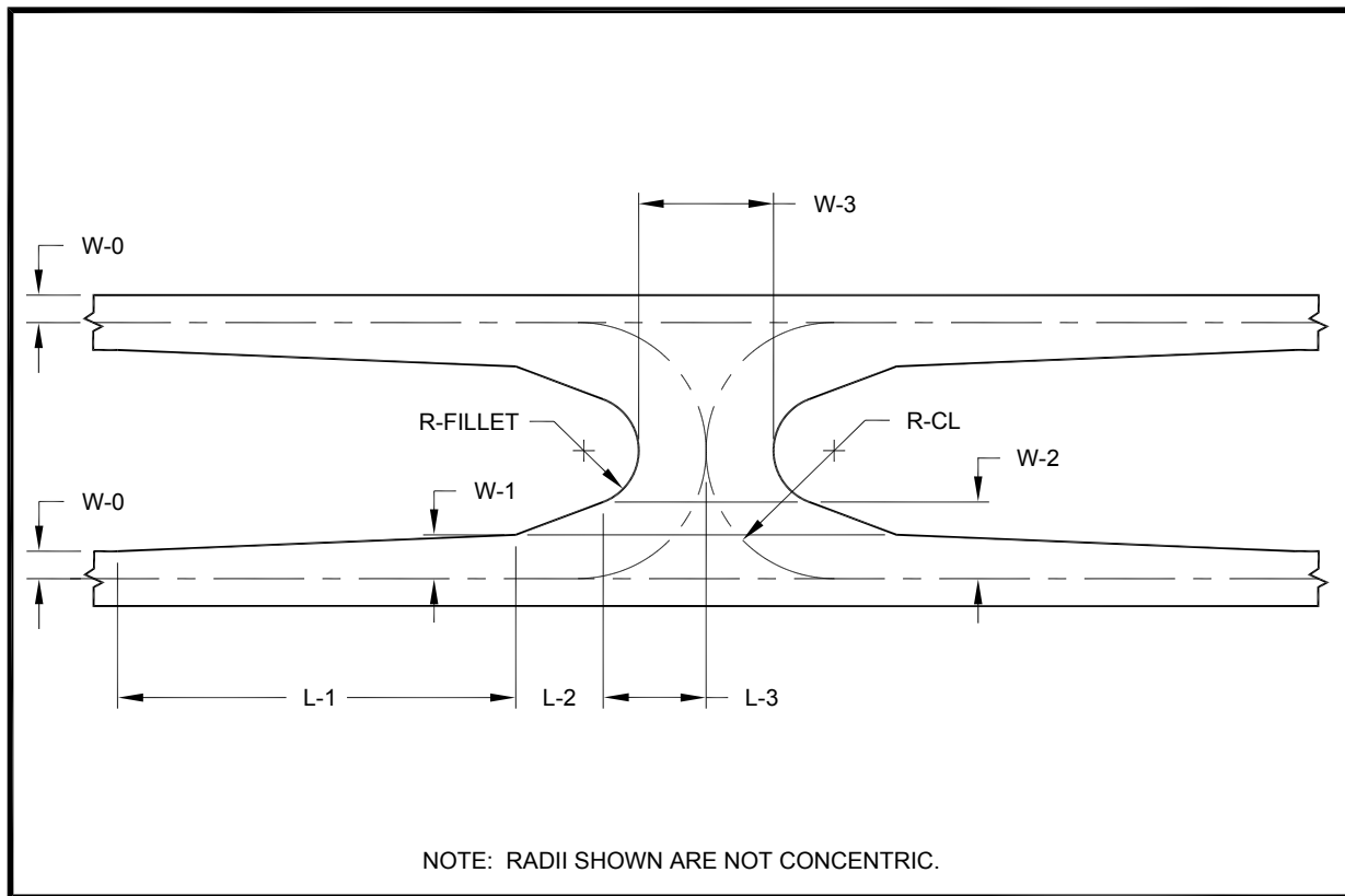
Figure 4-16. Crossover taxiway
