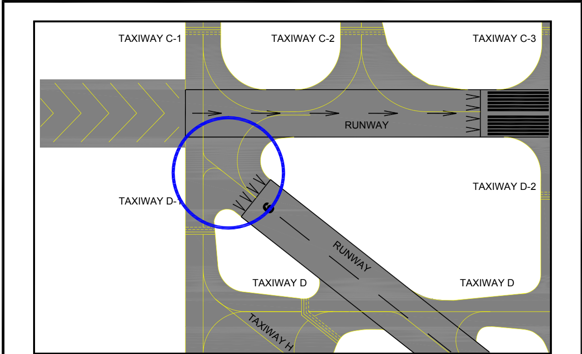
(e) Aligned taxiway between two closely spaced runway ends
