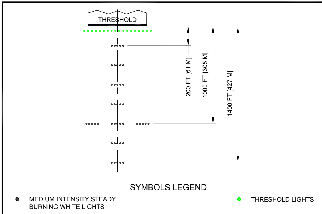
Figure 6-11. MALS
