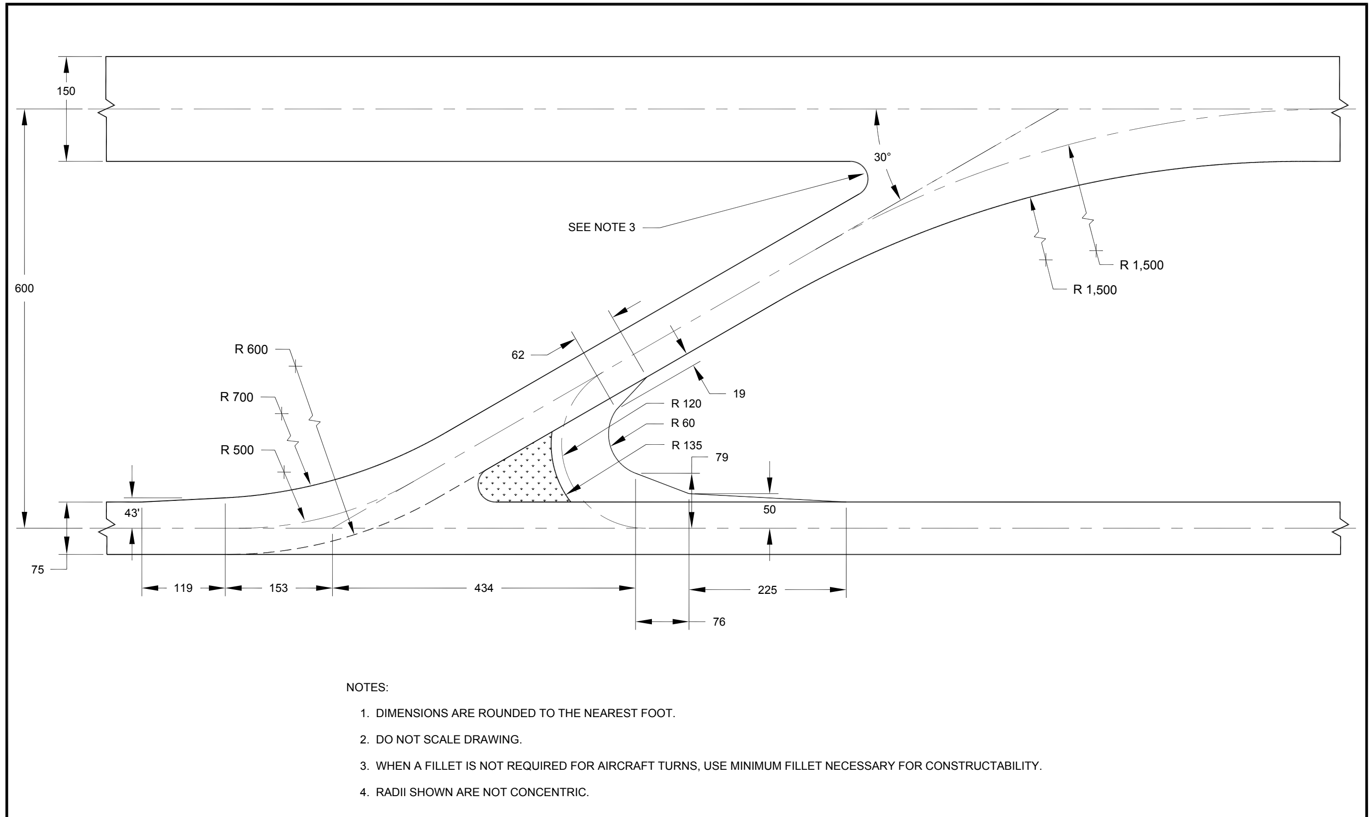
Figure 4-22. ADG-IV/V, TDG-5 high speed exit
