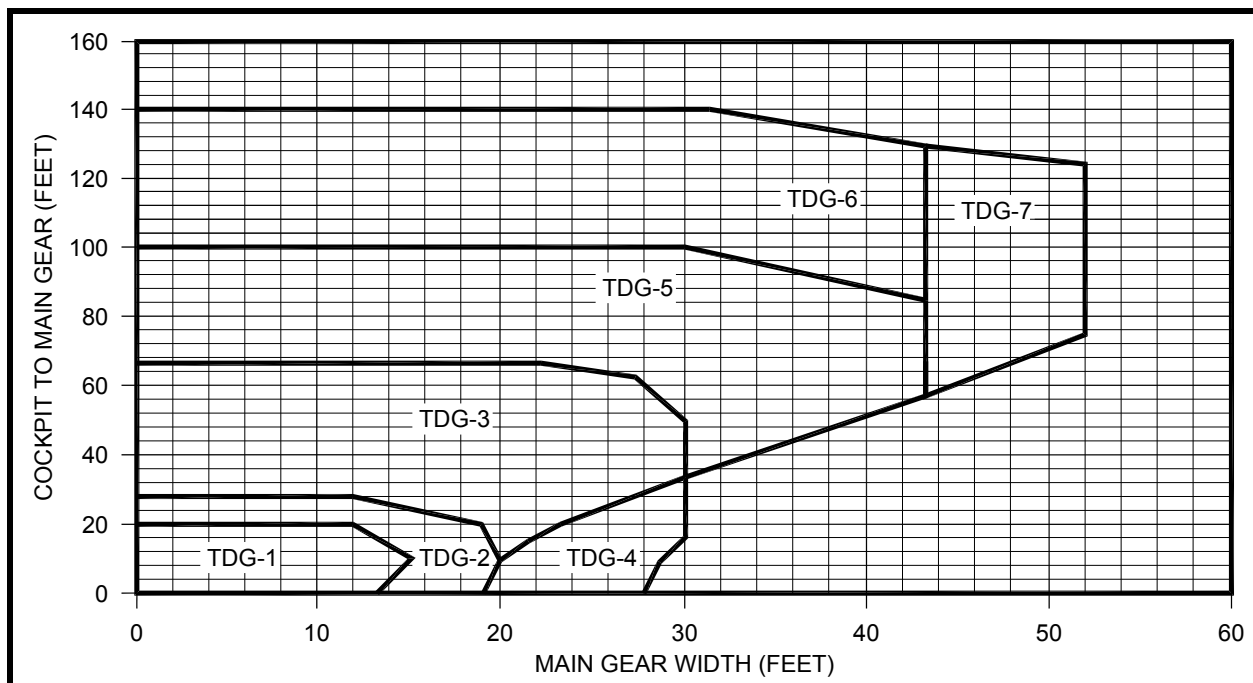
Figure 4-1. Taxiway Design Groups (TDGs)
