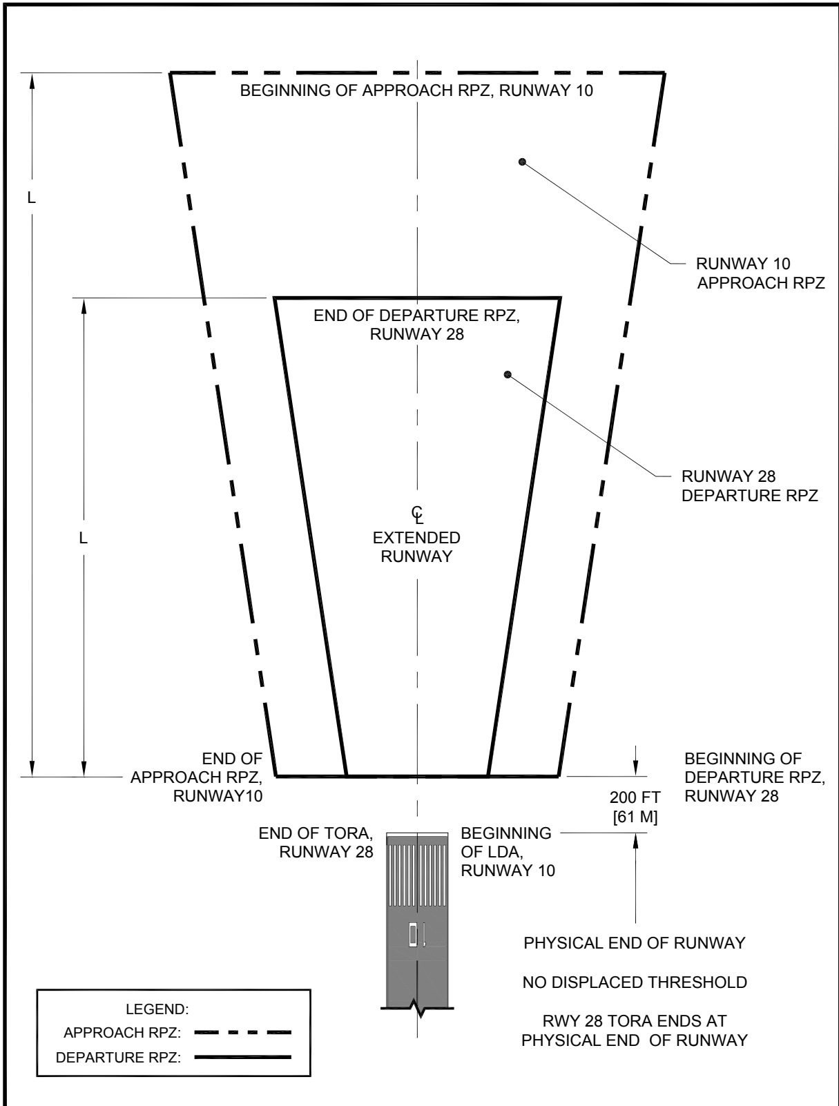
Figure 3-17. Runway with no published declared distances
