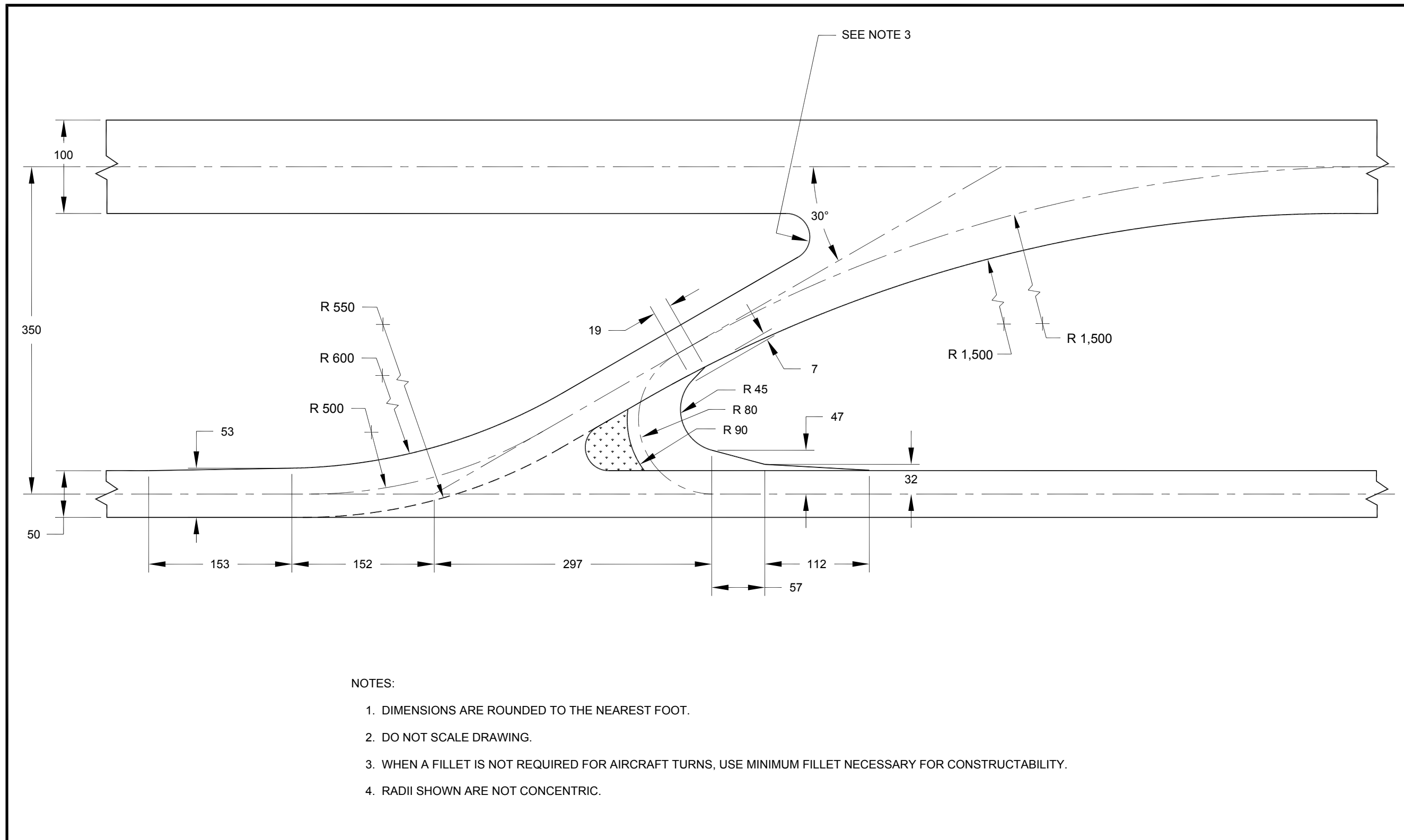
Figure 4-20. Airplane Design Group (ADG-III), TDG-3/4 high speed exit
