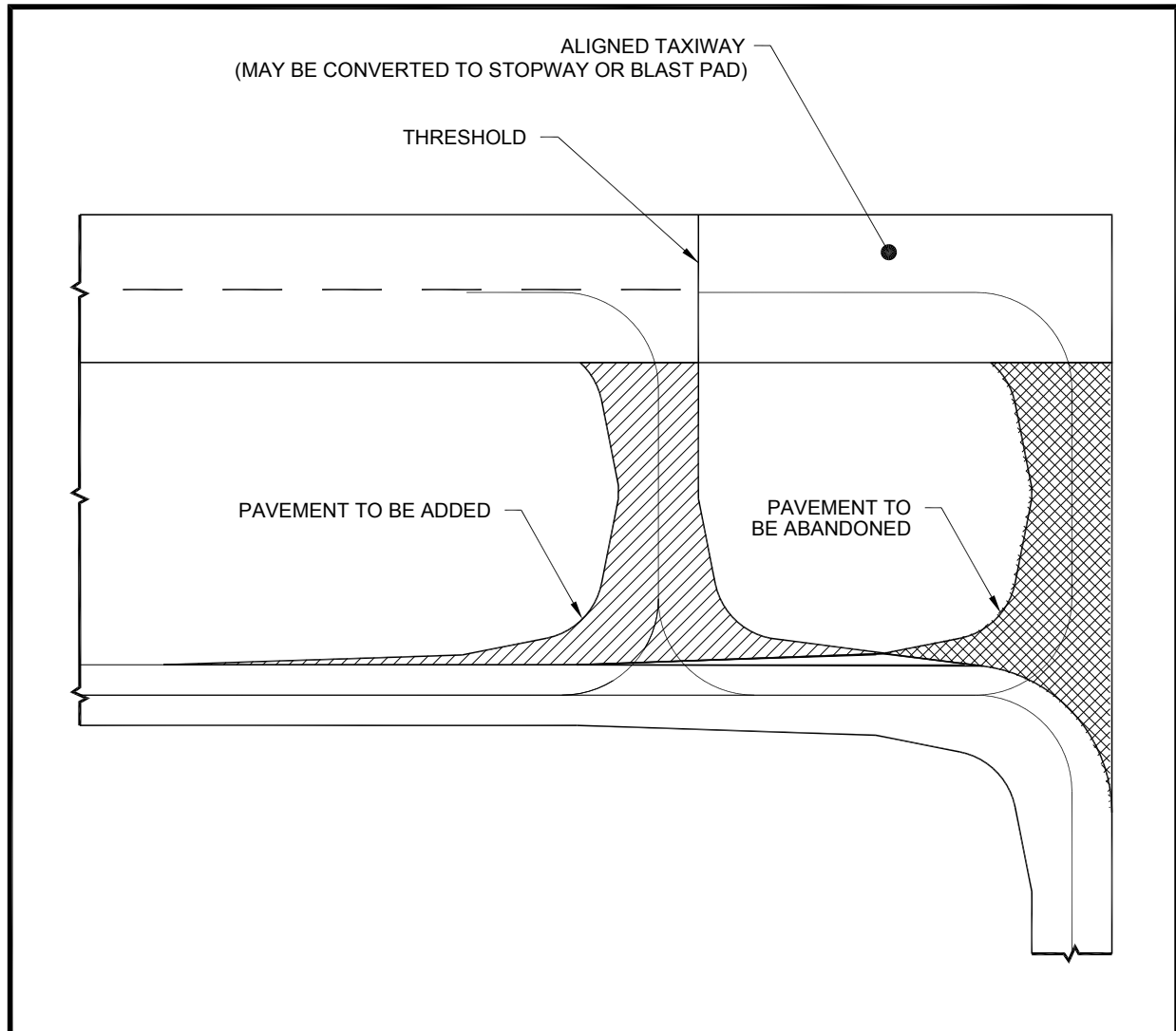
Figure 4-34. Aligned taxiway
