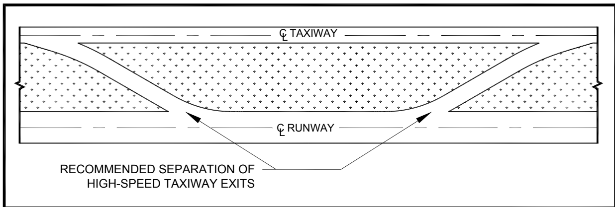
Figure 4-27. Proper design of high speed exits
