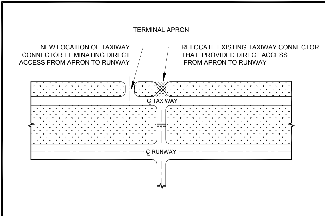
Figure 4-4. Proper taxiway design
