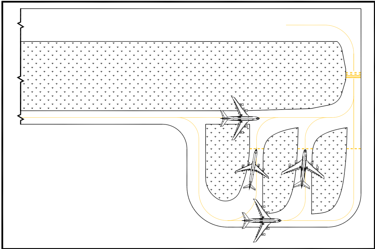
Figure 4-28. Typical holding bay configuration
