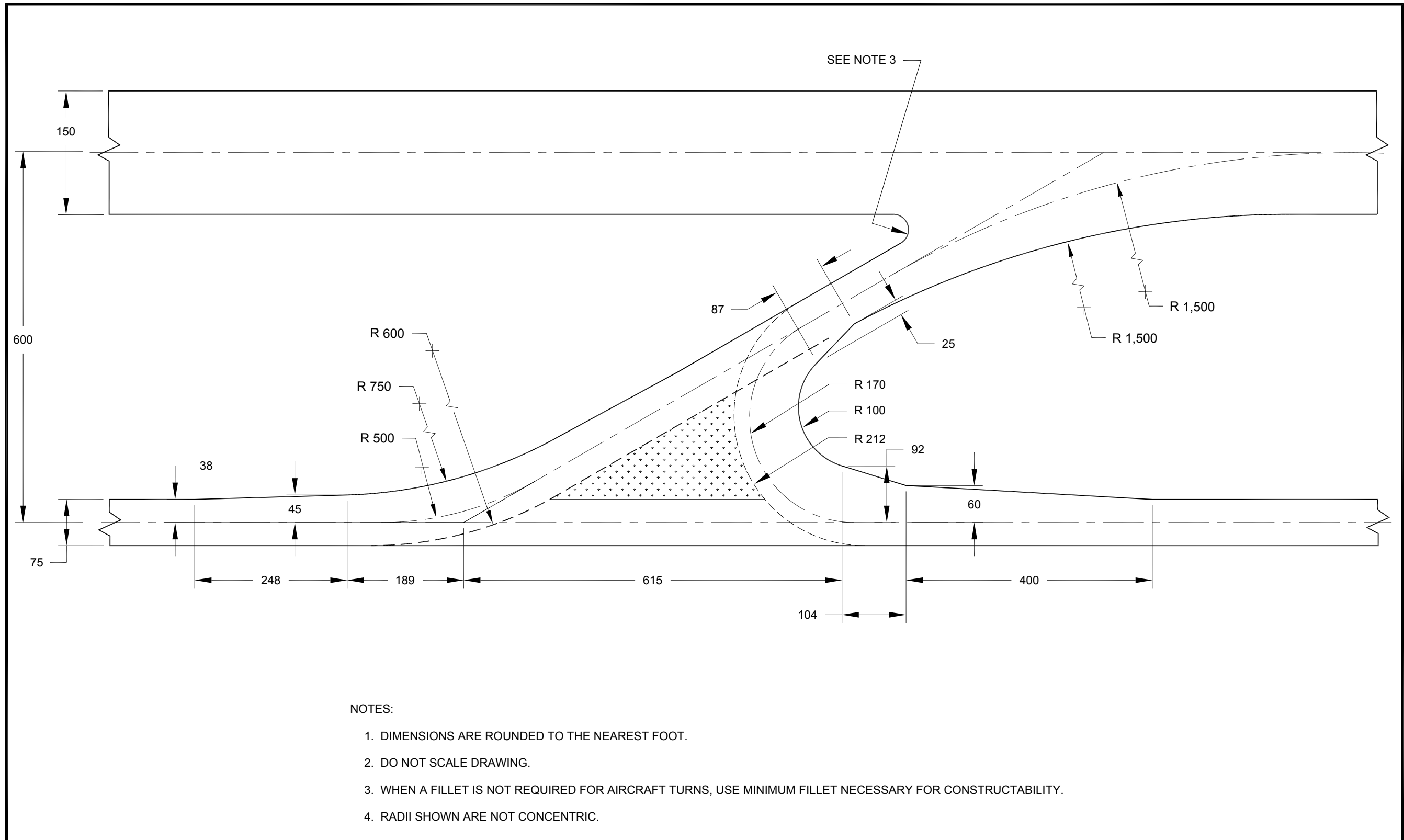
Figure 4-23. ADG-V, TDG-6 high speed exit
