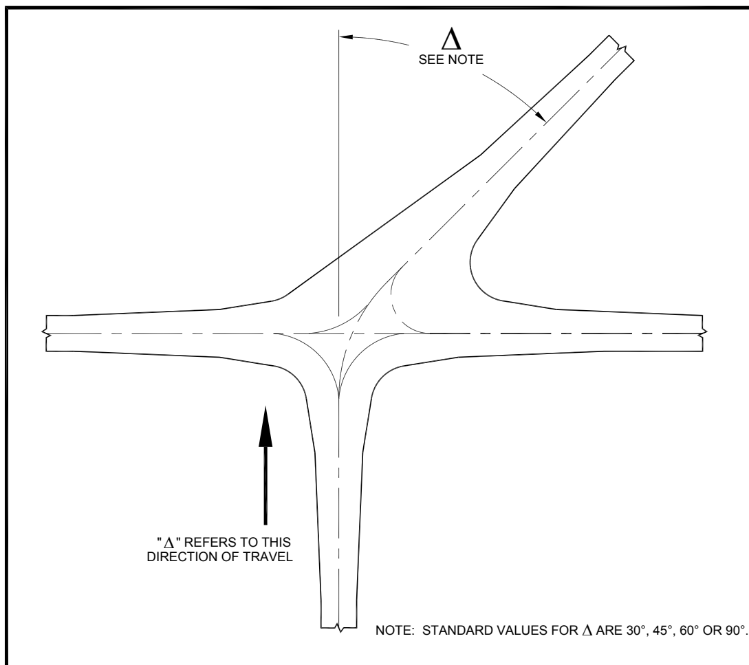
Figure 4-2. Three-node taxiway intersection
