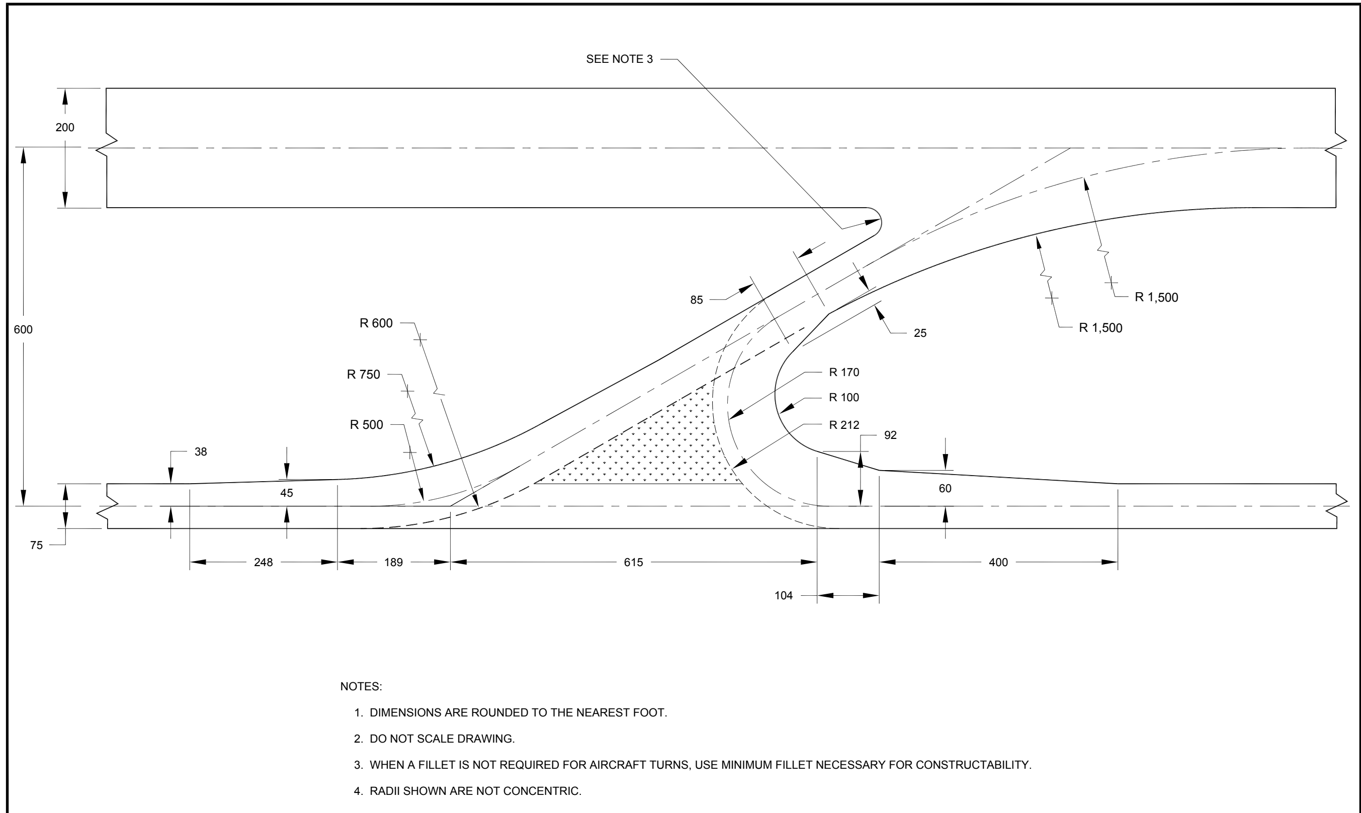
Figure 4-24. ADG-VI, TDG-6 high speed exit
