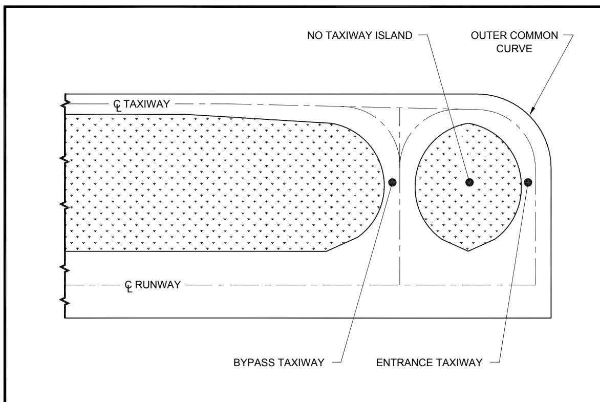
Figure 4-17. Bypass taxiway
