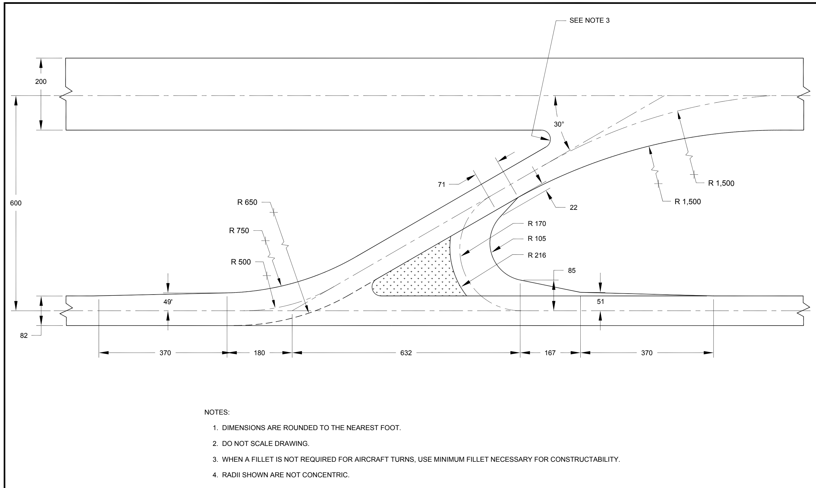
Figure 4-25. ADG-VI, TDG-7 high speed exit
