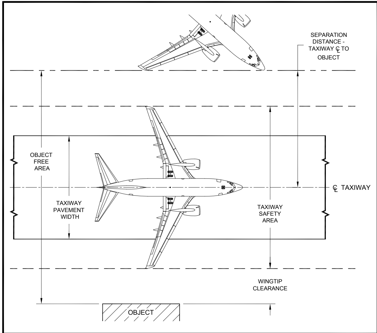
Figure 4-9. Wingtip clearance from taxiway
