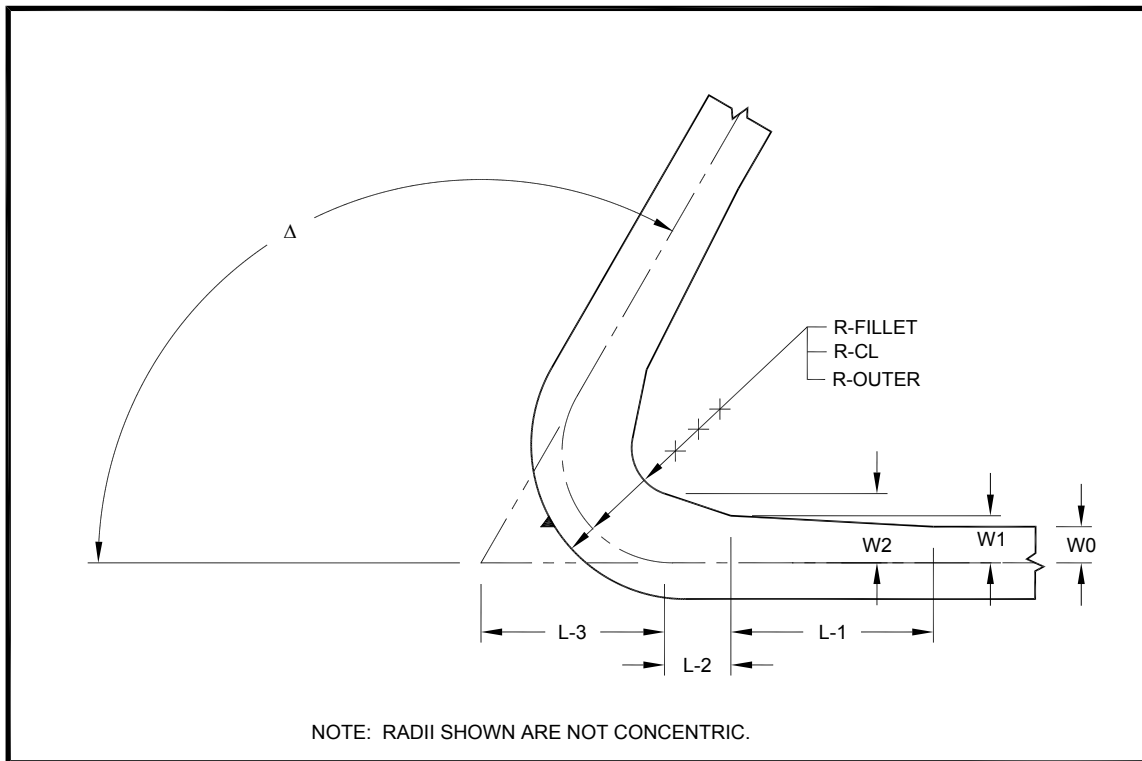
Figure 4-15. Greater than 90 degree delta
