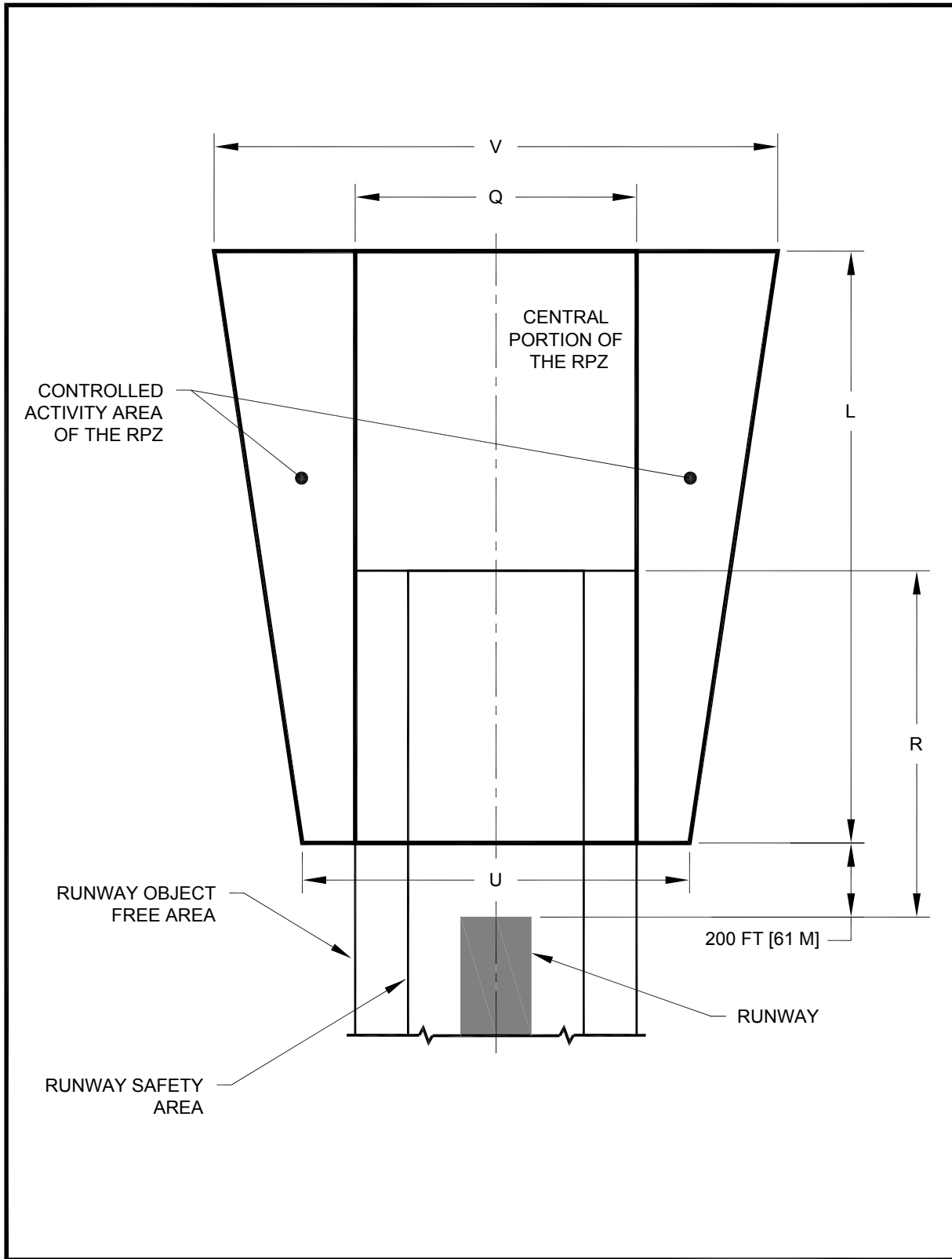
Figure 3-16. Runway Protection Zone (RPZ)
