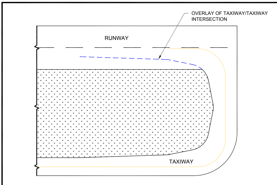
Figure 4-18. Entrance taxiway
