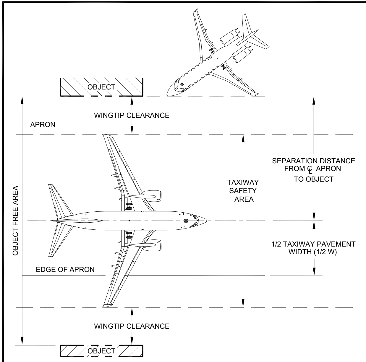
Figure 4-11. Wingtip clearance from apron taxiway
