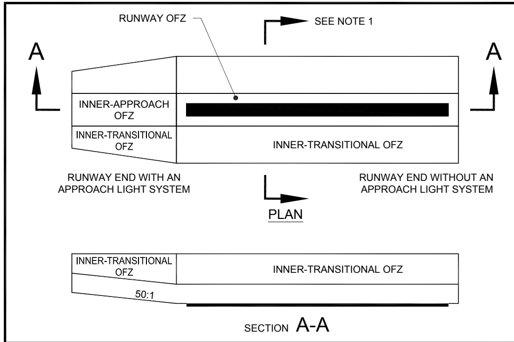
Figure 3-11. OFZ for operations on runways by large aircraft with lower than 3/4 statute mile (1.2 km) approach visibility minimums
