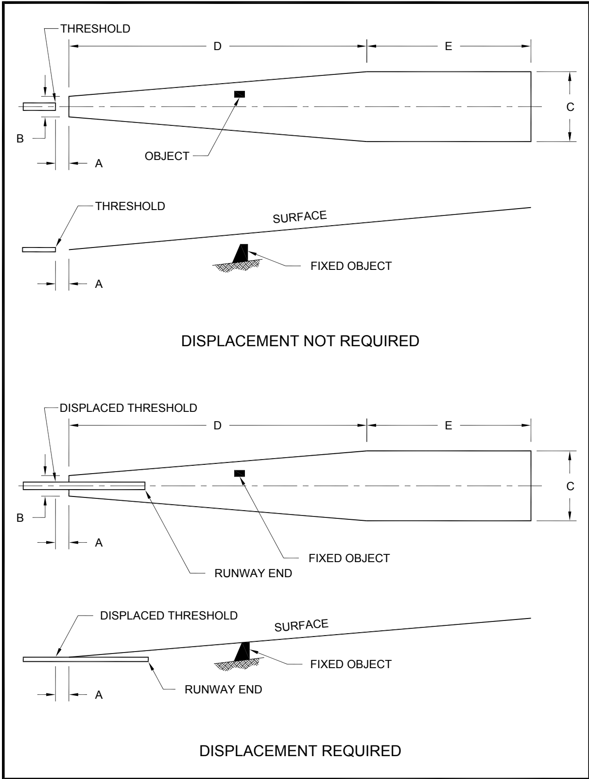
Figure 3-2. Threshold siting based on approach slope
