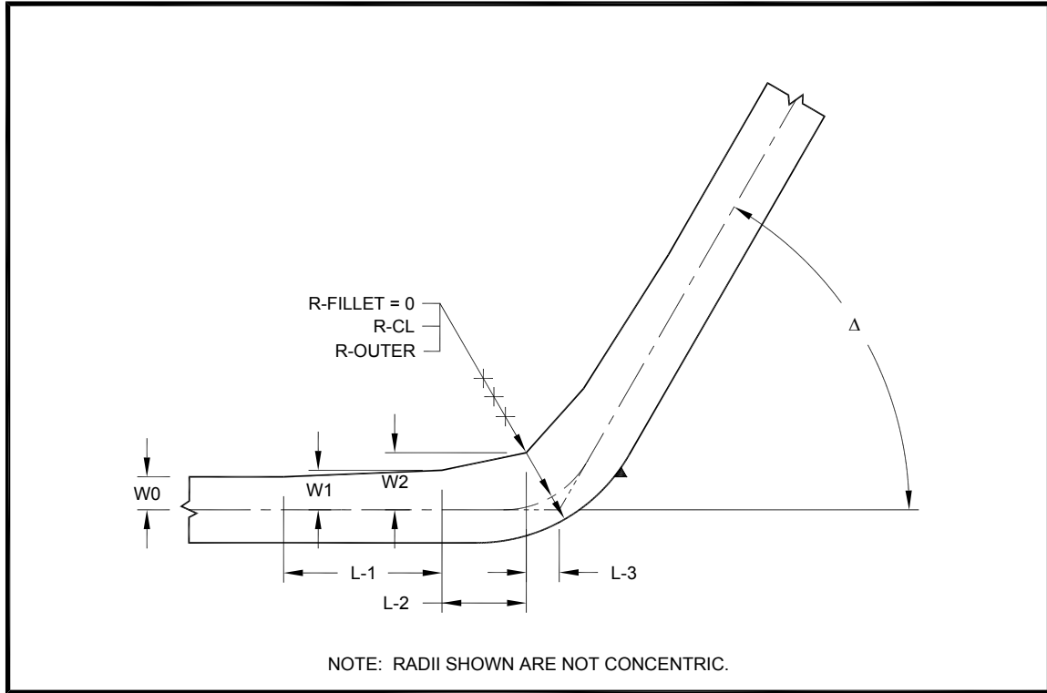
Figure 4-14. Less than 90 degree delta
