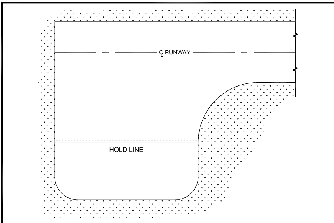
Figure 4-30. Poor holding bay design
