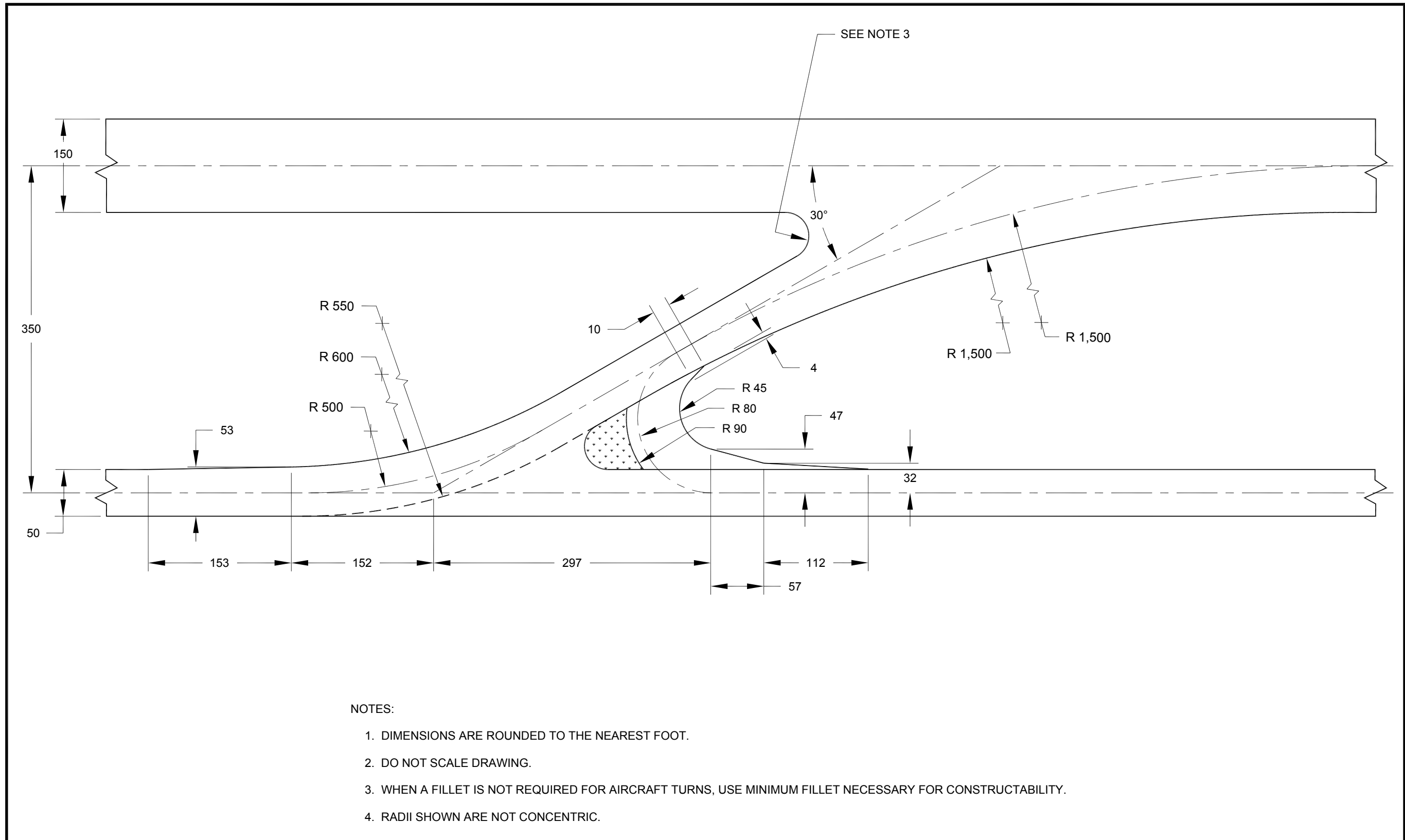
Figure 4-21. ADG-IV, TDG-3/4 high speed exit
