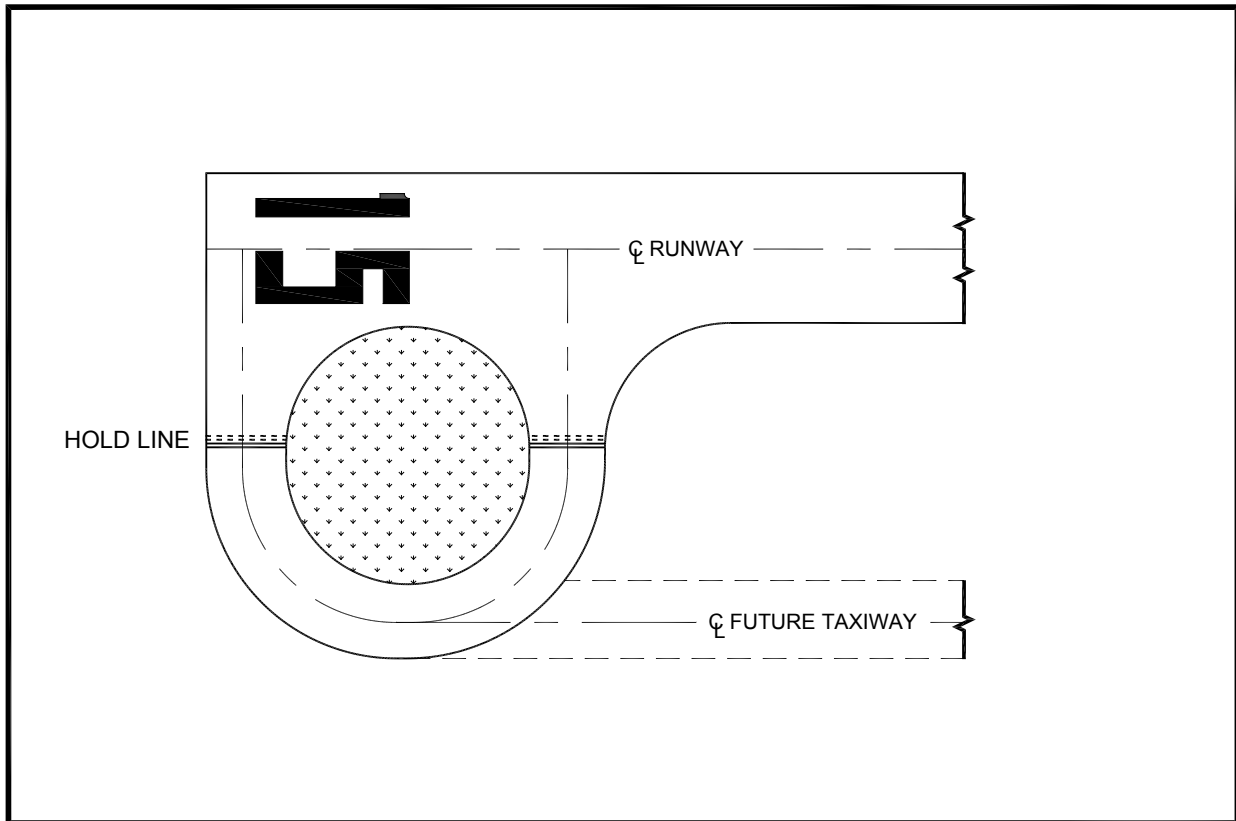
Figure 4-31. Taxiway turnaround
