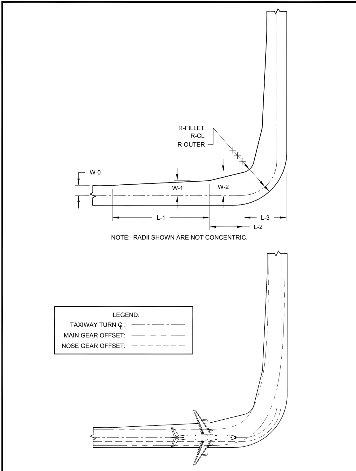
Figure 4-13. Taxiway turn
