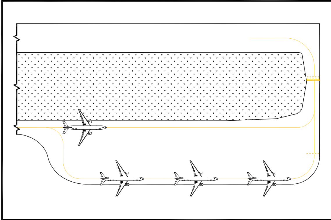
Figure 4-29. Holding bay – not recommended design
