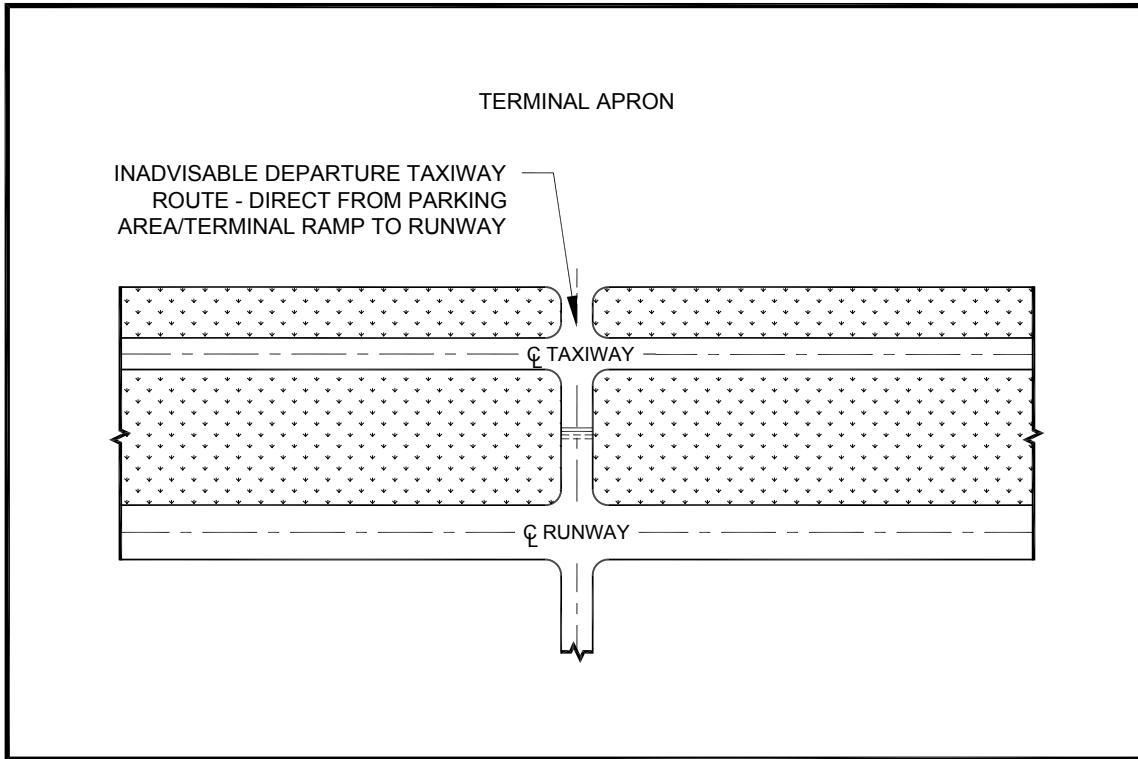
Figure 4-3. Not recommended taxiway design
