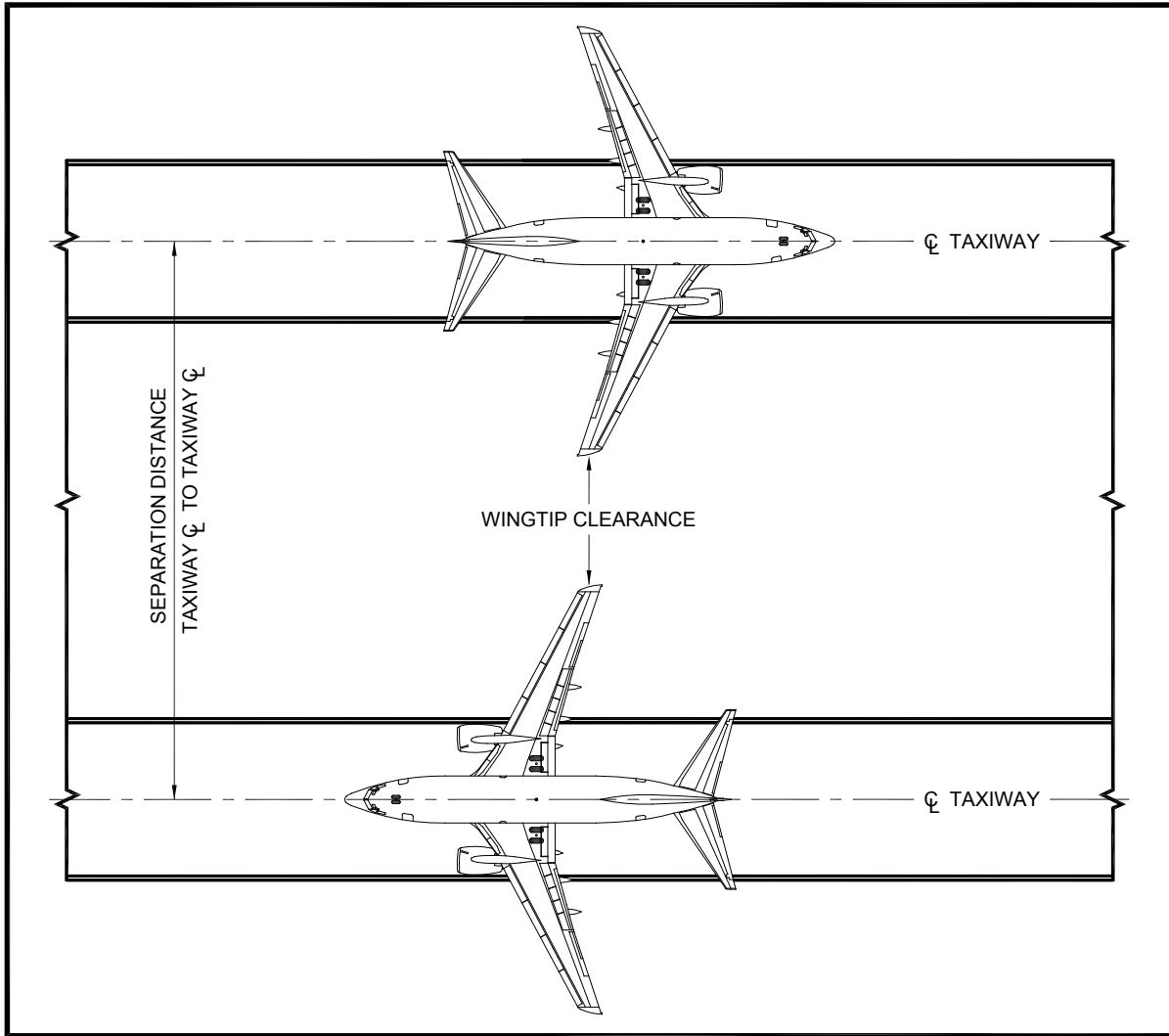
Figure 4-8. Wingtip clearance - parallel taxiways
