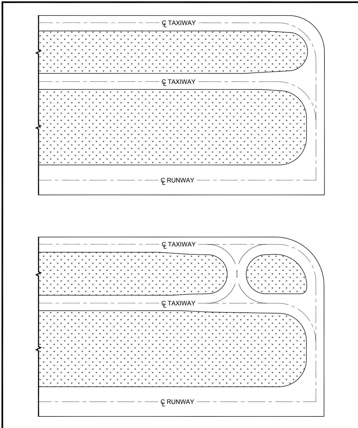
Figure 4-12. Parallel taxiways
