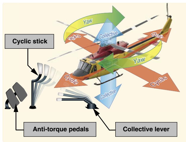
Figure 5-3. Helicopter flight control system.
