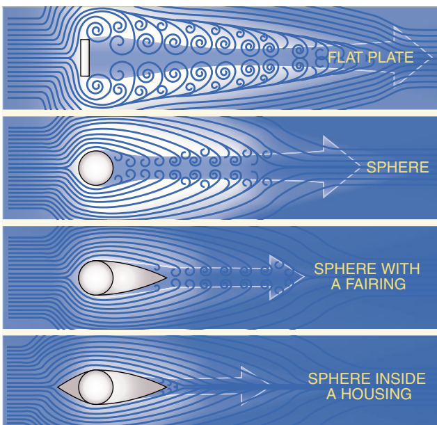
Figure 4-5. Form drag.
