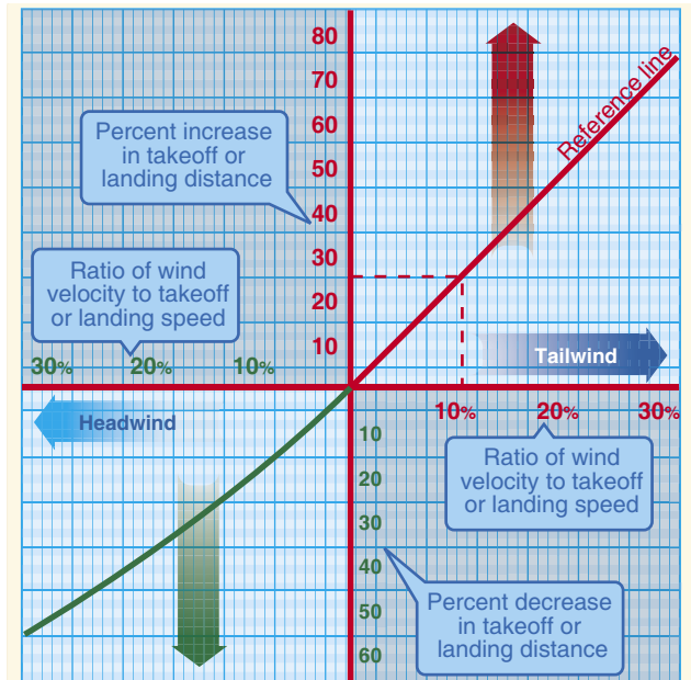
Figure 10-18. Effect of wind on takeoff and landing.
