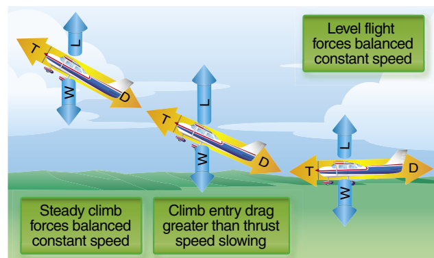
Figure 4-31. Changes in speed during climb entry.
