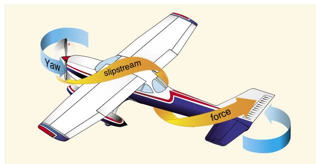
Figure 4-40. Corkscrewing slipstream.
