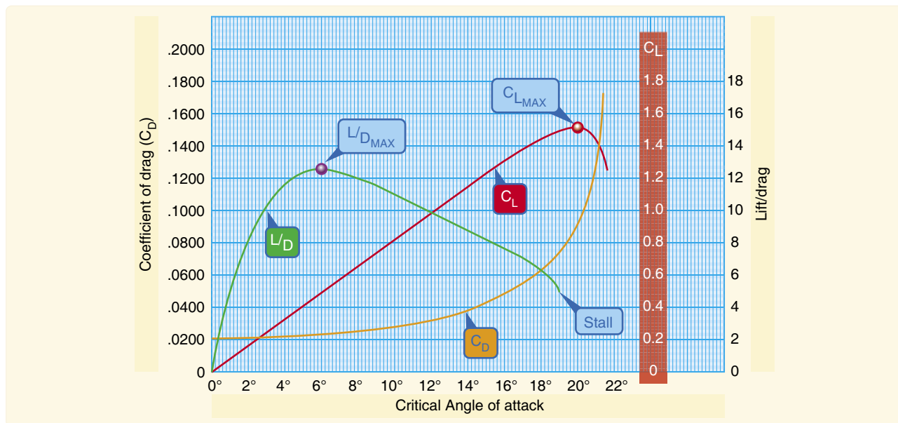
Figure 4-9. Lift coefficients at various angles of attack.
