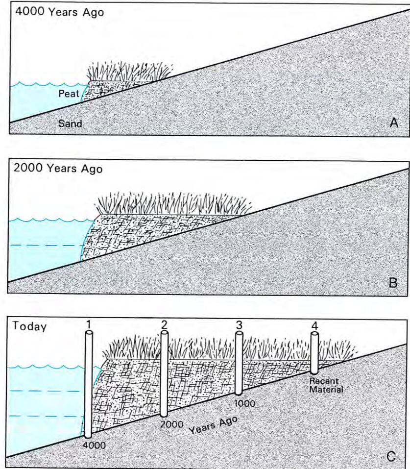
Figure 5. Growth and development of the Bay's wide marshy plains in response to slowly rising sea level. Core samples taken at the marsh peat base are used to age-date marsh development.
