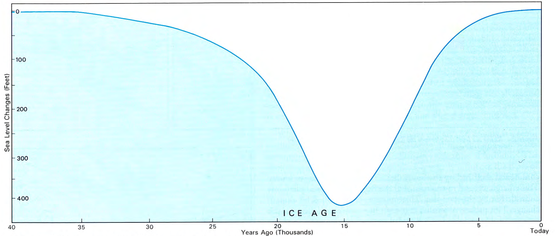
Figure 4. Sea-level rise curve for past 40,000 years, responding to advance and retreat of great ice sheets.
