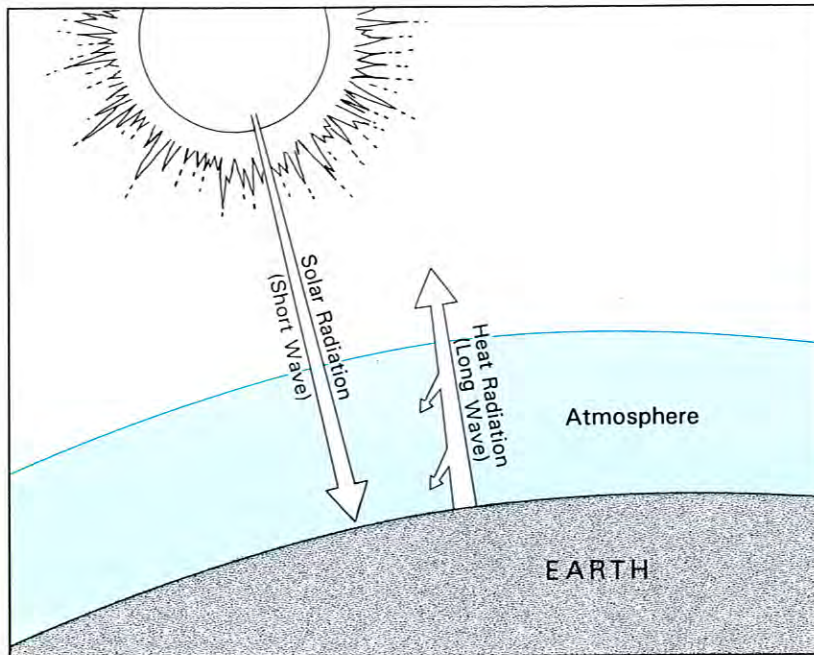
Figure 6. Schematic of the greenhouse effect. Small arrows indicate heat radiation directed back to Earth because of greenhouse gases.
