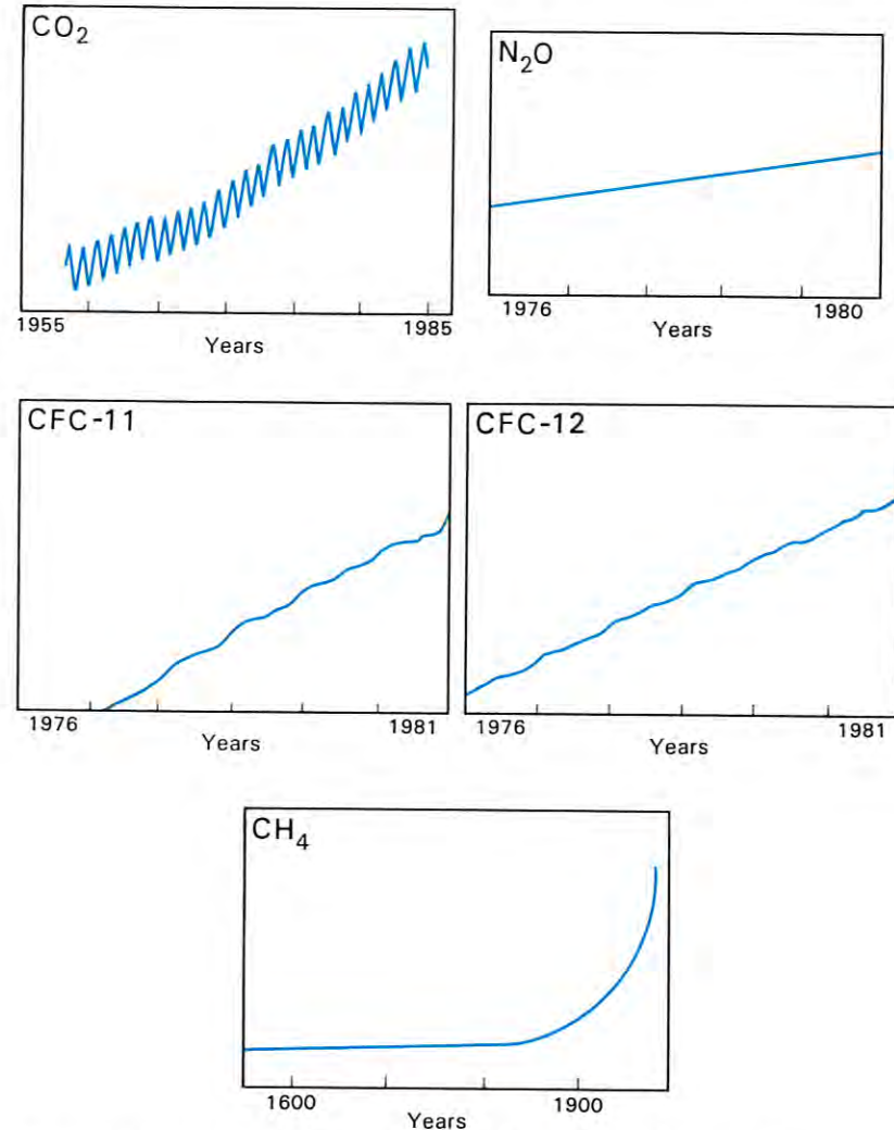
Figure 8. Increasing concentrations of greenhouse gases in the atmosphere (Intergovernmental Panel on Climate Change, 1990).
