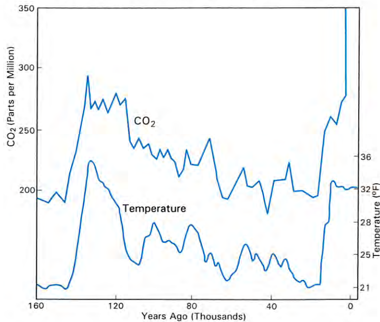
Figure 7. Correlation between temperature change and an increase of atmospheric \text{CO}_2 (Intergovernmental Panel on Climate Change, 1990).
