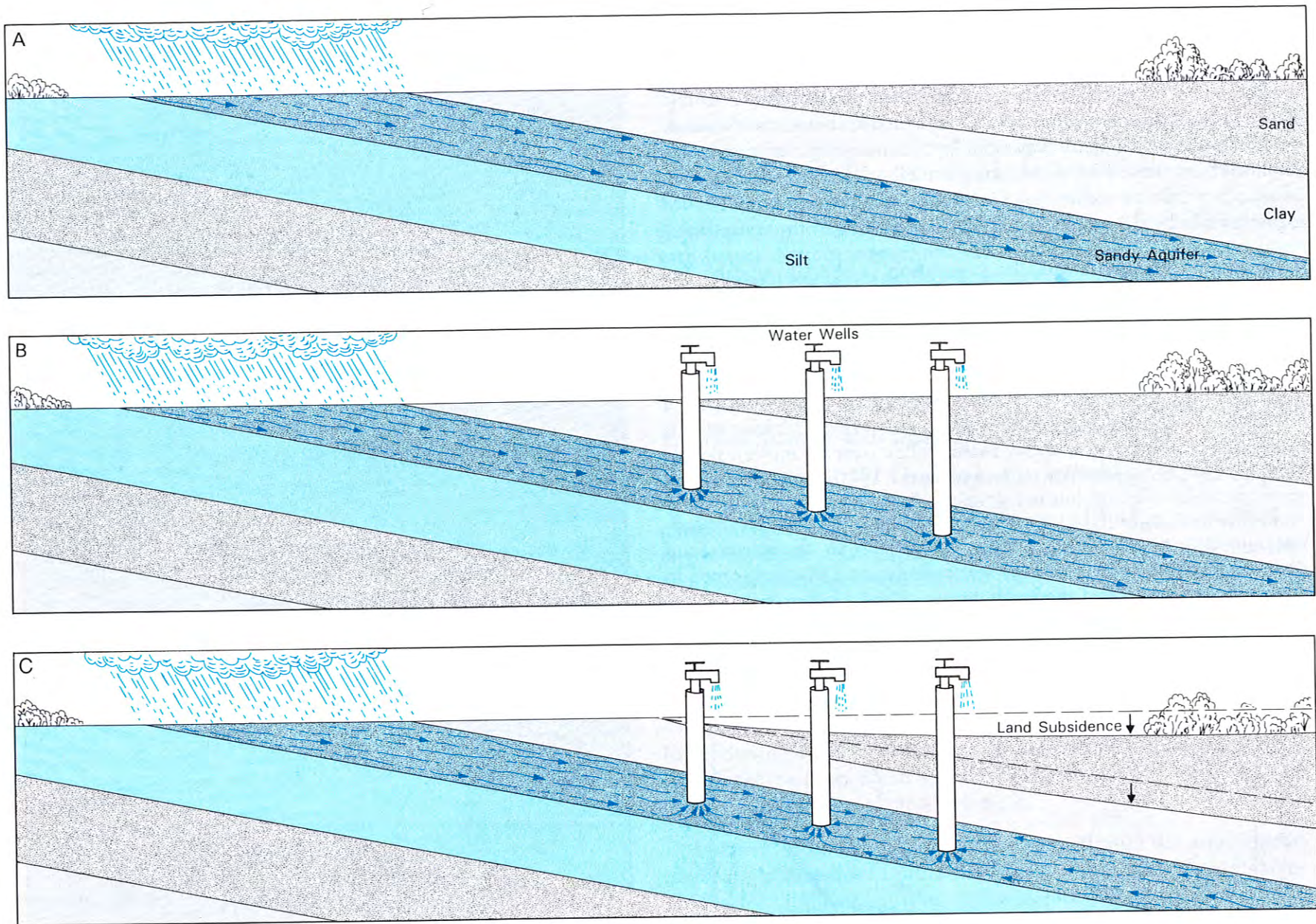
Figure 21. Groundwater withdrawal removes water from clay layers, resulting in layer compaction and land subsidence.
