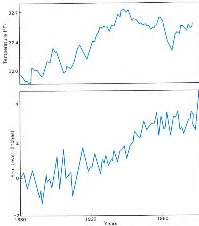
Figure 9. Correlation between global temperature and sea-level rise (Intergovernmental Panel on Climate Change, 1990).
