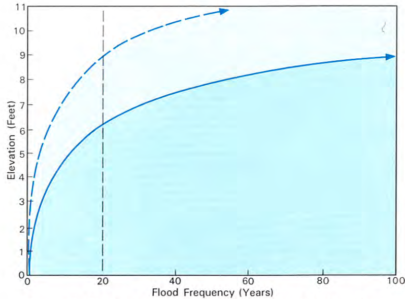
Figure 12. Flood frequency curve (solid curve from U.S. Army Corps of Engineers, Baltimore, Md.). A 3-foot rise in sea level (dashed curve) turns a 20-year storm into a 100-year flood.
