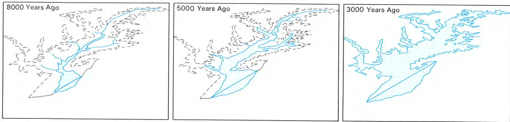
Figure 2. Rising sea level transformed the Susquehanna and other rivers into the Chesapeake Bay.
