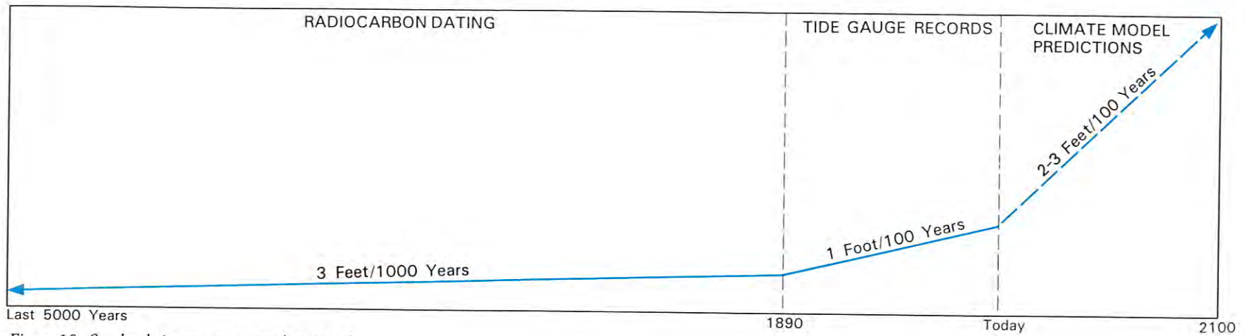
Figure 10. Sea-level rise curve: past and projected.
