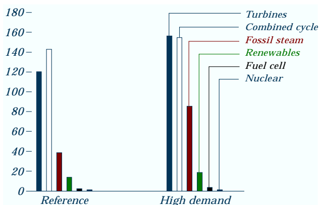
Figure 67. Cumulative new generating capacity by type in two cases, 1995-2015 (gigawatts)
