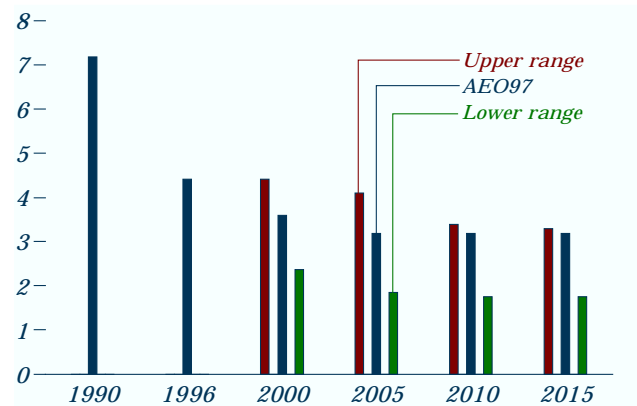
Figure 72. Levelized costs of electricity from wind power, 1990-2015 (1995 cents per kilowatthour)
