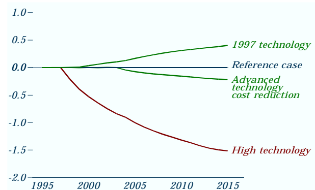
Figure 54. Variation from reference case primary commercial energy use in three alternative cases, 1995-2015 (quadrillion Btu)
