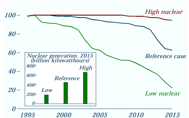
Figure 66. Operable nuclear capacity in three cases, 1995-2015 (gigawatts)
