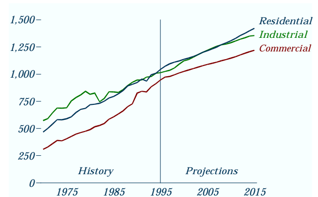
Figure 58. Annual electricity sales by sector, 1970-2015 (billion kilowatthours)
