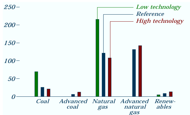
Figure 69. Cumulative new electricity generating capacity by technology type in three cases, 1995-2015 (gigawatts)
