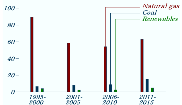
Figure 60. Electricity generation and cogeneration capacity additions by fuel type, 1995-2015 (gigawatts)
