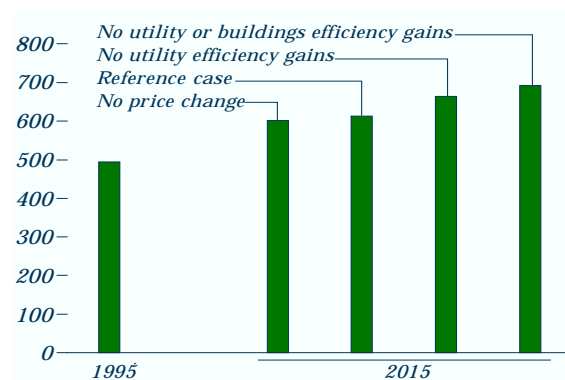
Figure 18. Buildings sector carbon emissions in alternative price and efficiency cases (million metric tons of carbon)
