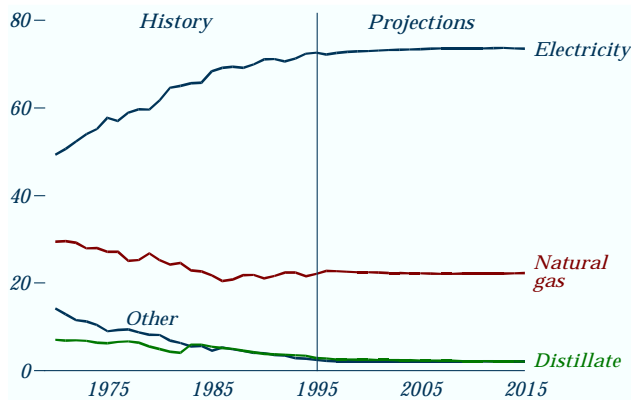
Figure 40. Commercial nonrenewable total energy consumption by fuel, 1970-2015 (percent of total)
