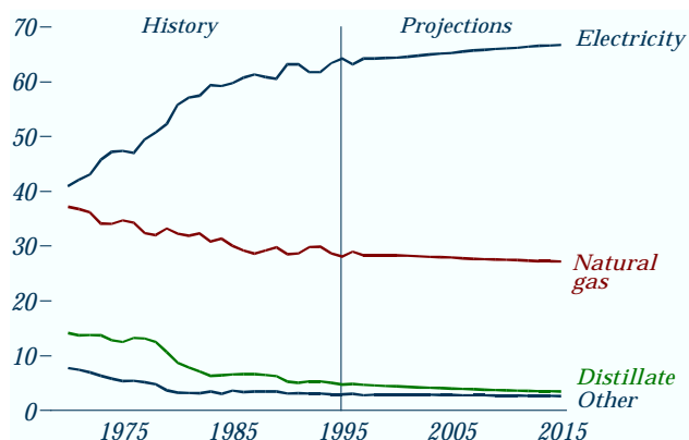
Figure 38. Residential total energy consumption by fuel, 1970-2015 (percent of total)
