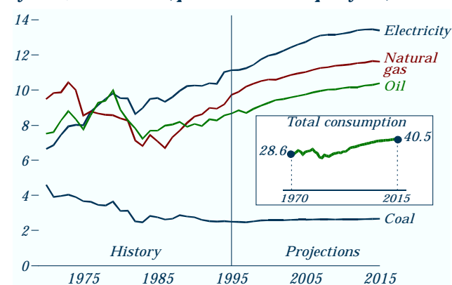
Figure 43. Industrial total energy consumption by fuel, 1970-2015 (quadrillion Btu per year)
