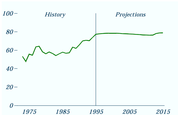
Figure 65. Nuclear power plant capacity factors, 1973-2015 (percent)
