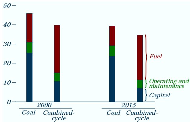
Figure 63. Electricity generation costs, 2000 and 2015 (1995 mills per kilowatthour)
