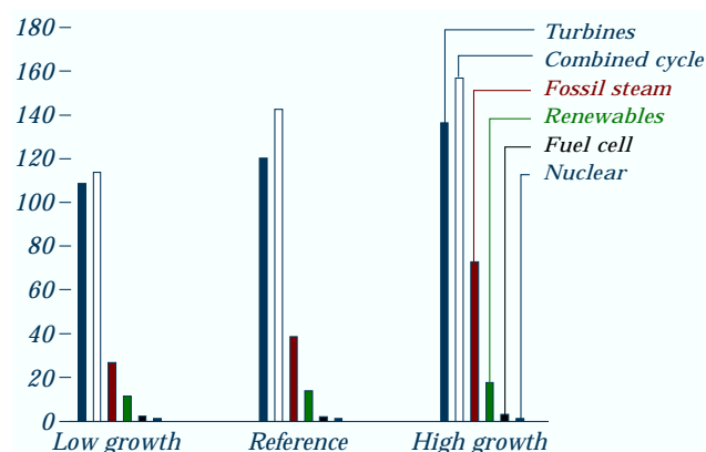
Figure 68. Cumulative new generating capacity by type in three cases, 1995-2015 (gigawatts)
