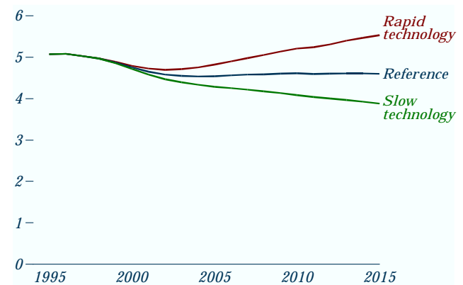
Figure 91. Lower 48 oil production in alternative technology cases, 1995-2015 (million barrels per day)
