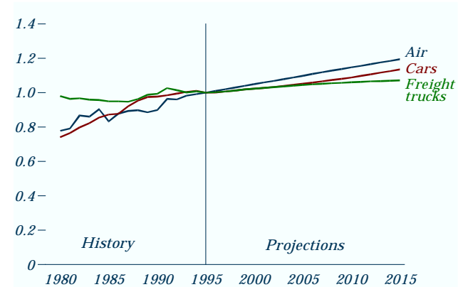
Figure 47. Transportation stock fuel efficiency by mode, 1980-2015 (index, 1995 = 1)
