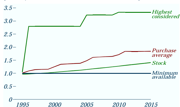
Figure 42. Efficiencies of commercial electric water heaters in the reference case, 1995-2015 (index, minimum available in 1995 = 1)
